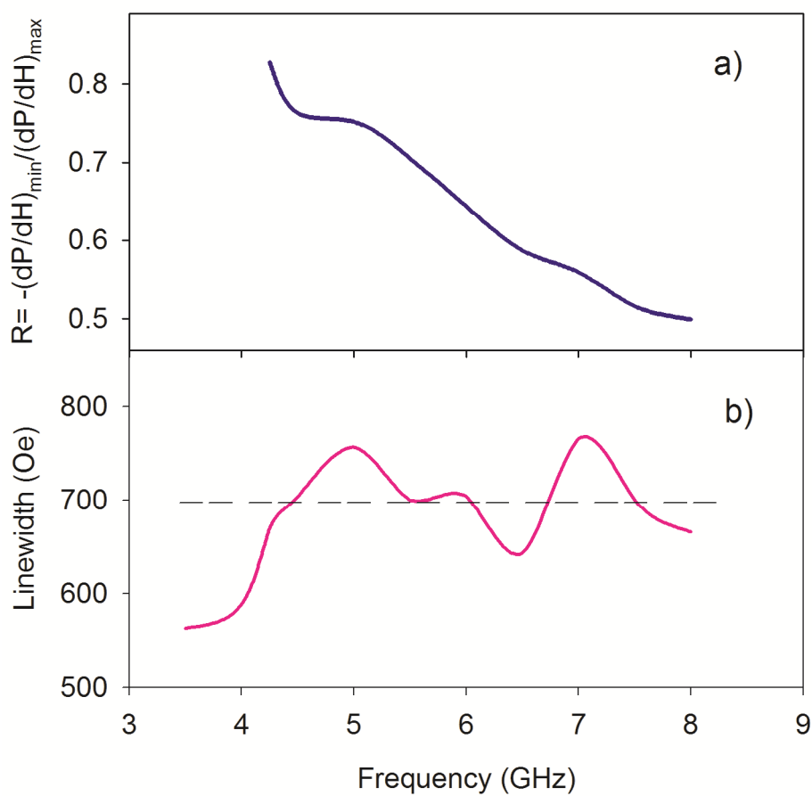
Figure 8. a) Broadening factor R = -(\text{dP/dH})_{\text{min}} / (\text{dP/dH})_{\text{max}} variation with frequency in sample annealed at 400° C. b) Linewidth of ferromagnetic resonance vs frequency.
