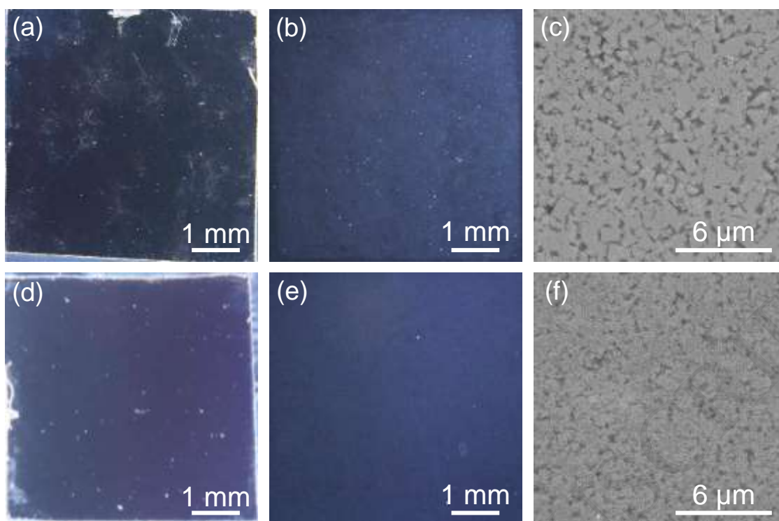
Figure 11 – Optical and SEM images of WC-NiCrCoMo (a-c) and WC-NiCrMo (d-f) after 2 weeks of immersion in 0.5 M NaCl: a) and d) surface of the samples just after testing; b) and e) same surfaces after flushing the surface with distilled water; c) and f) microscopic detail of the tested areas, showing no signs of corrosion.
