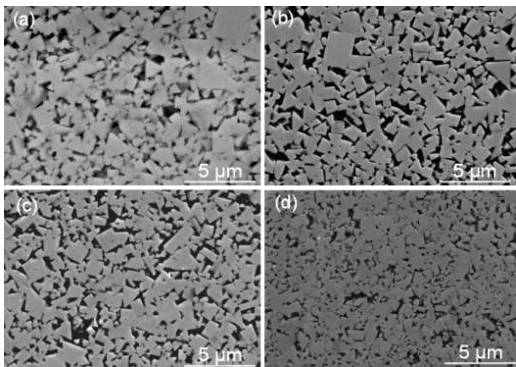
Figure 1 – SEM images of polished surfaces etched with Murakami's solution: (a) WC-Co; (b) WC-FeCoNi; (c) WC-NiCrCoMo and (d) WC-NiCrMo.
