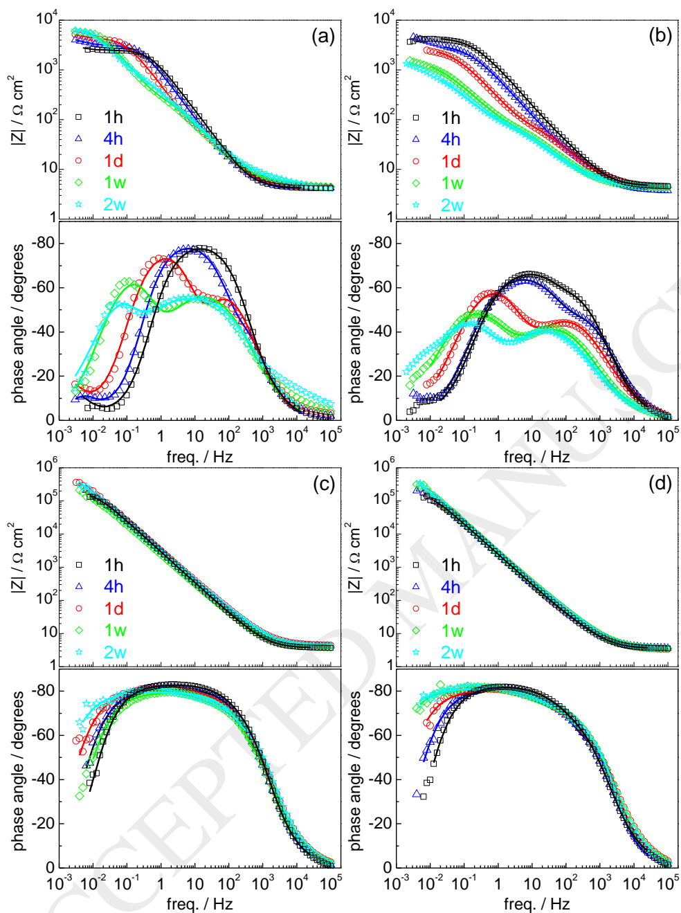
Figure 6 – Bode plots of the impedance measured in 0.5 M NaCl during 2 weeks for: (a) WC-Co, (b) WC-FeCoNi, (c) WC-NiCrCoMo and (d) WC-NiCrMo in 0.5 M NaCl. Symbols are experimental points and lines are the result of numerical fitting.
