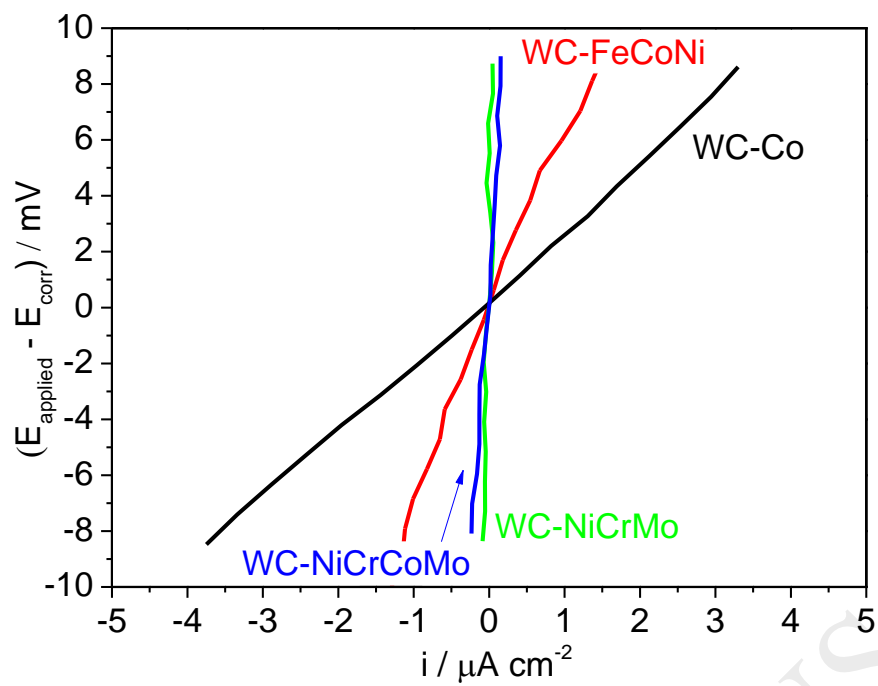
Figure 5 – Polarisation resistance measured in 0.5 M NaCl after 1 h in 0.5 M NaCl.
