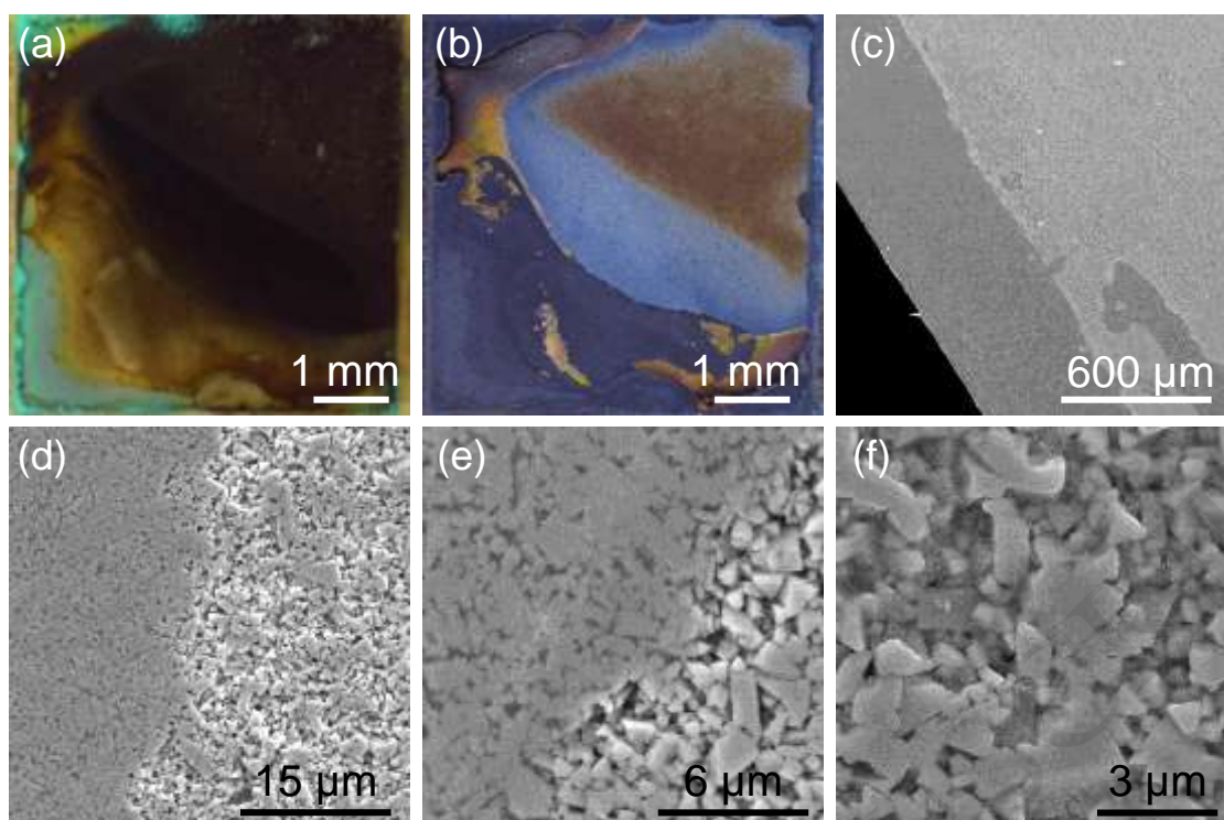
Figure 9 – Optical and SEM images of WC-Co after 2 weeks of immersion in 0.5 M NaCl:
