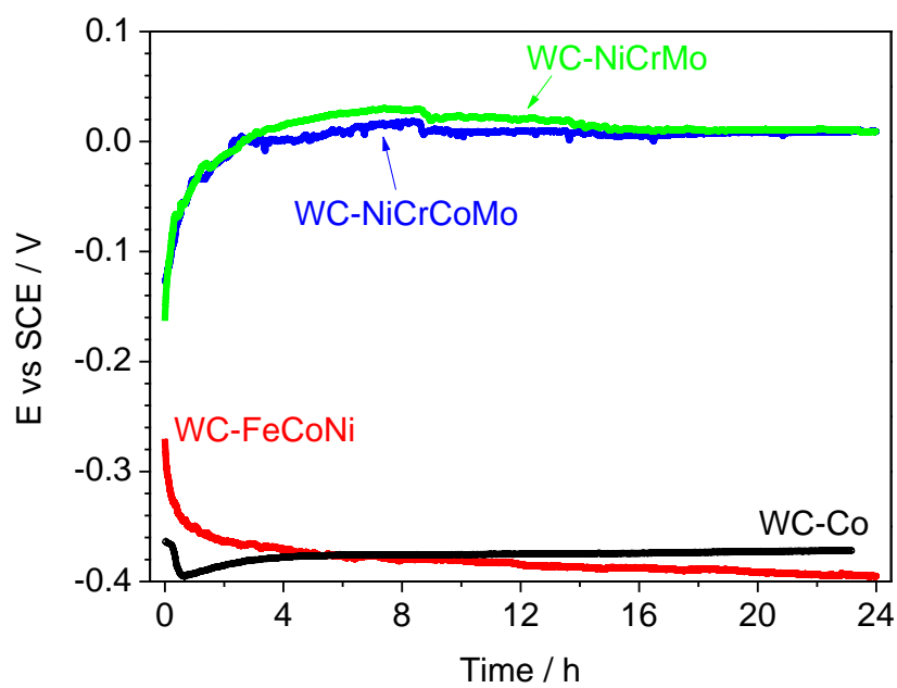
Figure 3 – Corrosion potential of the composites in the first 24 h of immersion in 0.5 M NaCl.
