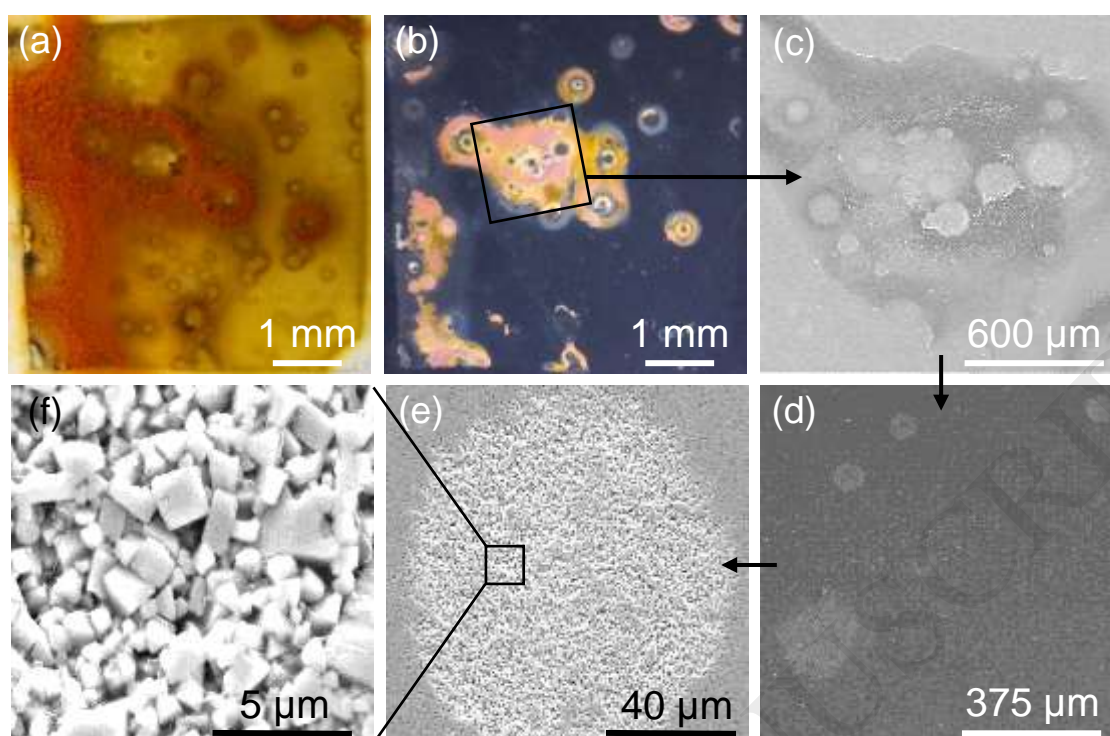
Figure 10 – Optical and SEM images of WC-FeCoNi after 2 weeks of immersion in 0.5 M NaCl: a) surface after testing; b) same area after removal of the loose corrosion products (flushing the surface with distilled water); c) magnification of a corroded region in b); d) a small area of c) after small abrasion of the surface; e) magnification of a corroded spot of d); f) inside the corroded spot (lack of binder surrounding the WC particles).
