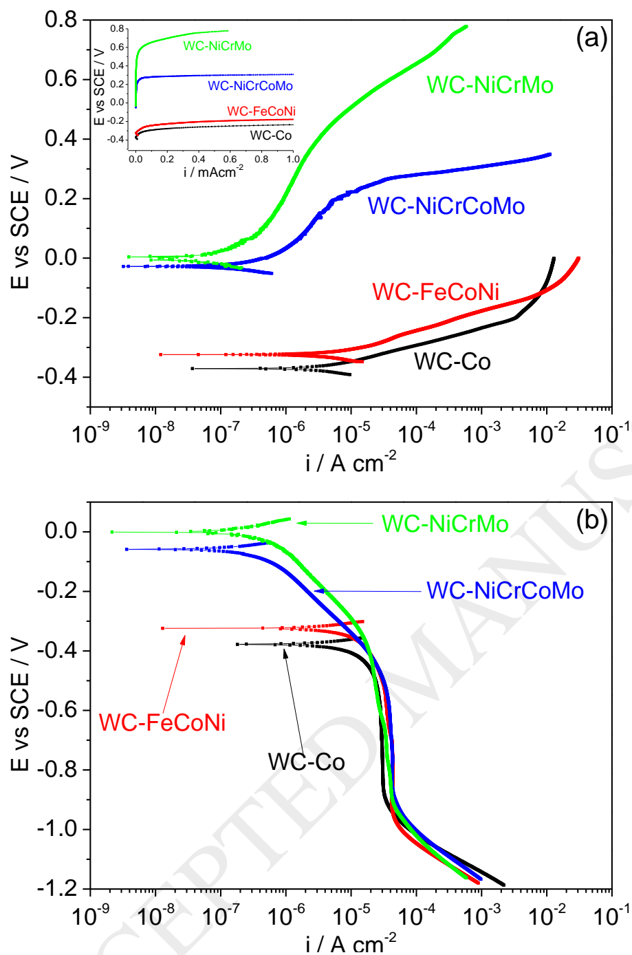
Figure 4 – Polarisation curves of the four composites after 1 h of immersion in 0.5 M NaCl:
