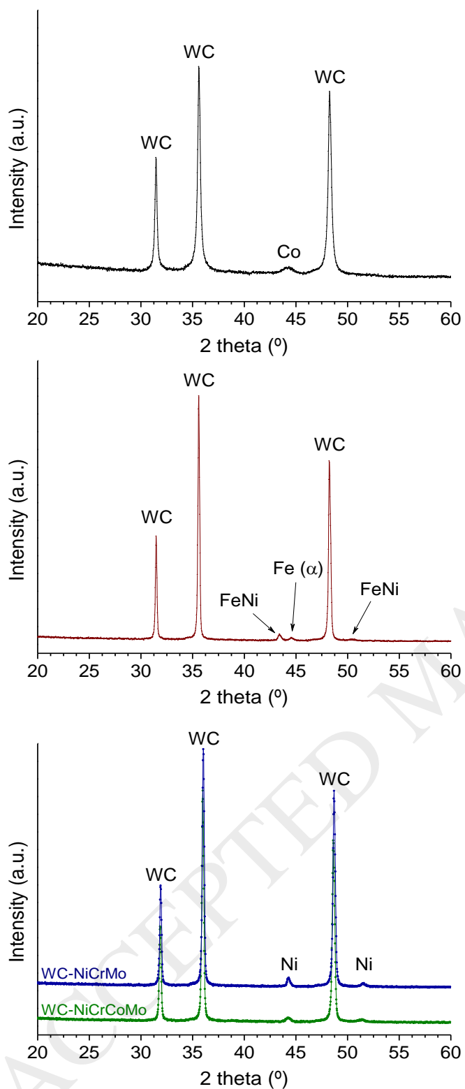
Figure 2 – XRD patterns of (a) WC-Co, (b) WC-FeCoNi, (c) WC-NiCrCoMo and WC-NiCrMo.
