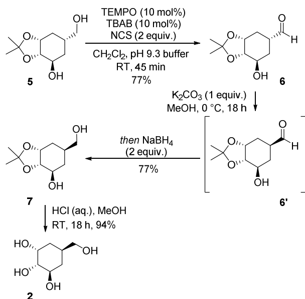
Scheme 3. Synthesis of carbasugar 2 from protected carbasugar 5 .
