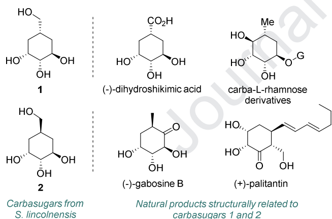
Figure 1. Selected natural products structurally related to carbasugars 1 and 2 .
