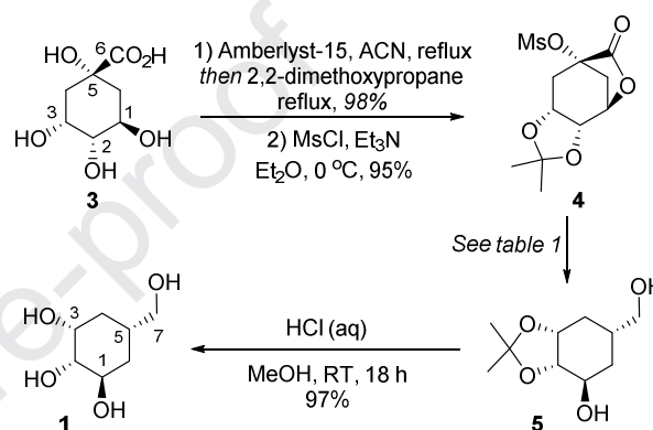
Scheme 1. Synthesis of carbasugar 1 from (-)-quinic acid.
