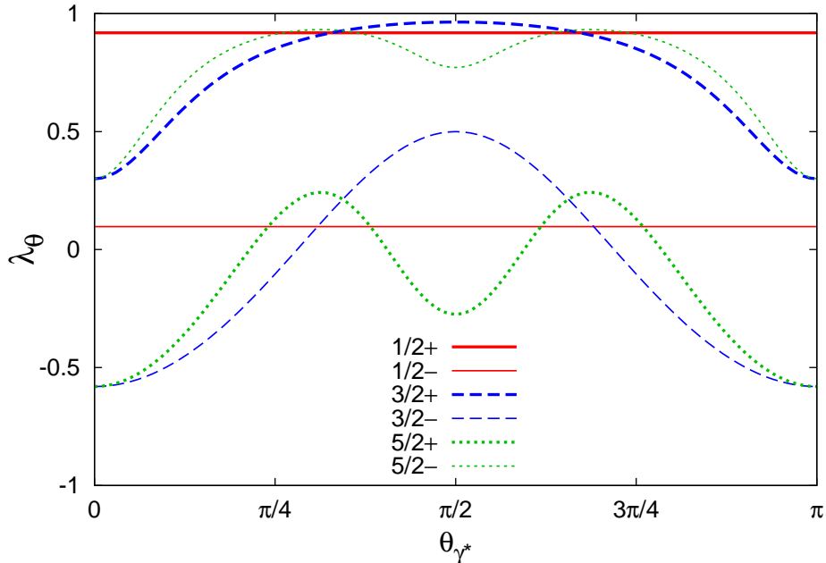
Figure 1: The anisotropy coefficient \lambda_\theta as a function of the virtual photon polar angle \theta_{\gamma^*} for hypothetical resonance states with different spins and parities in the s -channel at a dilepton mass M = 0.5 GeV. The resonance masses coincide with \sqrt{s} = 1.49 GeV, the resonance widths are \Gamma_R = 0.15 GeV.
