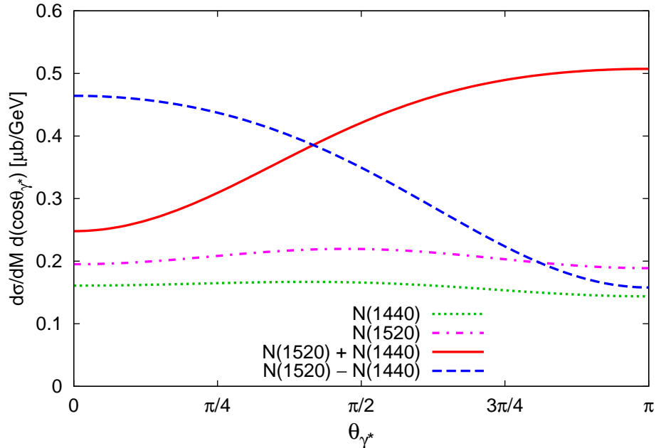
Figure 3: The contribution of the two dominant resonances, N(1440) and N(1520) , to the differential cross section of dilepton production at \sqrt{s} = 1.49 GeV CM energy. Two of the curves show the result obtained from s - and u -channel diagrams of each resonance. The other two curves are obtained from the sum of all four diagrams ( s - and u -channel diagrams of both resonances), assuming a positive and negative relative sign between the amplitudes of the two resonances.
