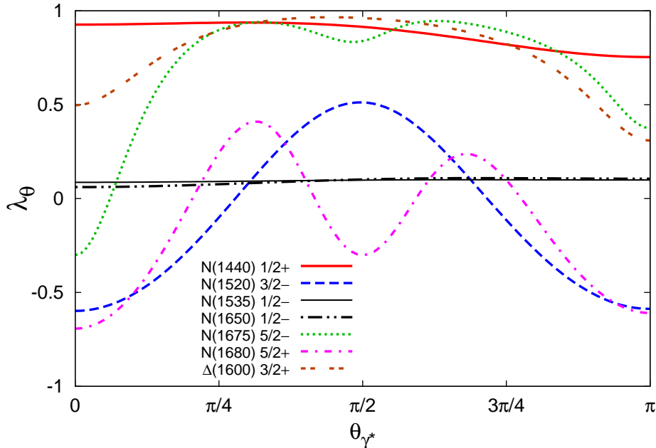
Figure 2: The anisotropy coefficient \lambda_\theta as a function of the virtual photon polar angle at a dilepton mass M = 0.5 GeV including s - and u -channel diagrams. The CM energy is \sqrt{s} = 1.49 GeV. For further details, see the text.
