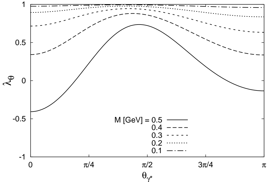
Figure 5: The anisotropy coefficient \lambda_\theta as a function of the virtual photon polar angle for various dilepton masses. The contributions of s - and u -channel diagrams of the two dominant resonances N(1440) and N(1520) and their interference term (with a positive relative sign) are included. The CM energy is \sqrt{s} = 1.49 GeV.
