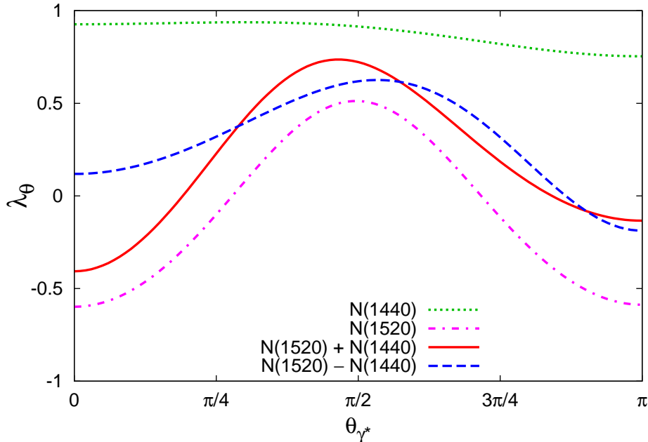
Figure 4: The contribution of the two dominant resonances, N(1440) and N(1520) , to the anisotropy coefficient, \lambda_\theta at \sqrt{s} = 1.49 GeV CM energy. The various curves correspond to the same assumptions as in Fig. 3
