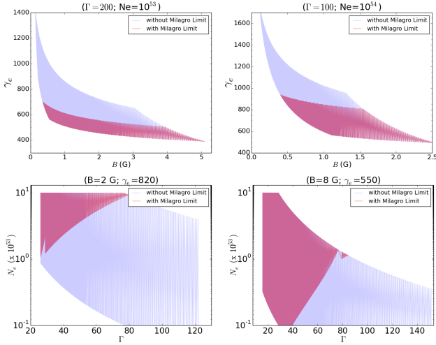
FIG. 1.— Range of parameters found using the observables of GRB080319B with and without Milagro limits. Upper panels show the electron Lorentz factor as a function of magnetic field and lower panels show the electron density as a function of bulk Lorentz factor.
