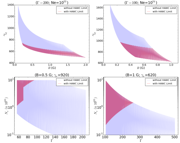
FIG. 2.— Range of parameters found using the observables of GRB130427A with and without HAWC limits. Upper panels show the electron Lorentz factor as a function of magnetic field and lower panels show the electron density as a function of bulk Lorentz factor.
