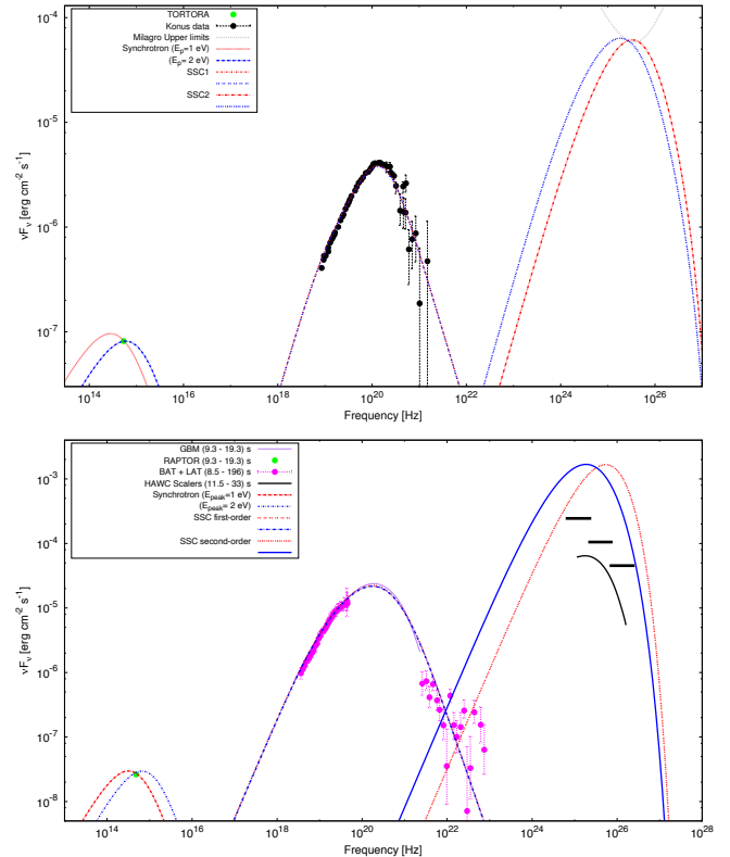
FIG. 3.— Fits of the SED of GRB 080319B (above) and GRB 130427A (below) observations with SSC model of first- and second-order. Synchrotron emission has been used to describe the optical data and the IC scattering has been used to fit MeV \gamma -ray data. We require the upper limits placed by the Milagro and HAWC experiments, respectively, to constrain the IC scattering of second order. (For details see Abdo et al. (2012); Abeysekara et al. (2015)).
