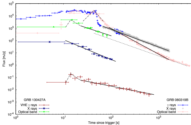
FIG. 5.— \gamma -ray, X-ray and optical light curves of GRB 080319B and GRB 130427A. The combine X-ray and Swift-BAT data are extrapolated down into the XRT energy range (0.3 - 10 keV).
