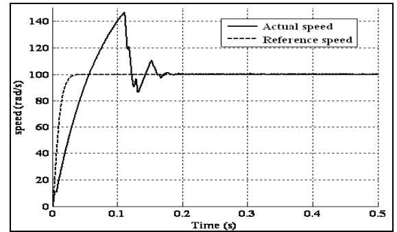
Fig. 4. Speed response without an anti-windup scheme
