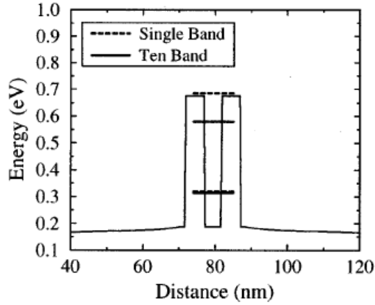
Figure 3.6.: Numerically calculated resonance energies for the InGaAs/InAlAs RTD using single and full (ten) band model [24]. Figure shows energy levels of two barriers and one well in relation to the distance from top of the device.
