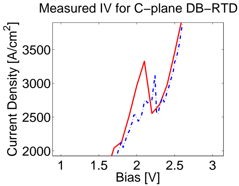
Figure 5.34.: Measured I-V characteristics of the HFTS-189 c-plane DB-RTD
