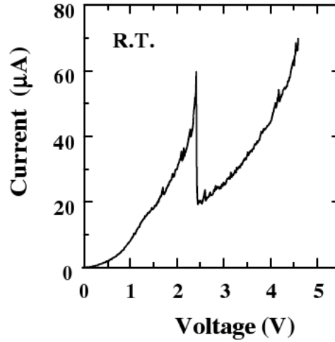
Figure 5.7.: Measured I-V curve of the RTD by Kishino et. al. [40].
