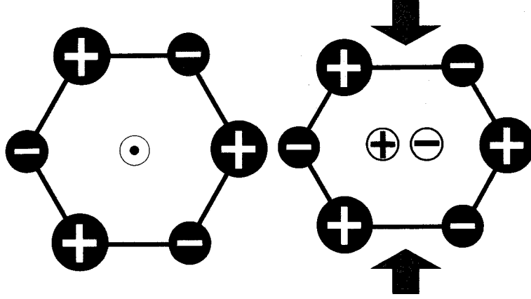
Figure 3.10.: Schematic illustration of the charge separation in c-plane GaN[18]
