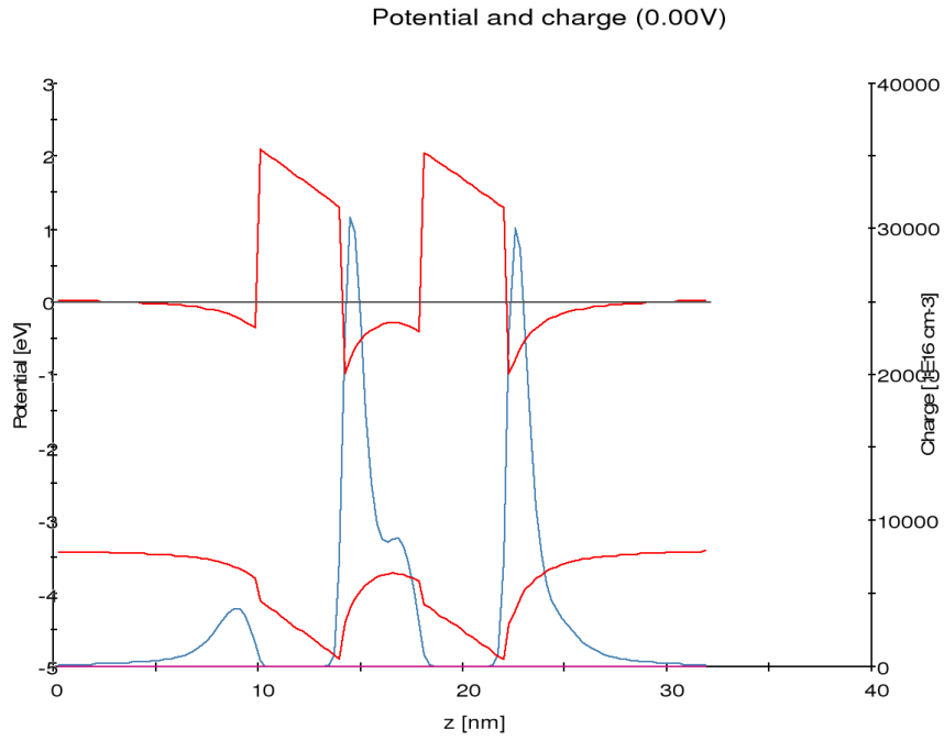
(a) V_B = 0V (Charge accumulation is visible)
