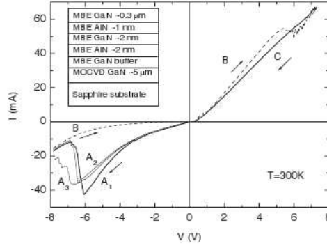
Figure 5.8.: Measured I-V curve of the RTD by Foxon et. al. [41].
