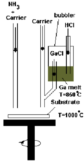
Figure 2.2.: Schematic of vertical HVPE reactor [9]
