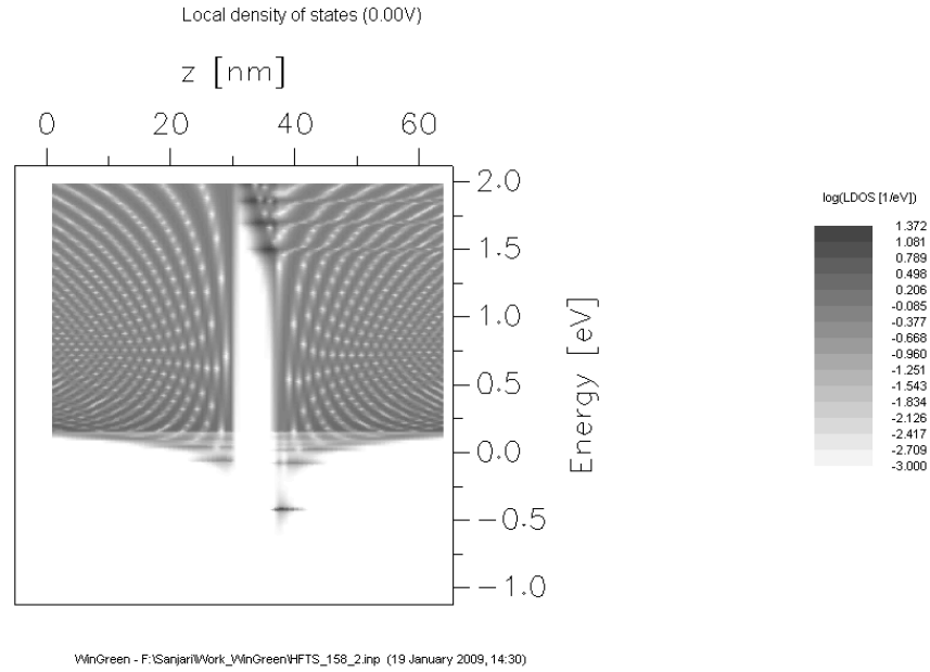
(a) V_B = 0V
