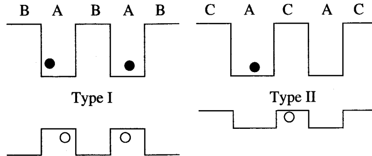
Figure 3.1.: The one dimensional superlattice in Type-I and Type-II double barrier systems [18].
