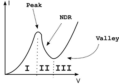
Figure 5.3.: The schematic current-voltage characteristics of NDR region [19].
