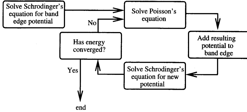
Figure 3.4.: Block diagram of self consistent iteration [18].
