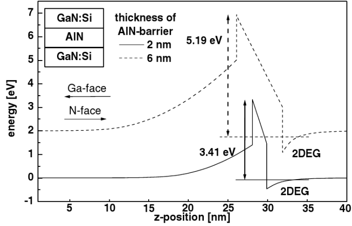
Figure 4.2.: Increase of barrier height with barrier thickness due to polarization effects [6]
