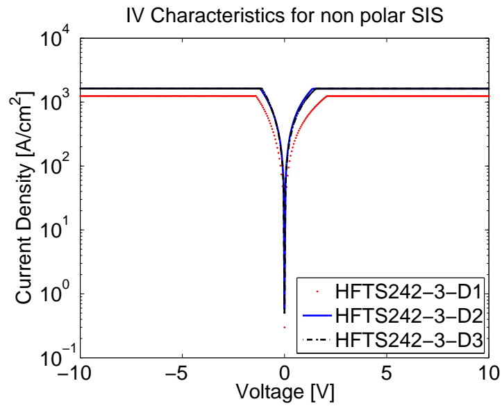
Figure 4.13.: Measured I-V curve for sample HFTS-242
