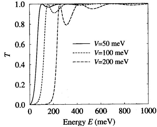
(b) Transmission coefficient as a function of energy through a 100 \text{ \AA} barrier.
