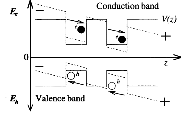
Figure 3.3.: Band tilting due to the application of an electric field[18]. Solid lines describe zero bias and dotted lines describe positive bias
