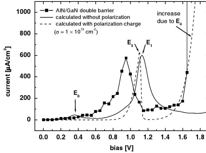
Figure 5.9.: Measured I-V curve of the RTD by Hermann et. al. [6].
