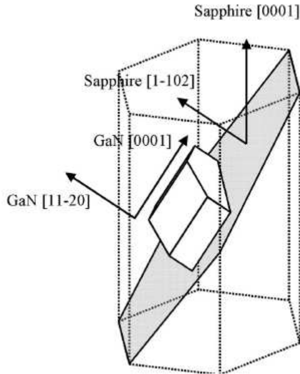
Figure 2.6.: Schematic representation of crystal directions in sapphire and GaN [13]
