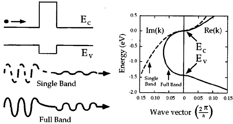
Figure 3.7.: Comparison between 1-band model and full (ten) band model [24].
