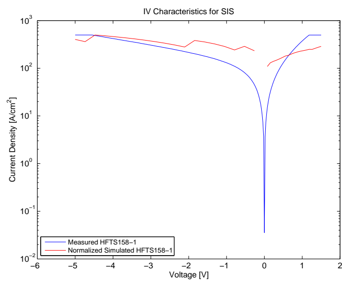
Figure 4.15.: The comparison between the simulated and measured I-V for the HFTS-158
