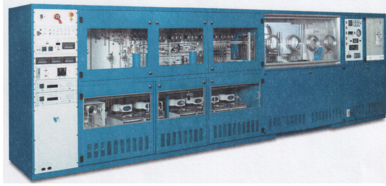
Figure 2.1.: Our MOCVD equipment in the lab [8]
