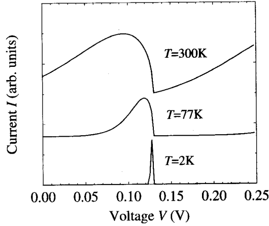
Figure 5.4.: Temperature dependent current-voltage curve for the 100\text{\AA} Al_{0.2}Ga_{0.8}As/50\text{\AA} GaAs/100\text{\AA} Al_{0.2}Ga_{0.8}As of the Figure 5.1(b) [18]
