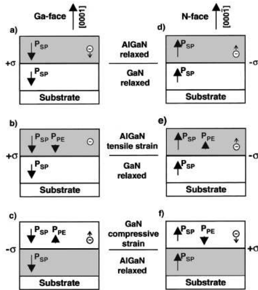
Figure 2.4.: Directions of spontaneous and piezoelectric polarization [12]
