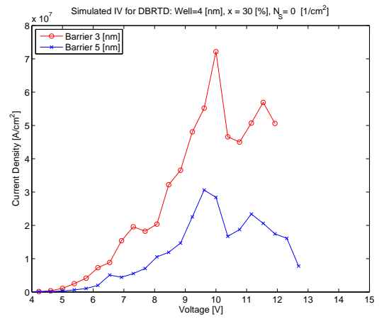
Figure 5.27.: Well=4nm,x=30%
