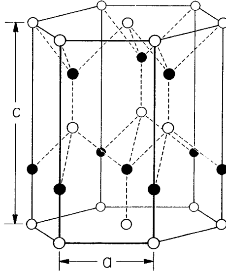
Figure 2.3.: The wurtzite crystal structure [11]
