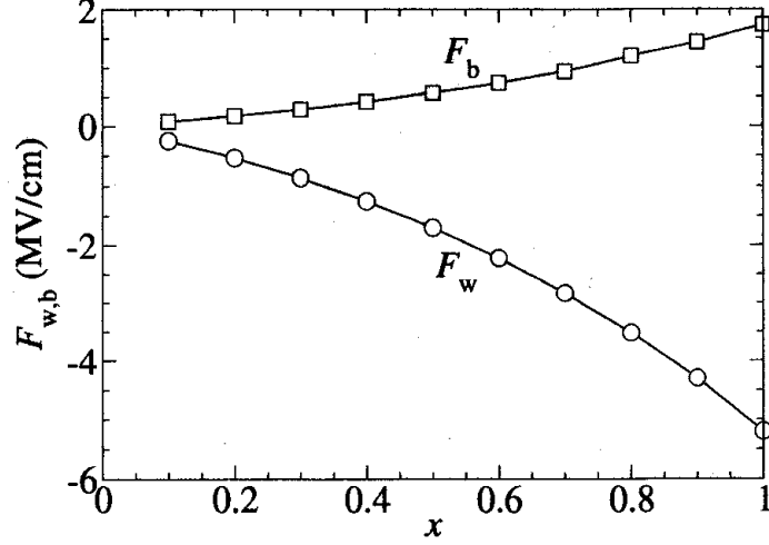
Figure 3.11.: Calculated induced piezoelectric field in GaN F_w well and two Al_xGa_{1-x}N barrier layers F_b [18].
