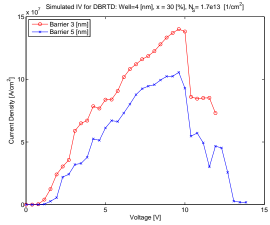
Figure 5.17.: Well=4nm,x=100%, \sigma = 5.6 \times 10^{13} \text{ cm}^{-2} Figure 5.18.: Well=4nm,x=30%, \sigma = 1.7 \times 10^{13} \text{ cm}^{-2}
