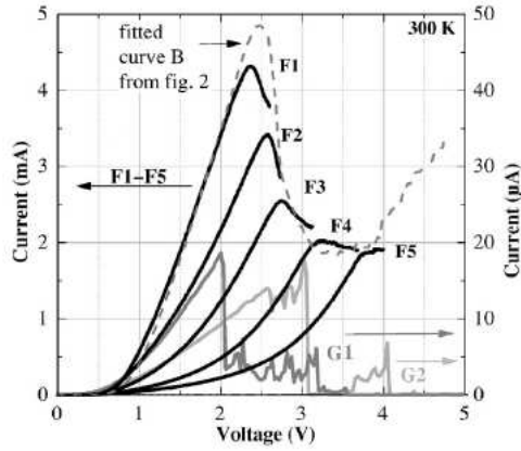
Figure 5.11.: Measured retrace of the I-V curve of the RTD by Golka et. al. [42].
