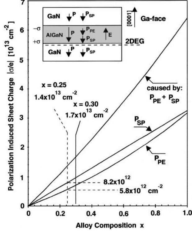
Figure 5.13.: Calculated polarization induced charges vs. alloy composition [12].
