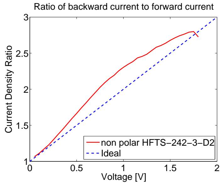
Figure 4.14.: Difference in the measured forward and backward voltages for non polar sample HFTS-242
