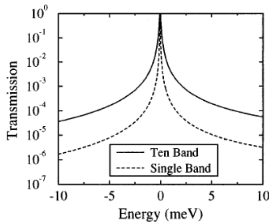
Figure 3.8.: Transmission coefficient versus energy for single and full (ten) band models [24].
