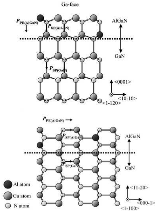
Figure 2.4.: Directions of spontaneous and piezoelectric polarization [12]
