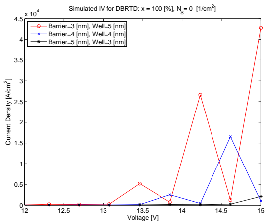
Figure 5.28.: Barrier=4nm,x=100%
