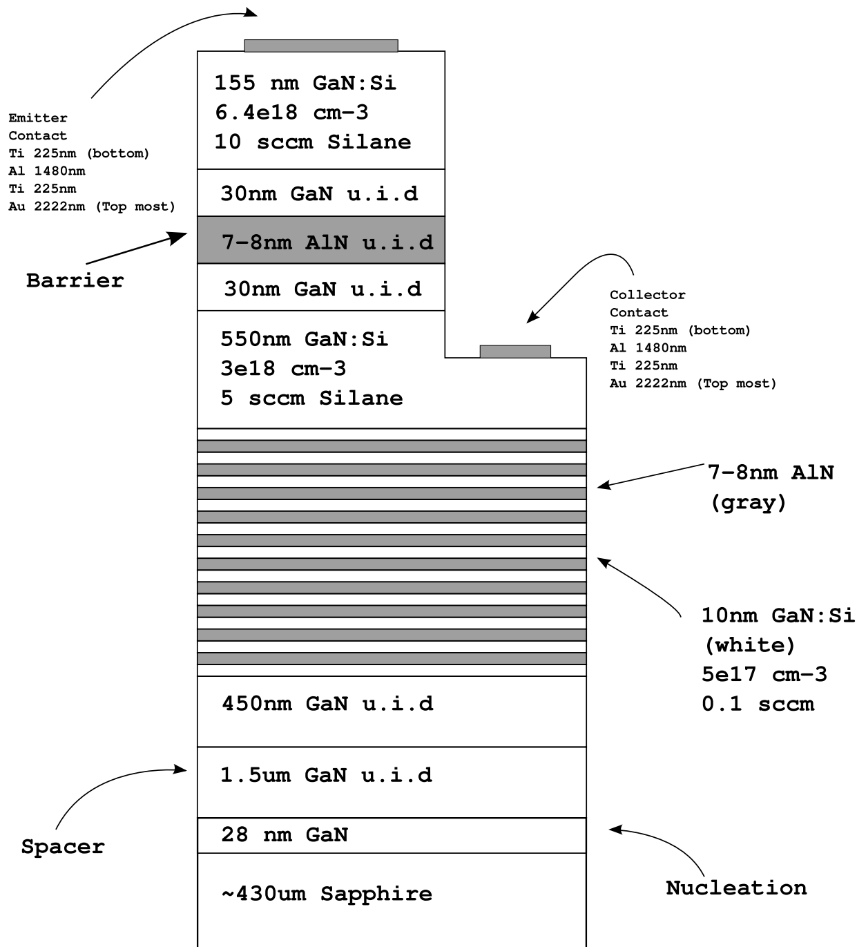
Figure 4.8.: Growth structure of HFTS-158 (not to scale)
