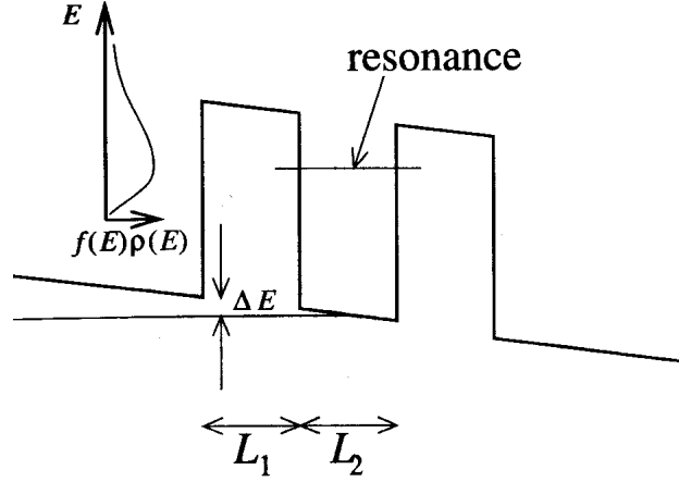
Figure 5.2.: Simple model of current flow through a double barrier structure [18].
