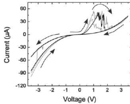
Figure 5.12.: Measured I-V curve of the RTD by Leconte et. al. [43].
