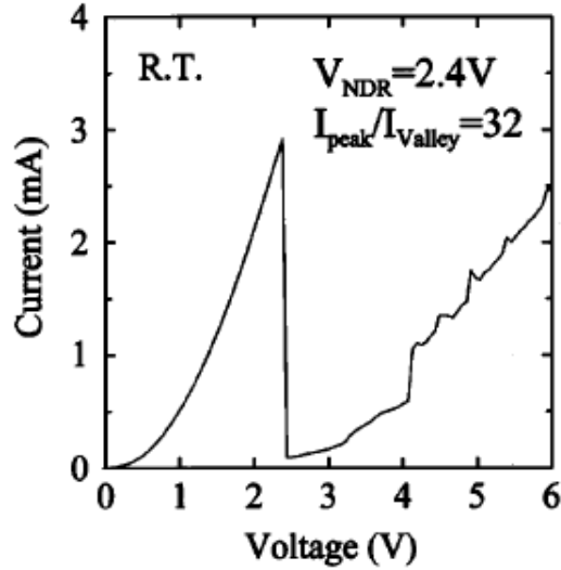
Figure 5.6.: Measured I-V curve of the RTD by Kikuchi et. al. [37] and [38].
