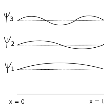
Figure 3.2.: The first three allowed standing waves for a particle in a box [19].
