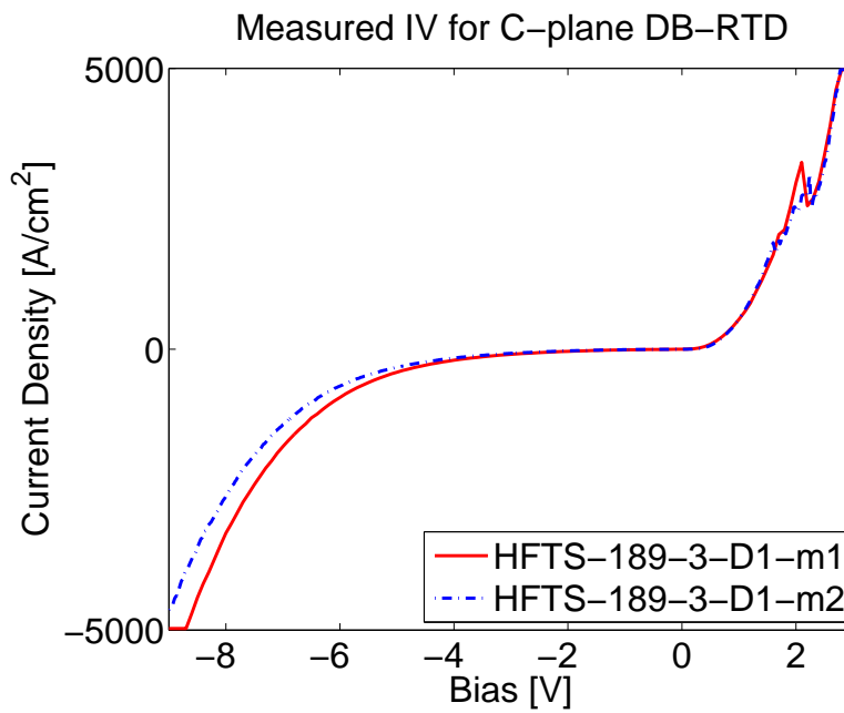
Figure 5.35.: Zoomed out: Measured I-V characteristics of the HFTS-189 c-plane DB-RTD
