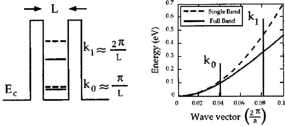
Figure 3.5.: (Left) Approximate resonant energies. (Right) Band structure of a typical III-V calculated by full (ten) and single band models [24].
