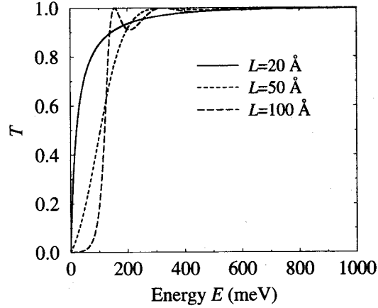
(a) Transmission coefficient as a function of energy through different barrier widths.
