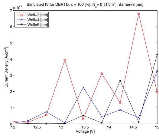
Figure 5.32.: Barrier=3nm, x=100%
