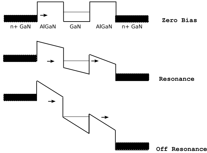
Figure 5.5.: The negative resistance in a double barrier structure, after [19]. Arrows show direction of electron transport
