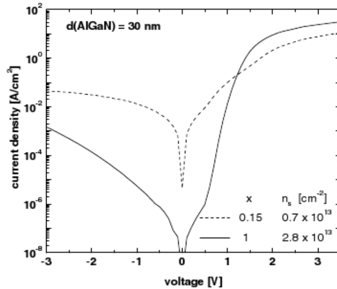
Figure 4.3.: The calculated I-V curve for different sheet carrier densities [6]
