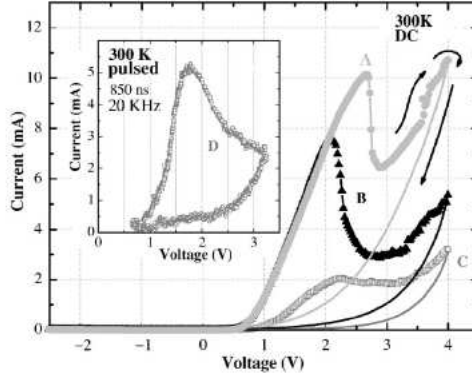
Figure 5.10.: Measured I-V curve of the RTD by Golka et. al. [42].
