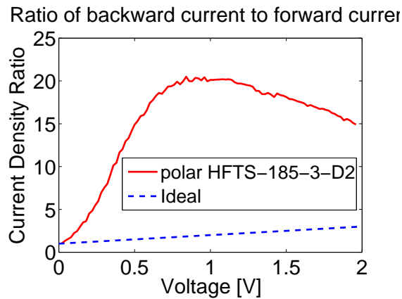
Figure 4.12.: Difference in the measured forward and backward voltages for c-plane sample
