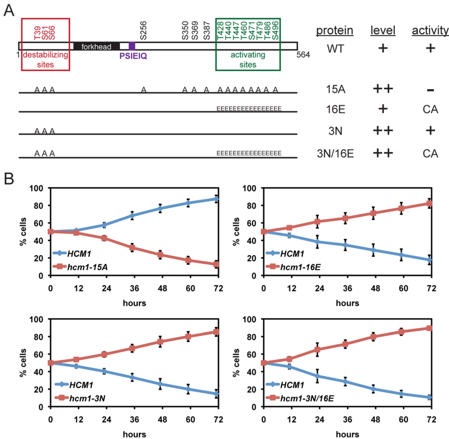
FIGURE 1: Hcm1 phosphorylation affects cellular fitness. (A) Positions of Cdk1 phosphosites that activate (green) and destabilize Hcm1 (red). Mutations that block degradation lead to an increase in protein level (15A, 3N, 3N/16E); phosphomimetic mutations (16E, 3N/16E) lead to constitutive activity (CA). (B) Strains expressing PGK1-URA3 (blue lines) and PGK1-GFP-URA3 (red lines) were cocultured and the percentage of each strain in the population determined at the indicated time points. Average values \pm 1 SD of five to eight replicates.
