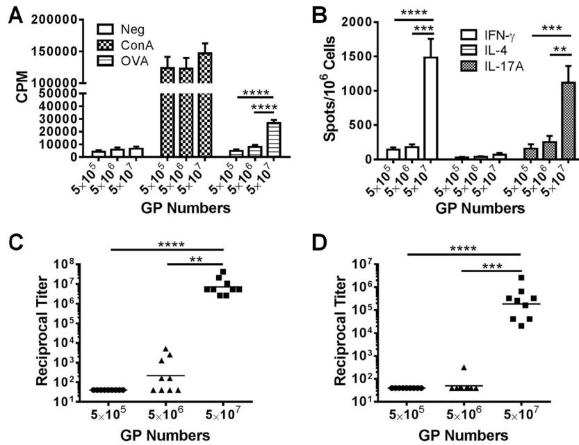
FIG 3 Effect of GP number and antigen concentration on immune responses. Mice were immunized three times at 2-week intervals with the indicated number of GP-OVA/tR (containing 50 \mu g OVA per 5 \times 10^7 particles; 5 \mu g OVA per 5 \times 10^6 particles; 0.5 \mu g per 5 \times 10^5 particles). Two or 4 weeks after the last immunization, CD4 + T-cell lymphoproliferation (A), ELISpot (B), IgG1 ELISA (C), and IgG2c ELISA (D) were performed. Data shown are combined results from two independent experiments with 4 or 5 mice per group for each experiment. Some of the data for the 5 \times 10^7 GP group are also used in Fig. 1 (part of the GP-OVA/tR group) and Fig. 2 (50 \mu g OVA group). **, P < 0.01 ; ***, P < 0.001 ; ****, P < 0.0001 .
