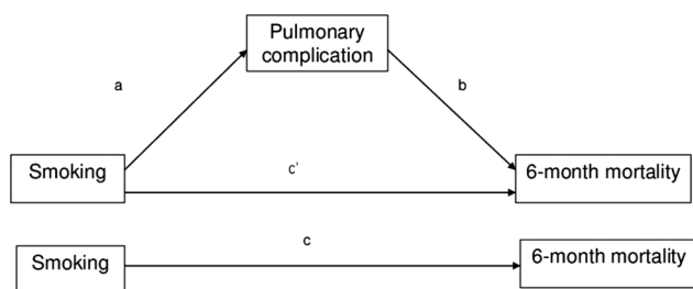
Figure 1 Path diagram of the relations among the three standardised variables and standardised coefficients of paths. a=regression coefficient for path from smoking to pulmonary complications; b=regression coefficient for path from pulmonary complications to 6-month mortality, controlling for smoking; c'=regression coefficient for path from smoking to 6-month mortality, controlling for pulmonary complications; c=regression coefficient for direct path from smoking to 6-month mortality. Smoking is the independent variable, pulmonary complications the mediator and 6-month mortality dependent variable. a, b, c and c' are coefficients from logistic regression analyses.
