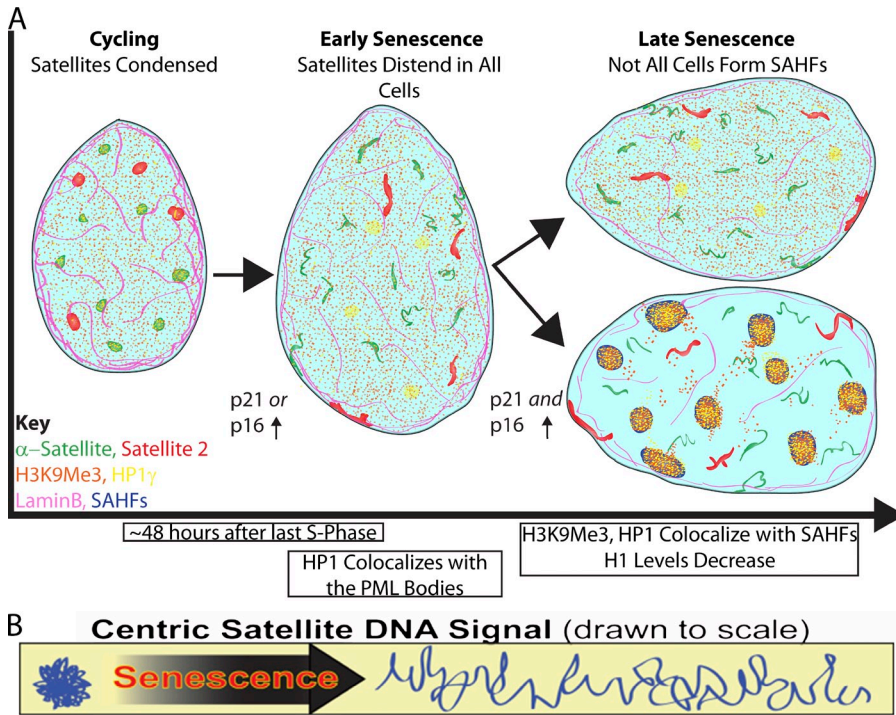
Figure 8. Satellite distension in relation to other events in the cell senescence process. (A) In nuclei of cycling cells, the peri/centromeric satellite DNA signals are tightly compacted, but dramatically distend in senescent cells. This occurs before and irrespective of the later formation of SAHF, and in some cells within 48 h of the last S phase. SADS is seen in essentially all noncycling cells and occurs in cells that first up-regulate either the p21 or p16 pathway. In late stage senescence, both pathways are up-regulated, and the p16 pathway promotes formation of SAHF. During this process there is a reorganization of several heterochromatin factors as seen by immunofluorescence including H3K9Me3 and HP1 \gamma , whereas H1 levels uniformly decrease with the formation of SAHF. Whereas nuclear diameter increases progressively and is most pronounced in cells with SAHF, SADS are seen in some cells before nuclear enlargement. The nuclear lamina protein (LaminB1) may play a role in the higher-order folding of the DNA as it is diminished in most cells before SADS form. (B) Sat DNA in cycling cells is tightly packaged and this packaging is lost during senescence as the DNA distends. Because three canonical histone modifications remain unchanged during senescence the difference in DNA packaging may be attributed to changes in higher-order folding.
