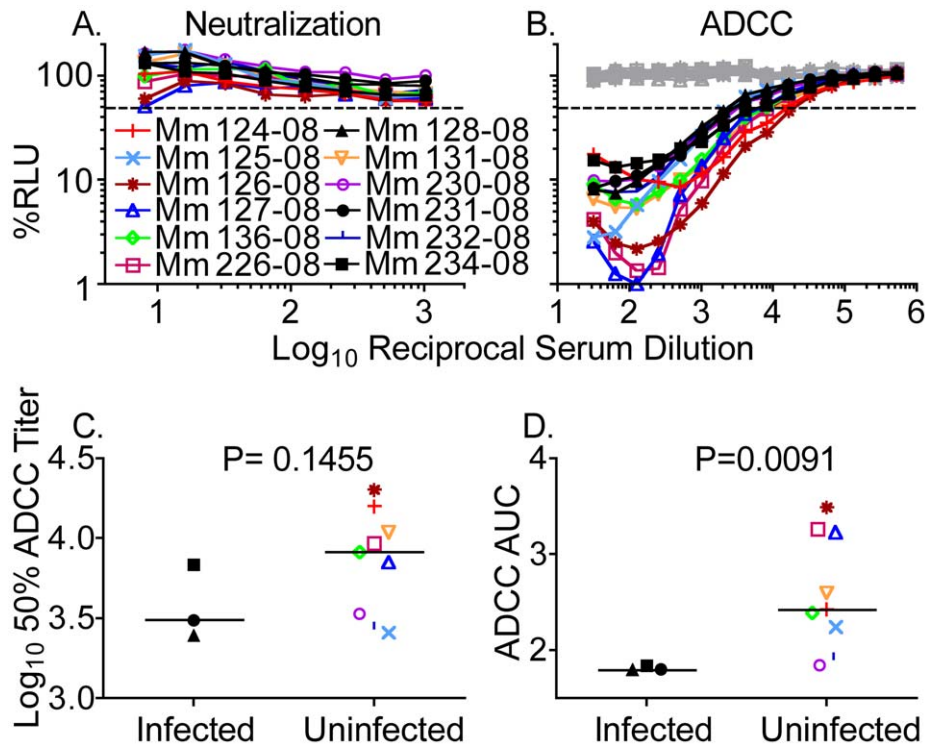
Figure 5. Neutralization and ADCC on the day of intravenous challenge with SIV_{mac251NE} . Macaques were challenged with an intravenous dose of SIV_{mac251NE} on week 46 after inoculation with SIV_{mac239\Delta nef} or SIV_{mac239\Delta nef/E543-3env} . Sera collected the day of challenge were evaluated for neutralization of SIV_{mac251NE} (A) and ADCC against SIV_{mac251NE} -infected cells (B). Solid black symbols indicate animals that became infected by SIV_{mac251NE} . Dashed lines indicate 50% activity. Target cells infected with SHIV_{SF162P3} served as a negative control for ADCC assays (gray). Differences in 50% ADCC titers were not significant (C). However, AUC values for ADCC were higher among the immunized animals that remained uninfected versus the immunized animals that became infected (2-tailed Mann-Whitney U test, P=0.0091 ) (D). None of these macaques had the MHC class I alleles Mamu-A*01 , -B*08 or -B*17 associated with reduced viral replication [67–69]. doi:10.1371/journal.ppat.1002890.g005
