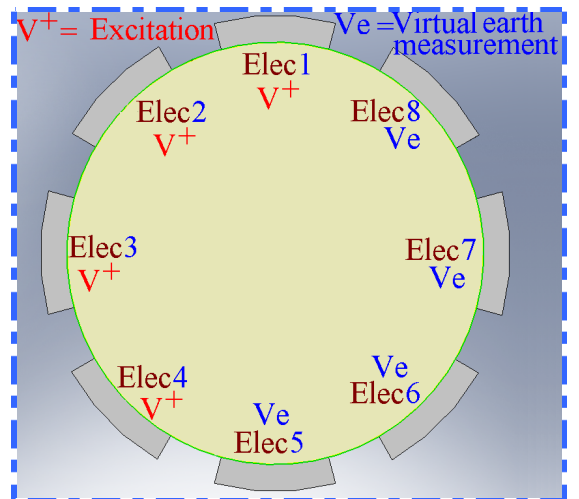
Fig. 3 Array A electrode configuration
