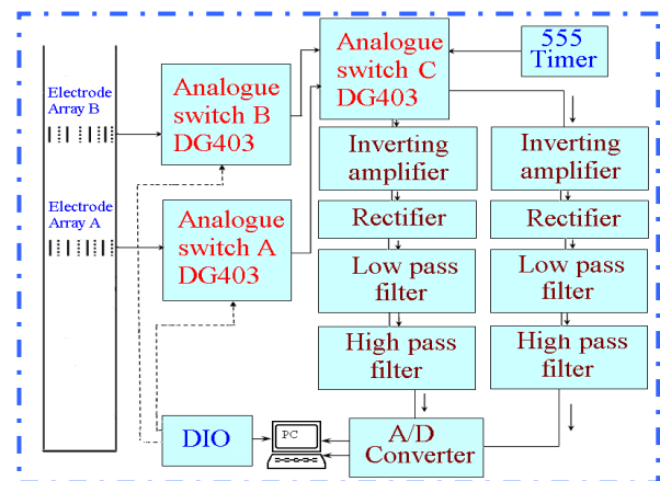
Fig. 1 Schematic diagram of the data acquisition and control system
