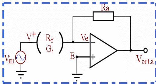
Fig. 4 Fluid conductance circuit
