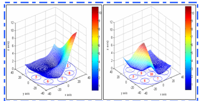
(a) Config-5 (b) Config-6 Fig. 9 Sensitivity distributions
