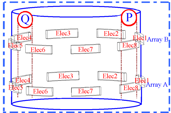
Fig. 12 Arrangement of electrode array on the pipe
