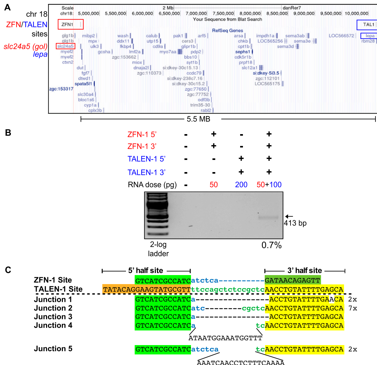
Figure 4. TALEN/ZFN-generated 5.5-Mb deletions on chromosome 18. (A) Schematic diagram of the target region within chromosome 18 demarcating the position of the ZFN target site in the slc24a5 ( golden ) locus and the TALEN target site in the lepa locus. (B) Segmental deletions of 5.5 Mb are detected in normal-appearing nuclease-treated embryos when the ZFN and TALEN RNAs are coinjected. The presence or absence of each nuclease component (5' and 3' recognition unit) is indicated above each gel lane, as is the dose of each component. PCR products corresponding to the desired 5.5-Mb segmental deletion (413 bp) are detected only in embryos injected with both nucleases. The estimated deletion rate is indicated below the positive lane. (C) Junction sequences for the 5.5-Mb segmental deletions on chromosome 18. The nuclease recognition sequences are indicated above the junction sequences, where the half-sites are differentially colored. In the recovered junction sequences, there are variable length deletions as well as evidence of insertions between some of the target sites, where the latter are indicated in plain text.
