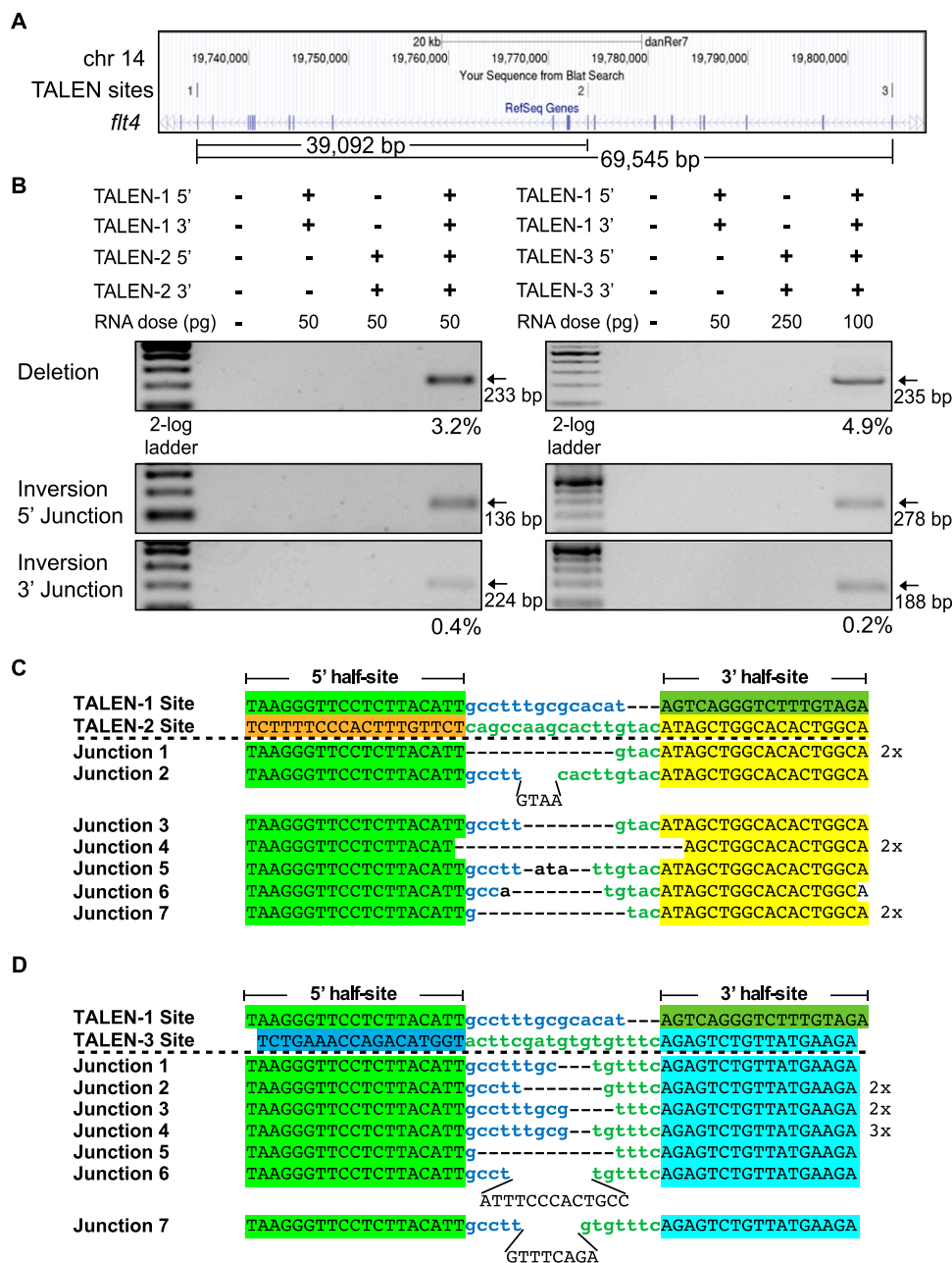
Figure 3. TALEN-generated 39-kb and 69-kb deletions within the zebrafish flt4 locus. (A) Schematic diagram of the flt4 locus demarcating the positions of all three TALEN binding sites and the distance separating them. (B) Segmental deletions of 39 and 69 kb are readily detected in normal-appearing TALEN-treated embryos when two TALENs are coinjected. The presence or absence of each TALEN component (5' and 3' recognition unit) is indicated above each gel lane, as is the dose of each TALEN component. PCR products corresponding to the desired 39-kb and 69-kb segmental deletion products are detected only in embryos injected with both TALENs. Estimated deletion rates are indicated below the positive lanes. Segmental inversions are detected in embryos treated with two TALENs for both segments, but at lower rates than the corresponding segmental deletions. Junction sequences for the 39-kb (C) and 69-kb (D) segmental deletions at the flt4 locus. The TALEN-1 and TALEN-2/3 recognition sequences are indicated above the junction sequences, where the half-sites recognized by each TALEN are differentially colored. In the recovered junction sequences, there are variable length deletions as well as evidence of insertions between some of the target sites, where the latter are indicated in plain text.
