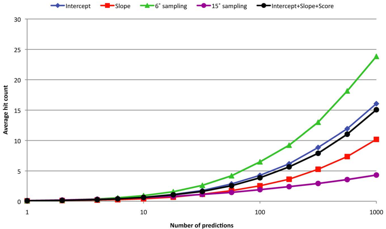
Figure 9. Average hit count for 15° and 6° rotational sampling, the Intercept and Slope funnel properties (based on 10 closed neighbors using angular distance), and the scores and properties combined in a weighted linear function (training and testing using 22-fold cross validation).
