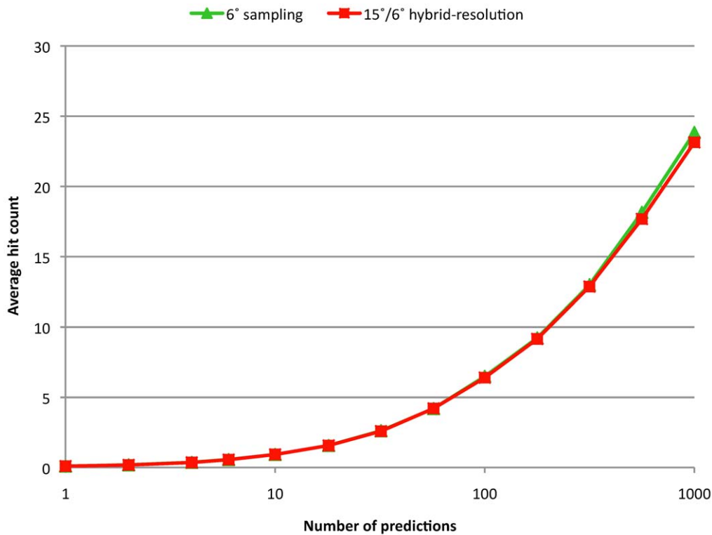
Figure 4. Average hit count for the standard 6° rotational sampling and the hybrid-resolution approach. doi:10.1371/journal.pone.0056645.g004
