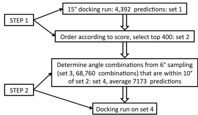
Figure 2. Schematic overview of the hybrid-resolution approach.
