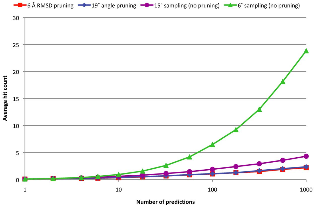
Figure 7. Average hit count for 15° and 6° rotational sampling, and for 6° rotational sampling with 19° angular distance pruning or 6 Å RMSD pruning.
