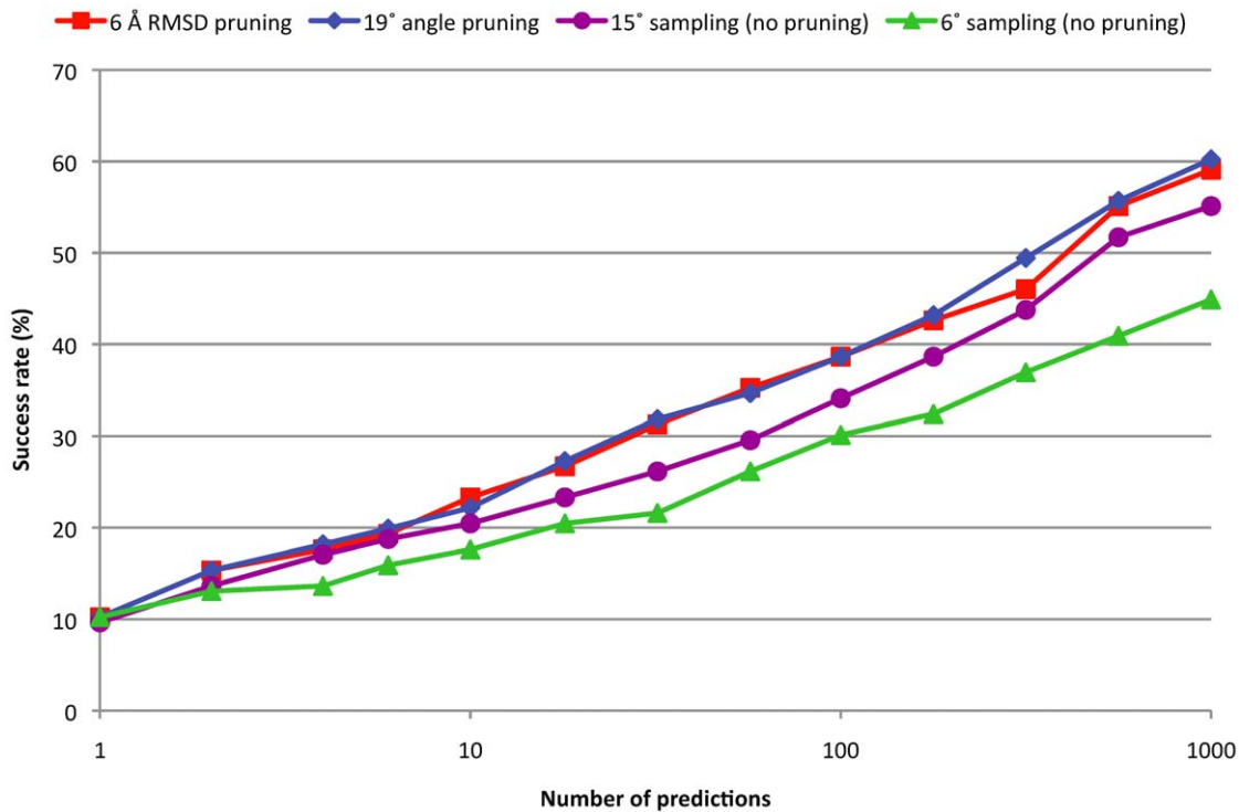
Figure 6. Success rate for 15° and 6° rotational sampling, and for 6° rotational sampling with 19° angular distance pruning or 6 Å RMSD pruning.
