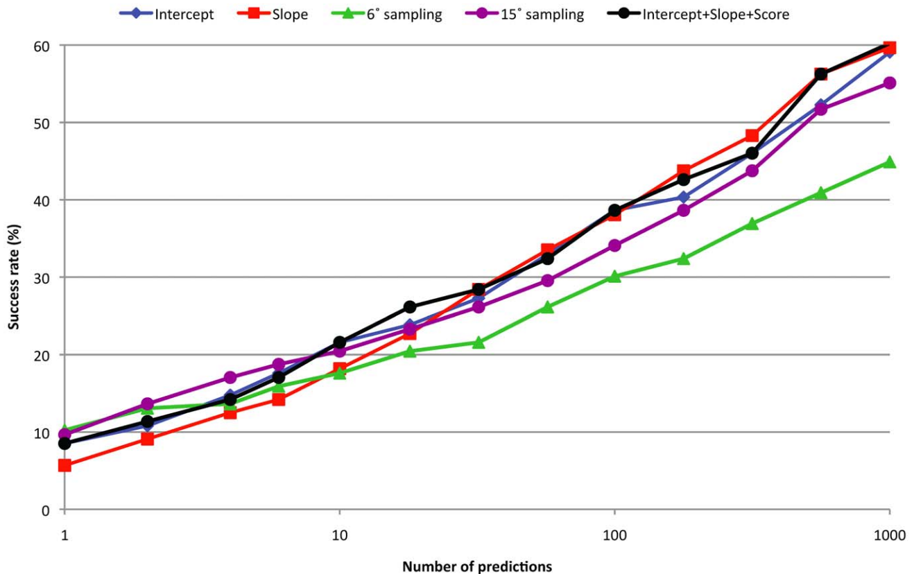
Figure 8. Success rate for 15° and 6° rotational sampling, the Intercept and Slope funnel properties (based on 10 closed neighbors using angular distance), and the scores and properties combined in a weighted linear function (training and testing using 22-fold cross validation).
