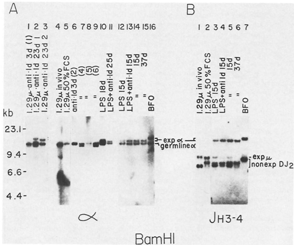
FIGURE 8. Blots of I.29 cell DNA digested with Bam HI. DNA were prepared from untreated I.29 \mu or BFO.3 cells, or from cultures of I.29 \mu cells that had been treated with the indicated reagents. Blots were annealed with the \alpha (A) or JH3-4 (B) probes. (A) The Bam HI fragments (12.6–15 kb) labeled expressed ["(exp) \alpha "] in A, lanes 2 and 3 and 10–16, co-migrated with bands detected by the JH3-4 probes (B, lanes 3–7). (JH3-4 data for lanes 2 and 3 in A are not shown.) The germline \alpha band did not comigrate with bands detected by the JH3-4 probe. Smaller \alpha gene fragments present in lanes 1 and 2 and 7–9 in A also did not comigrate with bands detected with the JH3-4 probe. (B) The JH3-4 probe detected: (1) the expressed \alpha segment (12.6–15 kb), (2) the expressed \mu segment, which was slightly larger (8.3 kb) in the in vivo line of I.29 \mu cells (lane 1) than in the in vitro lines (8 kb) (lanes 2–5), and (3) smaller fragments from the nonexpressed DJ 2 -C \mu segment, which comigrated with fragments detected by the M2-5B probe (not shown), except in BFO cell DNA (lane 7), where the nonexpressed DJ segment comigrated with a fragment detected by the \gamma_3 probe (not shown). The percent of the cells that were IgA + in the cultures analyzed in A were: (1) 3, (2) 30, (3) 50, (4–7) 0, (8) 1.1, (9) 2, (10) 27, (11) 99, (12) 32, (13) 74, (14) 58, (15) 100, and (16) 100 cloned IgA + cell line. The DNAs present in lanes 12–16 in A were identical to those present in lanes 3–7 in B.
