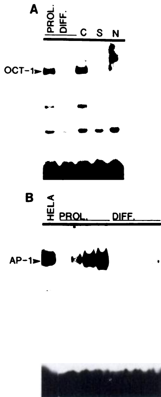
Fig. 9. A, regulation of OCT-1 binding activity to the H2B histone gene promoter during differentiation of normal rat osteoblasts. Each lane contains 1 µg of nuclear protein. Lanes C, S, and N, competition with 1 µg of HeLa nuclear extract. Lane C, no competitor (C); Lane S, OCT-1 oligonucleotide as specific competitor; Lane N, with Sp1 as nonspecific competitor oligonucleotide. The same probe and competitor DNA fragments were used as described in Fig. 5A. B, regulation of AP-1 binding activity during osteoblast differentiation. Lane HELA, 4 µg of HeLa nuclear extract. PROL., 1.6, 3.1, 4.7, and 6.3 µg of proliferating ROB cells; DIFF., 1.1, 2.2, 3.3, and 4.4 µg of differentiated ROB nuclear extracts. The probe spans an AP-1 consensus sequence (see Fig. 5B).
