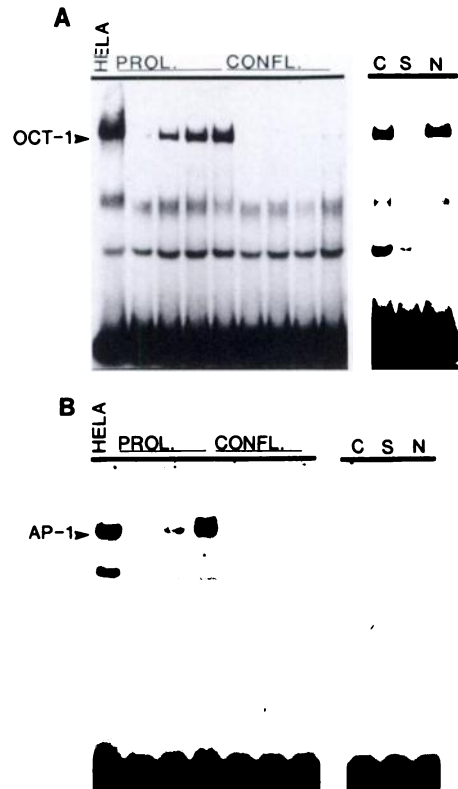
Fig. 5. A , OCT-1 binding activity decreases during density inhibition of rat osteosarcoma cells. Lane HELA , 1 \mu g HeLa nuclear protein. The amounts of protein loaded from proliferating ROS (Lanes 2–5 from the left) and from density-inhibited ROS (Lanes 6–9 from the left) cells were, respectively, 0.4, 0.8, 1.1, and 1.5 \mu g in each set. The probe used a synthetic oligonucleotide spanning an OCT-1 element of a human H2B gene (51), and 2 \mu g of poly (dI-dC)-poly (dI-dC) were present in the binding reaction. Competition analysis was performed with the unlabeled OCT-1 DNA fragment (Lane S ), with the Sp1 oligonucleotide (Lane N ), or in the absence of competitor DNA fragments (Lane C ) using 1 \mu g HeLa nuclear protein. B , AP-1 binding activity is present in proliferating ( PROL. ) but not in confluent ( CONFL. ) ROS cells. For both nuclear extract preparations, binding reactions contained, respectively, 2.5, 3.8, and 5 \mu g protein. Competition analysis was performed with 5 \mu g protein from confluent ROS 17/2.8 cells using the following DNA fragments, respectively: Lane 3 from the left, no competitor DNA added ( C ); Lane 4 from the left, AP-1 as specific competitor ( S ) and lane 5 with Sp1 as nonspecific competitor ( N ). The probe is a synthetic AP-1 consensus oligonucleotide (26), and 2 \mu g of poly (dI-dC)-poly (dI-dC) were present in the binding reaction. The protein/DNA complexes were separated on a 4% (40:1) polyacrylamide gel using TGE buffer.
