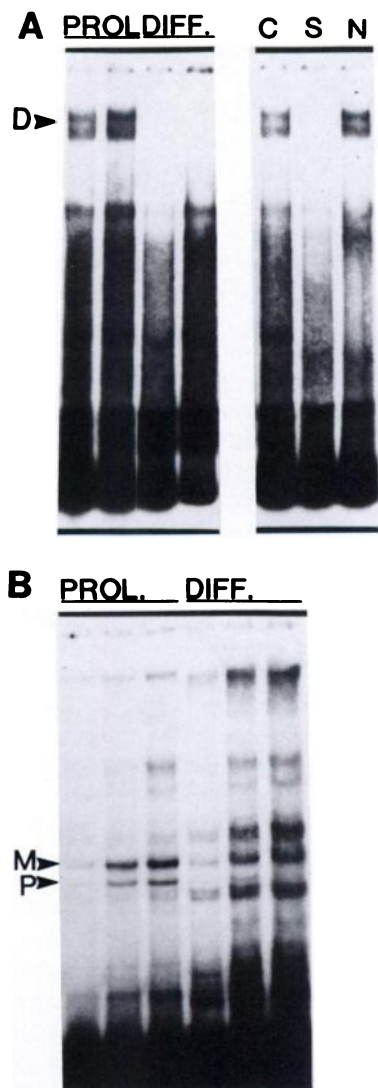
Fig. 7. A, protein/DNA interactions to Site II of the H4 histone gene promoter during differentiation of normal rat osteoblasts. The autoradiogram shows a gel shift assay indicating that HiNF-D binding activity is detectable in nuclear extracts from proliferating rat osteoblasts (Lanes 1 and 2 from the left, 2 and 4 \mu g, respectively) but not in differentiated rat osteoblasts (Lanes 3 and 4 from the left, 1.9 and 3.8 \mu g, respectively). Competition analysis is shown in the last 3 lanes on the right. Reactions were performed in the absence of competitor (C, control) or in the presence of a 100-fold molar excess of specific (S, TM3) or nonspecific (N, DD-1) competitor DNA fragment (17). Binding reactions were performed using the nt -130 to -38 promoter fragment of the H4-F0108 gene cloned in pFP-1 (43) in the presence of 2 \mu g of poly (dG-dC)-poly (dG-dC). B, regulation of HiNF-P and HiNF-M binding activity during rat osteoblasts differentiation (PROL., 2.6, 3.9, and 5.2 \mu g; DIFF., 2.8, 4.1, and 5.5 \mu g). Reactions were performed using a fragment spanning nt -97 to -38 of the histone H4-F0108 gene promoter in the presence of 1 \mu g salmon sperm DNA.
