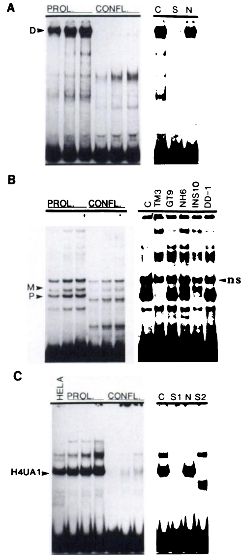
Fig. 3. Protein/DNA interactions at Sites II and III of the H4 gene promoter during growth inhibition of ROS 17/2.8 cells. In A, HiNF-D activity is detectable in proliferating rat osteosarcoma cells ( first 3 lanes from the left , 2.5, 3.8, and 5 \mu g nuclear protein, respectively) but not in density-inhibited ROS cells ( middle 3 lanes, left to right , 2.5, 3.8, and 5 \mu g, respectively). Competition analysis was performed in the presence of 5 \mu g protein from proliferating ROS 17/2.8 cells with a 100-fold molar excess of either a specific oligonucleotide spanning the HiNF-D binding site (designated TM3; Lane 5 ) that competes or a HiNF-D mutant oligonucleotide (SUB-11; Lane N ) that does not compete (17). The probe spans H4-Site II (nt -97 to -38) of the H4 gene promoter ( EcoRI/HindIII fragment of pFP202 (41)). B, HiNF-M binding activity is detectable in proliferating as well as in density-inhibited rat osteosarcoma cells, whereas the level of HiNF-P decreases to below the limit of detection during growth inhibition. Nuclear extracts from both proliferating ( PROL ) and confluent ( CONFL ) ROS 17/2.8 cells were used in the assay. The amount of nuclear protein used in each binding reaction was, respectively, 5, 7.5, and 10 \mu g for each preparation. Competition analysis is shown in 5 right-hand lanes using oligonucleotides (described in detail in Ref. 17) that compete for both HiNF-P and HiNF-M (TM3) or specifically compete for either HiNF-P (NH6) or HiNF-M (DD-1) and specifically mutated DNA fragments that do not compete for HiNF-P (GT9) or HiNF-M (INS10). ns , nonspecific complex. The probe fragment encompasses Site II of the histone H4-FO108 gene promoter and spans nt -97 to -38; binding reactions were performed in the presence of 1 \mu g salmon sperm DNA. In C, H4UA-1 binding activity decreases during osteosarcoma cell growth inhibition. Shown is a gel retardation assay monitoring the abundance of H4UA-1 binding activity interacting with Site III of the H4 gene promoter using nuclear extracts from proliferating ( PROL ) and density-inhibited ( CONFL ) ROS 17/2.8 cells. The amounts of protein loaded for each extract were, respectively, 2.5, 3.8, and 5 \mu g. First lane on the left , pattern obtained using 5 \mu g of protein from HeLa S3 cells. Competition analysis was performed with 5 \mu g protein from proliferating ROS 17/2.8 cells in the absence of competitor DNA (C) or in the presence of specific competitor (S1, H4 Site III, spanning nt -369 to -323; S2, proximal part of H4 Site III (nt -349 to -323) or nonspecific competitor (N; distal part of H4 Site III (nt -369 to -349)). The probe for H4 Site III encompasses nt -326 to -371 and was used in the presence of 2 \mu g poly (dA-dT)-poly (dA-dT) DNA and 1 \mu g poly (dI-dC)-poly (dI-dC) as described previously (33).
