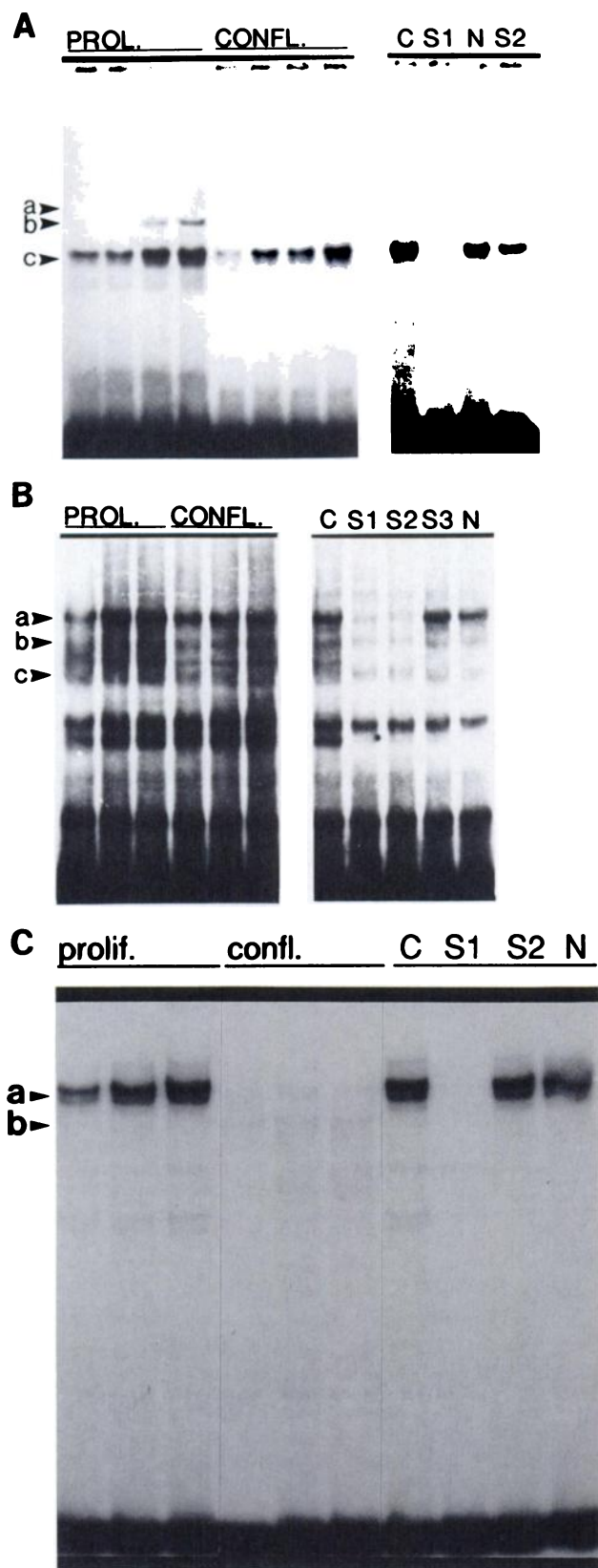
Fig. 6. Protein/DNA interactions in the osteocalcin gene promoter during growth inhibition of rat osteosarcoma cells. A , nuclear proteins interacting with the rat vitamin D-responsive element (nt -462 to -437) are observed in both proliferating ( PROL ) and density-inhibited ( CONFL. ) ROS cells (for each set, respectively, 1.25, 2.5, 3.8, and 5 \mu g protein were used). Competition assays were performed with 5 \mu g of nuclear extract derived from proliferating ROS cells using a panel of oligonucleotides ( S1 , unlabeled rat osteocalcin VDRE; N , Sp1; S2 , human osteocalcin VDRE). In B , the protein/DNA interactions at the osteocalcin box are similar in proliferating ( PROL ) and confluent ( CONFL. ) ROS cells. Increasing amounts of nuclear protein were used in each
