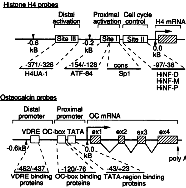
Fig. 2. The probe DNA fragments used in this study are shown relative to the modular organization of a prototypical cell cycle-regulated histone H4 gene promoter ( top ) and the bone-specific OC gene promoter ( bottom ). The nucleotide positions are indicated for each probe, except the Sp1 oligonucleotide, which conforms to an Sp1 consensus element. The histone H4 promoter contains a series of proximal and distal transcriptional domains (H4 Sites I to III) ( boxes ). These domains are bipartite and multipartite, and each interacts with several promoter factors as indicated (e.g., HiNF-D, Sp1, and H4UA-1; reviewed in Refs. 14 and 17). The osteocalcin promoter contains steroid hormone response elements (e.g., VDRE) and basal tissue-specific elements (OC box and TATA box). Whereas the OC gene represents a single gene in the rat genome (28), the H4 gene is present in multiple copies (44), each with a different organization of promoter elements. The distribution of protein/DNA interactions indicated in the diagram represents that of the human H4-FO108 gene, which has been most extensively studied (14, 17). Each of the evolutionarily conserved promoter elements depicted here has homologous counterparts in the promoters of several other vertebrate H4 genes, as well as other histone gene subtypes (17, 44).
