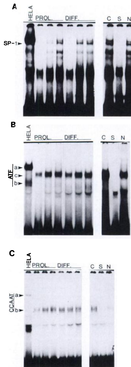
Fig. 8. Gel mobility shift analysis monitoring abundance of general transcription factors in nuclear extracts derived from proliferating (day 2) and differentiated (day 30) ROB cells. In A, the radiolabeled oligonucleotide containing the Sp1 binding site (36) was incubated with increasing amounts of nuclear extracts derived from HeLa S3 cells (HELA, 4 \mu g of protein), proliferating rat osteoblasts (PROL., 3, 6, and 9 \mu g), and differentiated rat osteoblasts (DIFF., 2, 4, and 8 \mu g). The last 3 lanes on the right represent a competition analysis, using 12 \mu g protein from proliferating rat osteoblasts. Reactions were performed in the absence of competitor DNA (C) or in the presence of specific competitor Sp1 (S) or the nonspecific competitor AP-1 (N). Additional sequence-specific complexes observed for this probe may reflect posttranslationally modified forms of Sp1 (e.g., oligomeric, glycosylated, and/or phosphorylated variants) (46). B, ATF binding activity was present in both proliferating (PROL., 0.9, 1.9, and 2.8 \mu g of nuclear extract) and differentiated (DIFF., 1.3, 1.9, and 2.5 \mu g) rat osteoblasts. Lanes C, S, and N, a competition assay in the absence (C) or in the presence (S, specific ATF competitor DNA; N, nonspecific, Sp1 oligonucleotide) of oligonucleotide competitor DNA. Lane HELA, 5 \mu g of HeLa nuclear protein. The probe spans the distal part of H4-site I (spanning nt -154 to -128 in the H4 gene promoter). In C, the CCAAT-binding element present in the H3 histone gene promoter interacts with nuclear proteins derived from HeLa S3 cells (Lane HELA, 2 \mu g), proliferating rat osteoblasts (PROL., 1, 1.9, and 2.9 \mu g), and differentiated rat osteoblasts (DIFF., 1.4, 2.1, and 2.8 \mu g). The last 3 lanes on the right show a competition analysis in the presence of no competitor DNA (C), with CCAAT (S) and ATF (N) as competitors. The probe used in this assay was identical to the fragment used in Fig. 4C.
