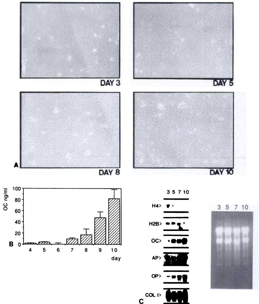
Fig. 1. A , rat osteosarcoma cells (ROS 17/2.8) cultured in vitro during density-induced cell growth inhibition. The photomicrographs were taken at days 3, 5, 8, and 10 after cell plating. B , osteocalcin production per day as determined by radioimmunoassays. The graph shows the increase in osteocalcin secretion into the culturing media when ROS 17/2.8 cells reach confluency. Each point represents the average of 5 samples, which were taken from the media of 5 different plates. C , left , Northern blot analysis of total cellular RNA from ROS 17/2.8 cells during the cessation of proliferation. Blots were analyzed for the representation of mRNAs encoded by cell cycle-dependent and tissue-specific genes. The probes used span mRNA coding sequences of H4, H2B, OC, AP, OP, or type I collagen (coll) and were prepared as reported previously (40, 60). The figure shows that the abundance of cell cycle-dependent histone H4 and H2B mRNAs decreases during density inhibition of rat osteosarcoma cells, whereas the levels for osteocalcin, alkaline phosphatase, and osteopontin increase. On the right , the integrity of mRNA extracted from rat osteosarcoma cells is shown in an ethidium bromide-stained gel. Each lane contains 10 \mu g of total RNA, extracted at, respectively, days 3, 5, 7, and 10.
