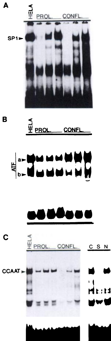
Fig. 4. Analysis of general transcription factor binding activities in nuclear extracts derived from proliferating and density-inhibited rat osteosarcoma cells. A , Sp1 binding activity was assayed in nuclear extracts from proliferating ( PROL. ) and growth-inhibited ( CONFL. ) ROS 17/2.8 cells. The first lane on the left shows Sp1 binding activity present in HeLa nuclear extracts (6 \mu g); Lanes 2–4 from the left, 1.9, 2.9, and 5.8 \mu g of nuclear protein, respectively, from proliferating cells; Lanes 5–7 from the left, 2, 4, and 6 \mu g of nuclear protein, respectively, from growth-inhibited cells. The probe is a consensus Sp1 binding site oligonucleotide (36) similar to the sequence present in the proximal portion of H4-Site I (Fig. 2). In B , total ATF binding activity ( a and b ) was monitored during density inhibition of rat osteosarcoma cells. The first lane from the left contains 2.5 \mu g protein from HeLa cells; Lanes 2–4 from the left, 2.3, 4.5, and 6.8 \mu g protein, respectively, from proliferating ROS 17/2.8 cells; Lanes 5–7 from the left, 3, 4.8, and 6.3 \mu g of protein, respectively, from density-inhibited osteosarcoma cells. The probe spans the ATF binding site present in the distal portion of H4-Site I (nt –154 to –128; DS-1 oligonucleotide) in the H4-FO108 gene promoter. The biological importance of differences in relative band intensities of complexes a and b is not clear. For example, this ratio varied from preparation to preparation with proliferating cells, and we could not discern a consistent pattern. In C , protein/DNA interactions at the CCAAT-box element of the H3 histone gene promoter was analyzed during growth inhibition of osteosarcoma cells. Lane HELA , 7.5 \mu g protein from HeLa nuclei; Lanes 2–4 from the left, 3.9, 7.7, and 11.5 \mu g protein, respectively, from proliferating ROS 17/2.8 cells; Lanes 5–7 from the left, 2.5, 3.8, and 5 \mu g protein, respectively, from density-inhibited ROS. The CCAAT sequence used as probe is derived from the histone H3-ST519 gene promoter (nt –139 to –110) (48). Competition analysis was performed with 5 \mu g protein from HeLa nuclear extracts in the presence of no competitor (Lane C ), the unlabeled CCAAT element oligonucleotide as specific competitor (Lane S ), or the Sp1 fragment as nonspecific competitor (Lane N ).
