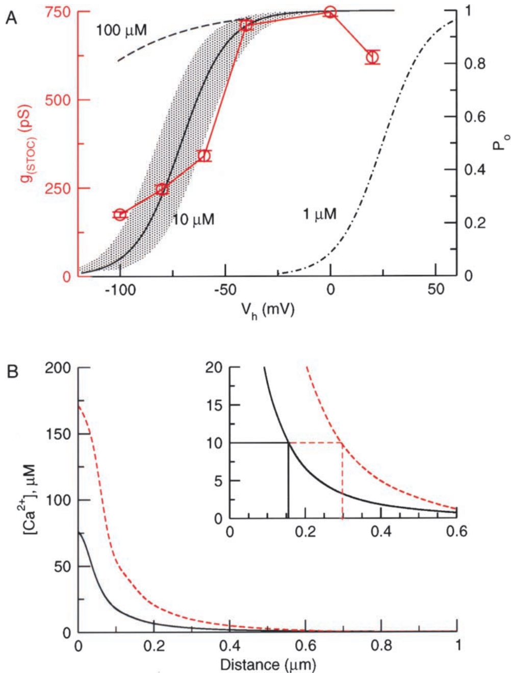
FIGURE 3. (A) Relationship between voltage dependence of g_{(STOC)} and P_o for BK channels. Red curve (continuous line connecting circles) is plot of g_{(STOC)} as a function of holding potential based on the experiments in Fig. 1. Three black lines (dot-dashed, solid, and dashed) were drawn according to published data on P_o of BK channels in excised inside-outside patches exposed to 1, 10, and 100 \mu\text{M} [\text{Ca}^{2+}] in the same cell type (Singer and Walsh, 1987). The shaded area indicates the variation observed at 10 \mu\text{M} . As in the cited publication, the data are fit according to the Boltzmann relationship (Eq. 1). (B) Simulation of [\text{Ca}^{2+}] spatial profile at the end of 15-ms pulses of 1 pA of \text{Ca}^{2+} current from the RyRs during a spark (50 \mu\text{M} fluo-3 plus 27 \mu\text{M} fixed buffer; black solid line) and 3 pA (50 \mu\text{M} fluo-3 plus 230 \mu\text{M} fixed buffer; red dashed line). Inset is the same plot on an expanded scale. The inset provides an indication of the lateral distance from the \text{Ca}^{2+} release site where the [\text{Ca}^{2+}] reaches 10 \mu\text{M} in the two buffer conditions.
