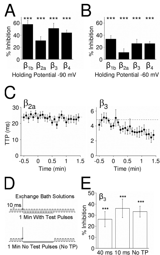
Figure 3. AA inhibition stabilizes closed states of Ca v 1.3b. (A and B) Summary of average percent inhibition of Ca v 1.3b currents after a 1-min exposure to 10 \mu\text{M} AA from a holding potential of -90 mV (A) or -60 mV (B; n = 7-17 ; ***, P < 0.001 compared with CTL currents and P < 0.05 comparing percent inhibition by AA at -90 to -60 mV for all \beta subunits). (C) Time course of averaged TTP for Ca v 1.3b currents with \beta_{2a} (left) or \beta_3 (right) from a holding potential of -60 mV. (D) Protocol for studying AA inhibition in the absence of depolarizing test pulses (TP) from a holding potential of -60 mV. (E) Summary bar graph for percent inhibition by AA: left, with 40-ms test pulses; middle, with 10-ms test pulses; right, with no test pulses ( n = 5-7 ; ***, P < 0.001 compared with CTL currents).
