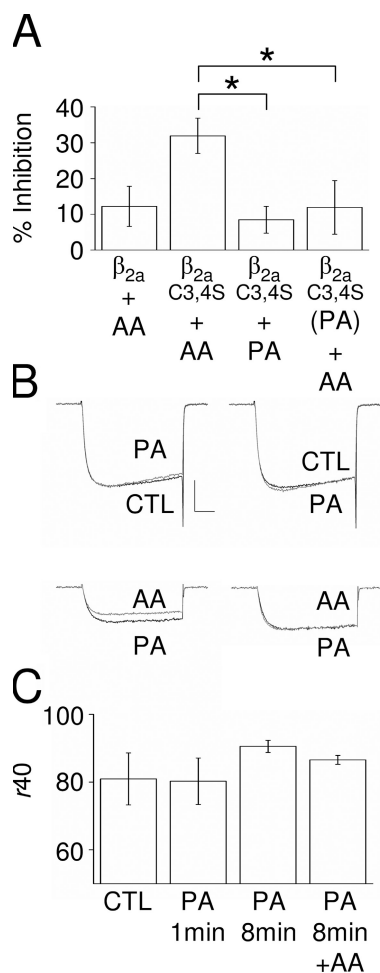
Figure 11. Palmitoylation of \beta_{2a} interferes with AA \text{Ca}_v1.3b inhibition. (A) Summary bar graphs of percent inhibition of \text{Ca}_v1.3b currents with \beta_{2a} , depalmitoylated \beta_{2a} C3,4S (from Fig. 10 A for comparison), \beta_{2a} C3,4S in the presence of 10 \mu\text{M} PA for 1 min, and \beta_{2a} C3,4S preincubated in 10 \mu\text{M} PA for at least 8 min, and then exposed to 10 \mu\text{M} PA + \mu\text{M} AA for 1 min ( n = 3-4 ; *, P < 0.05 compared with \beta_{2a} C3,4S). (B) Representative current traces. (Left, top) \text{Ca}_v1.3b coexpressed with depalmitoylated \beta_{2a} C3,4S before (CTL) and after exposure to 10 \mu\text{M} PA for 1 min. (Left, bottom) \beta_{2a} C3,4S preincubated with 10 \mu\text{M} PA for 8 min (PA), and the addition of 10 \mu\text{M} AA for 1 min (AA). (Right) Normalized to the end of the 40-ms test pulse. (C) Summary bar graphs of current remaining for each condition. Bars, 0.5 nA, 10 ms.
