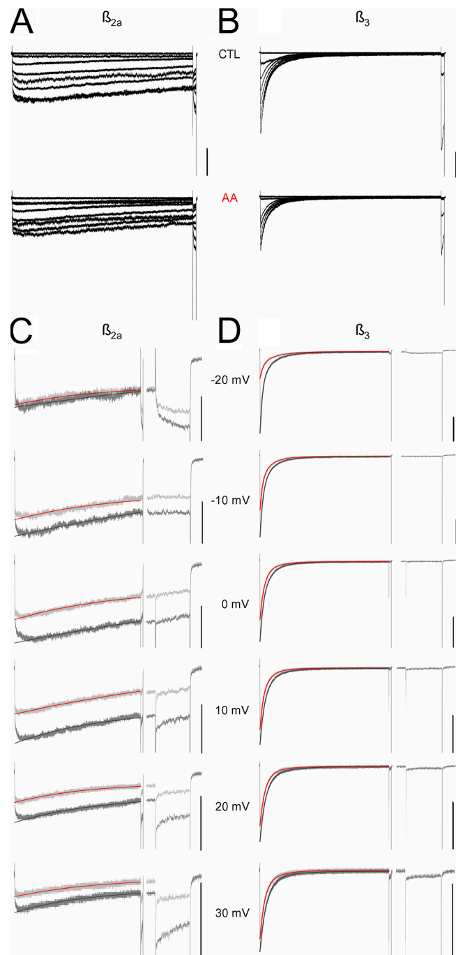
Figure 7. AA does not effect holding potential-dependent inactivation of Ca_v1.3b currents. (A) Representative current traces from Ca_v1.3b , \beta_{2a} channels for CTL conditions (top) or 1 min after a 10 \mu M AA application (bottom) from a holding potential of -60 mV to conditioning pulses from -40 to +30 mV for 2.2 s, and then to a test pulse at -10 mV for 40 ms. Bar, 0.2 nA. (B) Representative current traces from Ca_v1.3b , \beta_3 channels. Conditions are similar to A. Bar, 0.5 nA. (C) Representative current traces from Ca_v1.3b , \beta_{2a} channels for CTL (gray) or inhibited currents 1 min after a 10\text{-}\mu M AA application (light gray) for 2.2-s conditioning pulses from -20 to +30 mV. Fits of inactivation overlay each trace (dark gray, CTL; red, AA). The 40-ms test pulse after the conditioning pulse is expanded on the right. Bar, 0.2 nA. (D) Representative current traces from Ca_v1.3b , \beta_3 channels. Conditions are similar to C. Bar, 0.5 nA.
