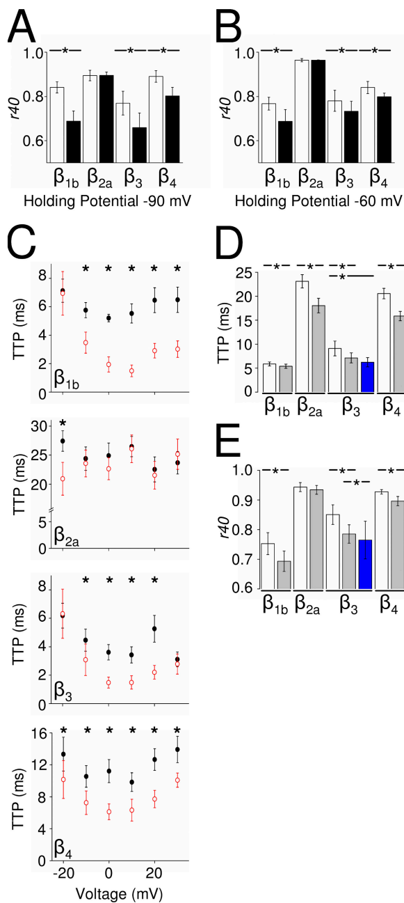
Figure 6. \text{Ca}_V1.3\text{b} kinetic changes by AA are not due to a shift in voltage sensitivity. (A and B) Summary of average current remaining at the end of a 40-ms test pulse ( r_{40} ) for currents before (open bars, CTL) or after a 1-min exposure to 10 \mu\text{M} AA (filled bars) from a holding potential of -90 mV (A) or -60 mV (B; n = 7 – 17 ; *, P < 0.05 ). (C) TTP for CTL (filled circles) or AA (open circles) currents across voltages where channels are activated from a holding potential of -60 mV ( n = 7 – 13 ; *, P < 0.05 ). (D) Summary of TTP changes produced by 30 \mu\text{M} ETYA (open bars, CTL before ETYA; gray bars, 1 min after ETYA; blue bar, 1 min after 30 \mu\text{M} ETYA + 10 \mu\text{M} AA for \beta_3 ; n = 4 – 8 ; *, P < 0.05 ). (E) Summary of r_{40} changes produced by ETYA. Bar descriptions are the same as in D.
