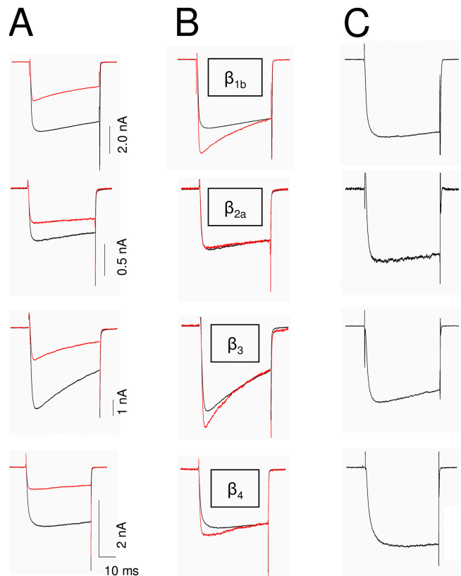
Figure 2. \text{Ca}_v1.3b current inhibition and kinetic changes by AA are \text{Ca}_v\beta subunit dependent. (A) Representative current traces from \text{Ca}_v1.3b channels coexpressed with \beta_{1b} , \beta_{2a} , \beta_3 , or \beta_4 before (CTL; black line) or 1 min after AA (10 \mu\text{M} ; red line) application highlight the smaller amount of inhibition with \beta_{2a} . (B) Current traces from A were normalized to the end of the test pulse to highlight kinetic changes produced by AA for \beta_{1b} , \beta_3 , and \beta_4 , but not \beta_{2a} -containing channels. (C) Inhibited currents were averaged and subtracted from averaged CTL currents to obtain a difference current for \text{Ca}_v1.3b with each \text{Ca}_v\beta subunit to determine the shape of the current lost after AA application ( n = 7-13 ).
