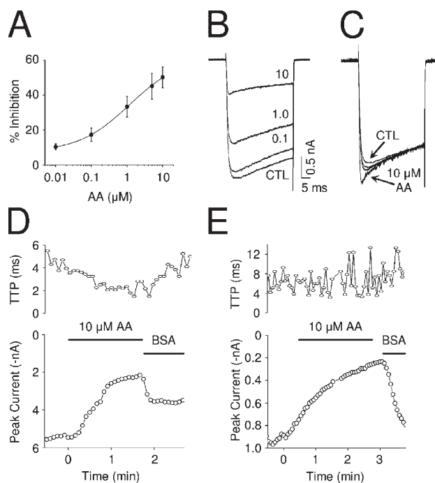
Figure 1. AA modulates amplitude and kinetics of whole cell Ca_v1.3b currents. (A) Concentration–response curve of AA on Ca_v1.3b , \beta_3 currents. Concentrations of 0.01, 0.1, 1, 5, and 10 \mu M were bath applied, and current inhibition was measured after 1 min ( n = 3–11 ). (B) Individual traces of Ca_v1.3b , \beta_3 currents before (CTL) and after the application of 0.1, 1, or 10 \mu M AA. (C) Individual traces from B were normalized, revealing that exposure to 10 \mu M AA decreases the TTP. (D) TTP and current amplitude for Ca_v1.3b , \beta_3 currents plotted versus time. Bars indicate where 10 \mu M AA and 1 mg/ml BSA were added. Both changes reverse after wash with BSA. (E) TTP and current amplitude for Ca_v1.3b , \beta_{2a} currents plotted versus time. Conditions are the same as in D. No TTP change is observed. AA still inhibits current over time that reversed by washing with BSA.
