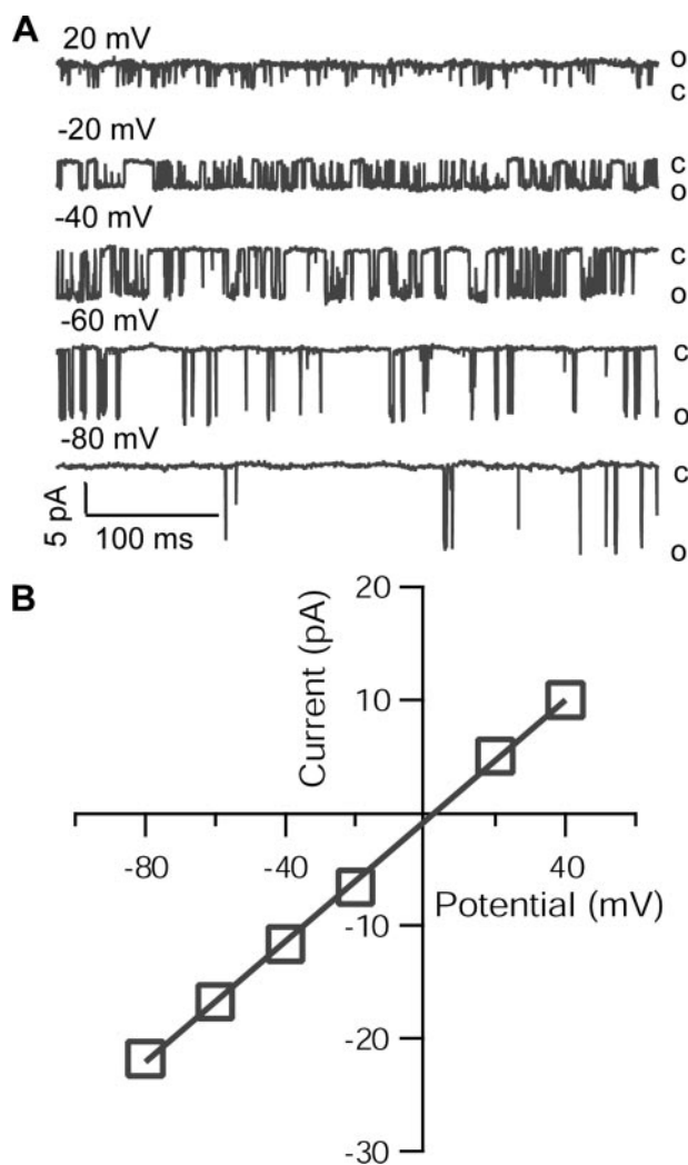
FIGURE 2. Voltage dependence of BK Ca channels expressed in HEK-293 cells. A , currents through a single channel recorded in inside-out patch clamp mode in the presence of 1 \mu M free Ca 2+ , shows an increase in activity with depolarization from a holding potential of -80 to +20 mV. B , an I-V plot (channel current versus membrane potential) averaged over 10 recordings yielded a BK Ca channel unitary conductance of 267 pS. O and C represent the open and closed states of the channel, respectively.
