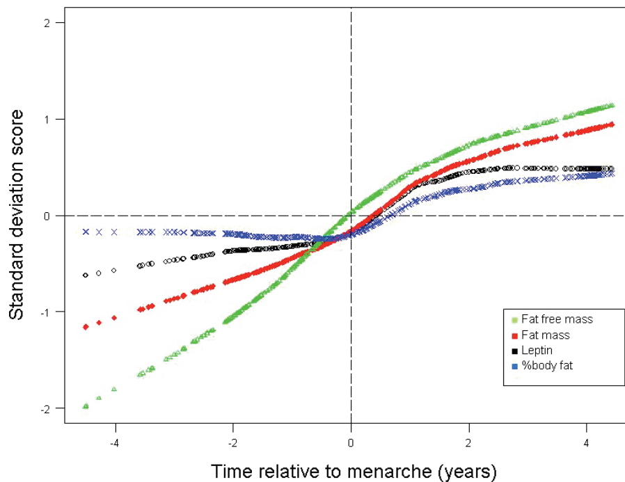
Figure 1 Body composition changes and serum leptin levels relative to menarche. Standard deviation score transformations were applied based on FFM (mean = 36.44, SD = 6.38 kg), Fat (mean = 12.95, SD = 4.20 kg), leptin (mean = 9.48, SD = 5.86 ng/mL) and %BF (mean = 25.75, SD = 4.46).
