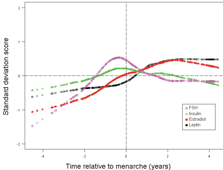
Figure 2 Change in serum hormone levels relative to menarche in years. Standard deviation score transformations were applied based on FSH (mean = 3.11, SD = 1.64 mIU/mL), insulin (mean = 13.17, SD = 6.51 \mu U/mL), estradiol (mean = 46.12, SD = 36.41 pg/mL) and leptin (mean = 9.48, SD = 5.86 ng/mL).
