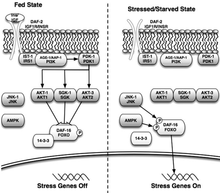
FIG. 6. Insulin/IGF signaling cascade in two different states. In a fed state, under high insulin/IGF-1 signaling, DAF-16 is located in the cytosol, whereas under stress or starvation, DAF-16 is located in the nucleus.
