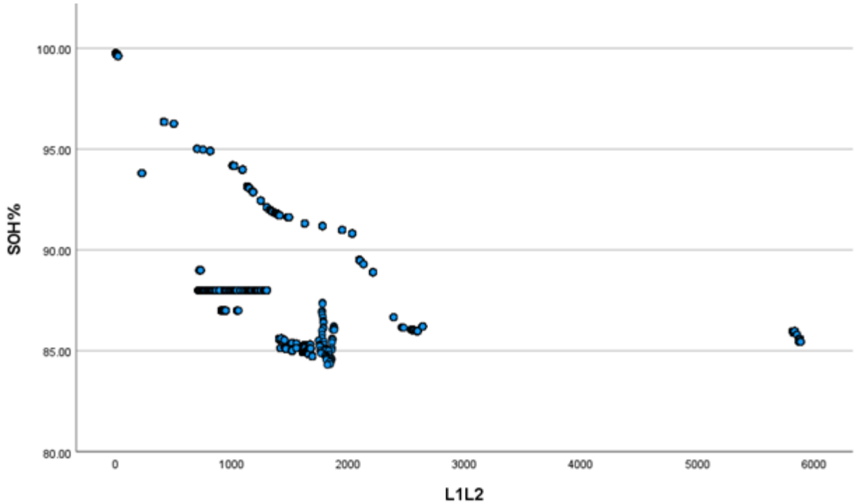
Figure 17. Scatterplot of SOH by L1/L2 for Nissan Leafs
