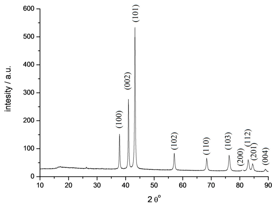
Figure 9. Diffractogram of technetium powder obtained by thermal decomposition of [\text{Me}_4\text{N}^+]\text{TcO}_4^- (fragment). \text{Cu K}\alpha radiation.
