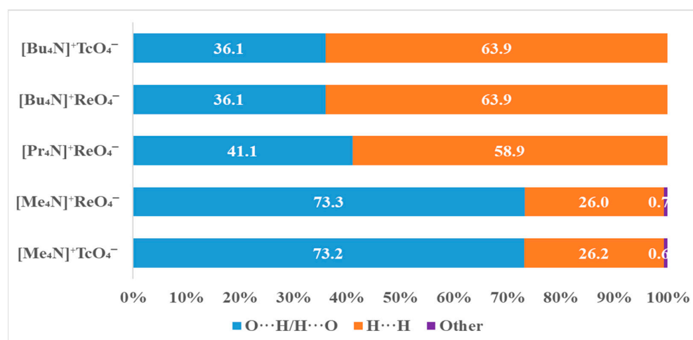
Figure 3. Percentage contributions of contacts to the Hirshfeld surface in the structures [\text{Me}_4\text{N}]^+\text{TcO}_4^- , [\text{Me}_4\text{N}]^+\text{ReO}_4^- , [\text{Pr}_4\text{N}]^+\text{ReO}_4^- , [\text{Bu}_4\text{N}]^+\text{ReO}_4^- and [\text{Bu}_4\text{N}]^+\text{TcO}_4^- .
