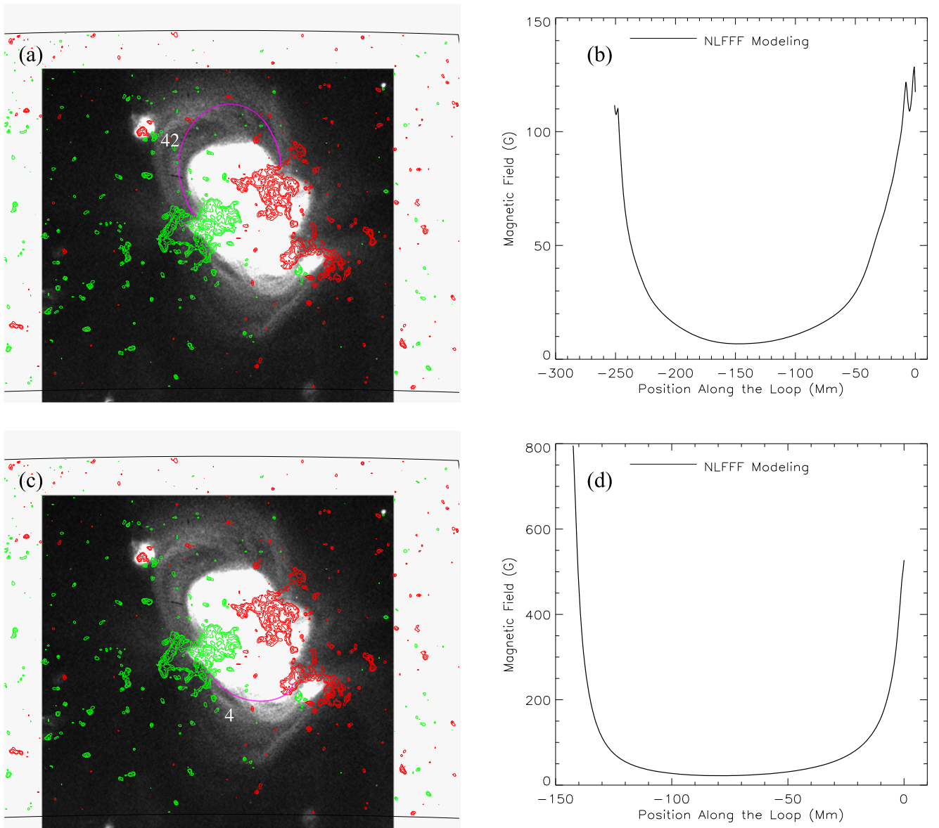
Figure 5. (a) XRT observation of active region NOAA 10938 on 2007 January 18 at 19:19:42 UT with a fitted field line, numbered 42, to the observed cloud. (b) The magnetic field variation as a function of position for field line 42. (c) The magnetic field line numbered 48 in the same active region. (d) Magnetic field variation as a function of position for field line 48.
