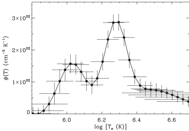
Figure 11. DEM at the coordinates (1001'', -90''/5). The bimodal form of the DEM is typical throughout the observed field of view.
