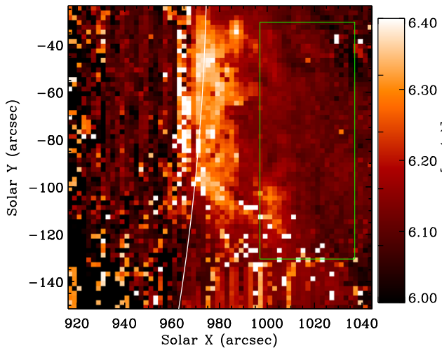
Figure 12. Map of T_e within the field of view in the 2'' binned data.
