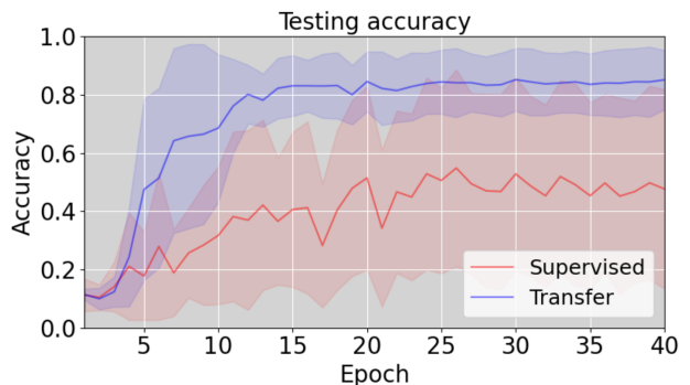
Figure 3: Comparison between supervised and transfer learning during the testing phase.
