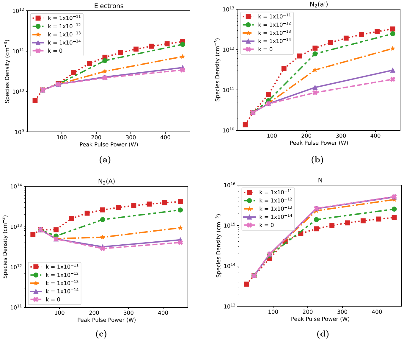
Figure 14. Average densities of electrons (a), \text{N}_2(a') (b), \text{N}_2(A) (c) and atomic nitrogen (d) in the equilibrium phase of the simulation, for different values of k_{51/52} . The average density is calculated over the time period 90–96 ms. The pulse repetition frequency and pulse width are 1 kHz and 10 \mu\text{s} , respectively.
