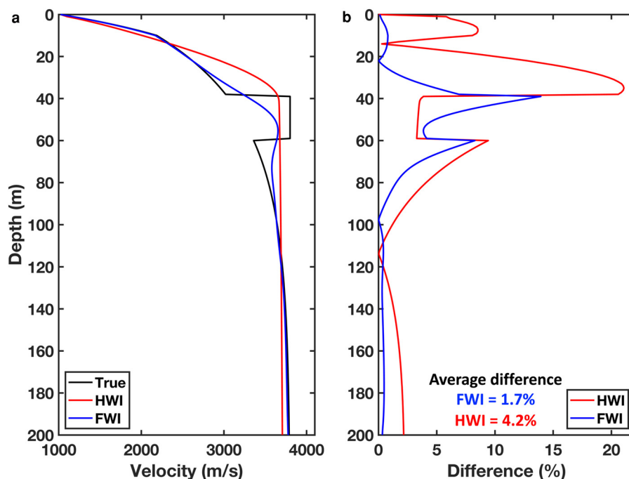
Fig. 1. (a) Velocity model outputs from HWI (Red) and FWI (Blue) compared to the True model (Black). The HWI generates a velocity profile that stops increasing in velocity at the depth of the ice slab top (40 m). This velocity is then extrapolated to the base of the model. FWI produces a velocity increase at 30 m depth and a decrease at 70 m depth, indicating the ice slab’s location. (b) The absolute percentage error between the inversion models for HWI (Red) and (FWI) relative to the True model. The average difference for the total depth shows FWI reduces the error by 2.5%. A maximum difference of 20% for the HWI velocity model is observed in the top 40 m.
