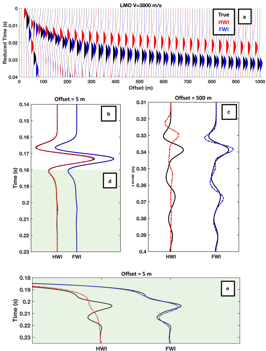
Fig. 2. Seismic data forward modelled from the True (Black), HWI (Red) and FWI (Blue). (a) All data with LMO applied with a velocity of 3800 \text{ m s}^{-1} . (b) Comparison of trace from an offset of 5 m, the first arrival is modelled well by both the HWI and FWI, the green panel indicates the zoomed in section of figure (d). (c) Comparison of trace from an offset of 500 m. FWI closely reproduces the true data, while HWI poorly represents the true data. (d) Zoom of the reflection at 5 m offset produced by the ice slab visible at near offsets.
