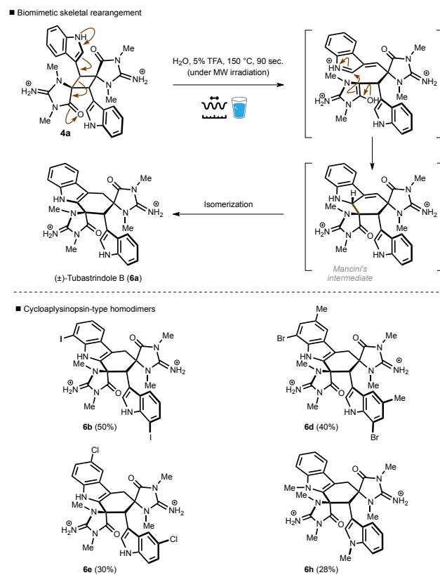
Figure 4. Ring expansion of dictazole-type structures.
