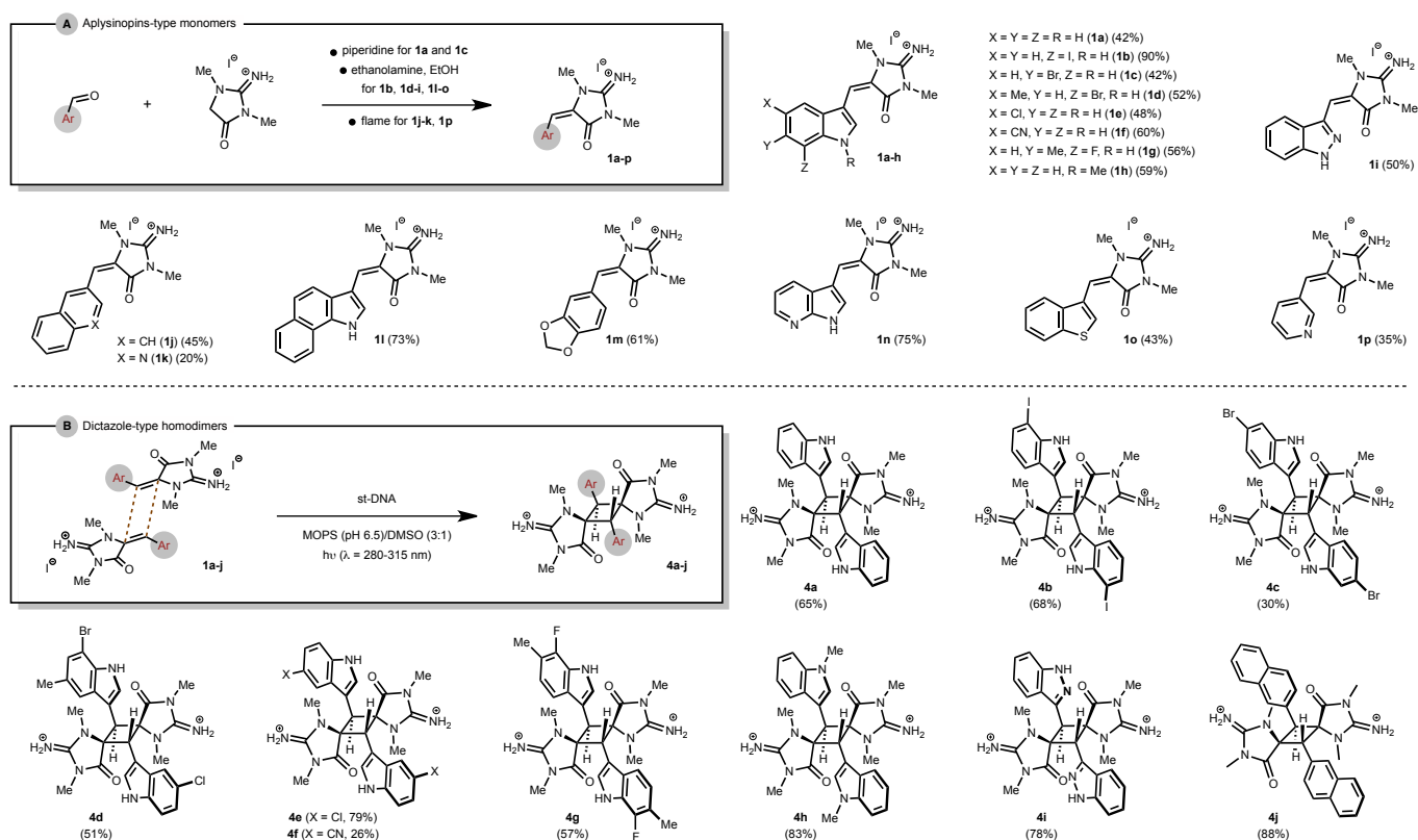
Figure 2. ( E )-Aplysinopsin- and dictazole-type products synthesized.
