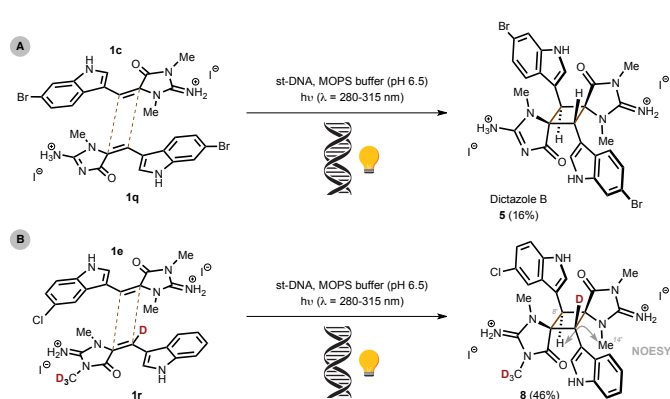
Figure 3. (A) Synthesis of dictazole B (5). (B) Cycloaddition of 5-chloro-( E )-aplysinsopin (1e) and deuterated-( E )-aplysinsopin (1r).
