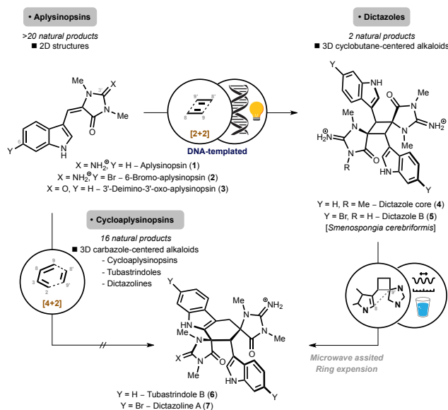
Figure 1. The 'aplysinopsin cascade' via a DNA-templated [2+2] cycloaddition.
