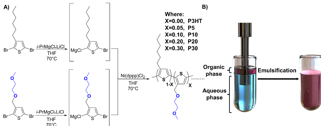
Figure 1: A) Schematic representation of the random copolymer synthesis. B) Representation of the ultrasonication process to generate the corresponding surfactant-free polymer dispersion.
