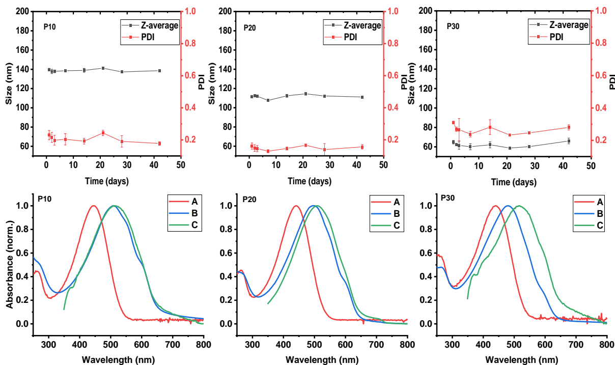
Figure 2: (Top) Analysis of particle stability over time via DLS measurements from P10 (left), P20 (centre), and P30 (right) dispersions in water. (Bottom) UV-vis spectra of A) polymer solutions in chloroform, B) polymer dispersions in water and C) thin films spin-cast from chloroform solutions, for P10 (left), P20 (centre), and P30 (right).
