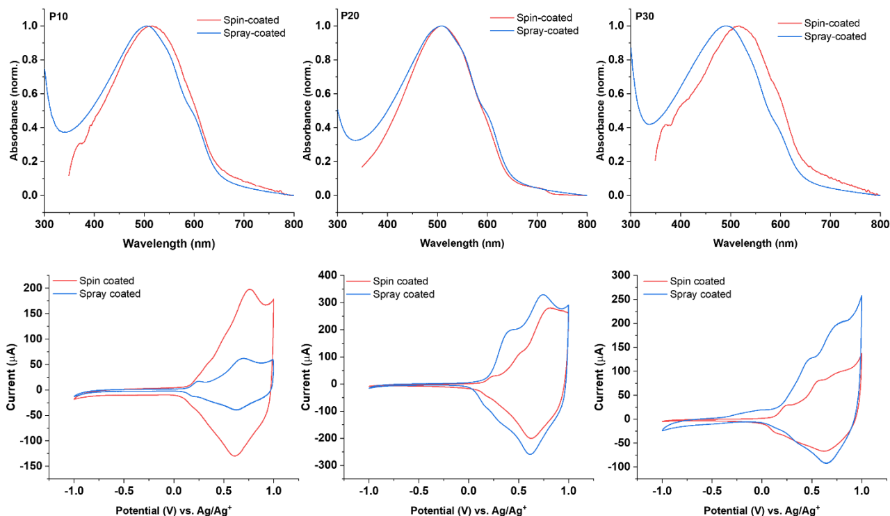
Figure 3: (Top) Solid state UV-vis spectroscopy of thin films deposited via spin-coating from organic solutions in chloroform (5 mg/mL) and via spray-coating from polymer dispersions (1 mg/mL). Cyclic voltammograms for thin films deposited onto indium tin oxide (ITO) coated glass via spin-coating from organic solutions in chloroform (5 mg/mL) and via spray-coating from polymer dispersions (1 mg/mL) in 0.1 M solution of tetrabutylammonium hexafluorophosphate in acetonitrile at a scan rate of 100 mV/s, plots correspond to the second scan of each measurement of P10 (left), P20 (centre), and P30 (right).
