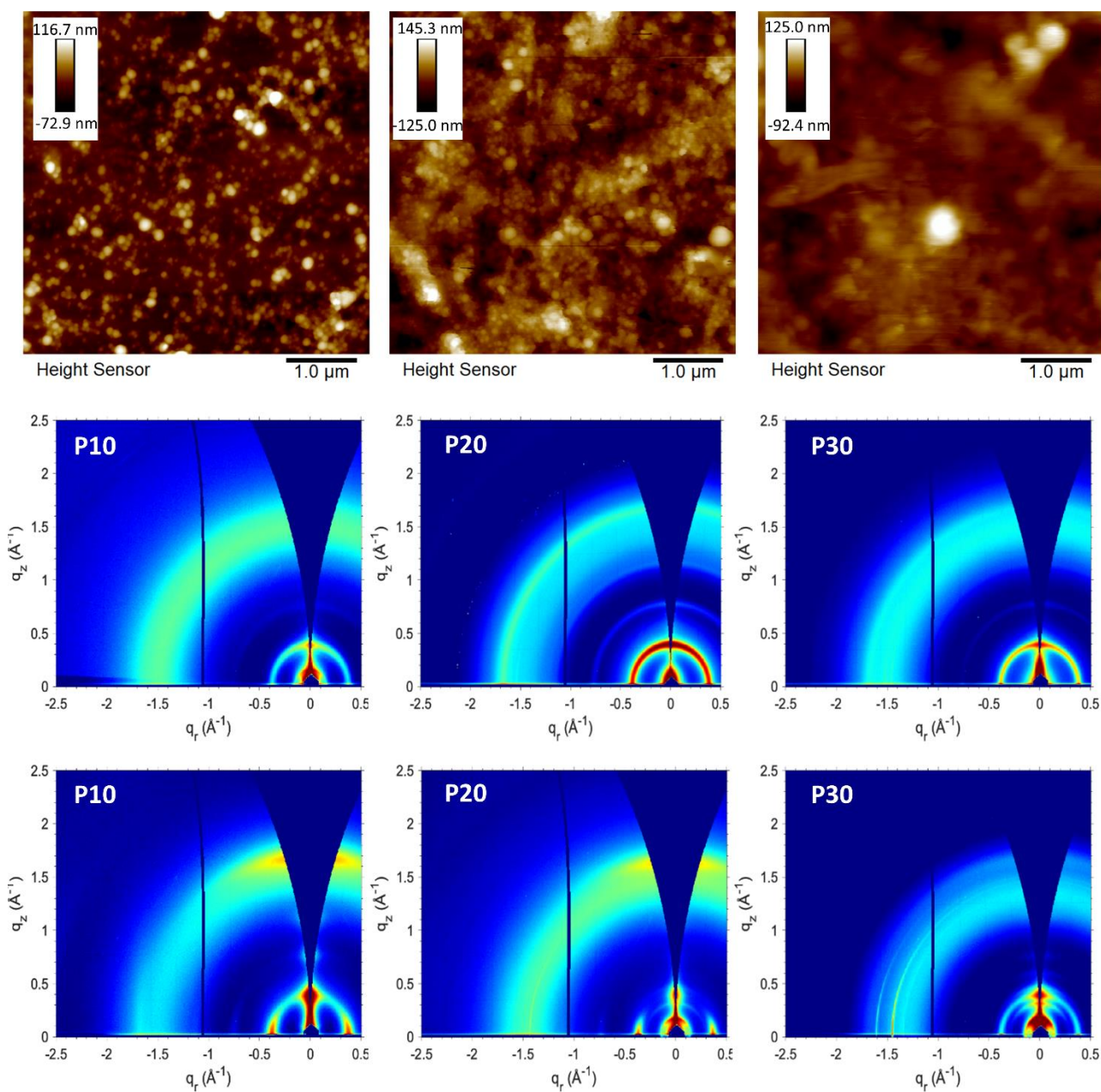
Figure 4: (Top) Atomic force micrographs of the polymer dispersions deposited via spray-coating onto glass substrates at 65 °C; P10 (left), P20 (centre), and P30 (right). Scale bars (insets) are in nm units. (Middle) 2D GIWAXS patterns of the polymer films deposited onto silicon substrates from aqueous dispersions via spray-coating at 90 °C. (Bottom) 2D GIWAXS patterns of the polymer films deposited onto silicon substrates from chloroform solutions via spin-coating.
