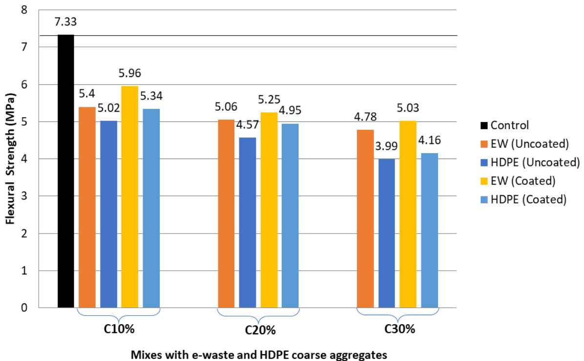
Figure 19. Comparison of flexural strength values of concrete mixes with control sample and concrete containing uncoated and coated recycled plastic.
