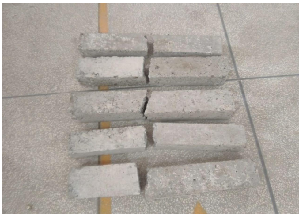
Figure 18. Failure mode of concrete beams with recycled plastics after flexural strength test.
