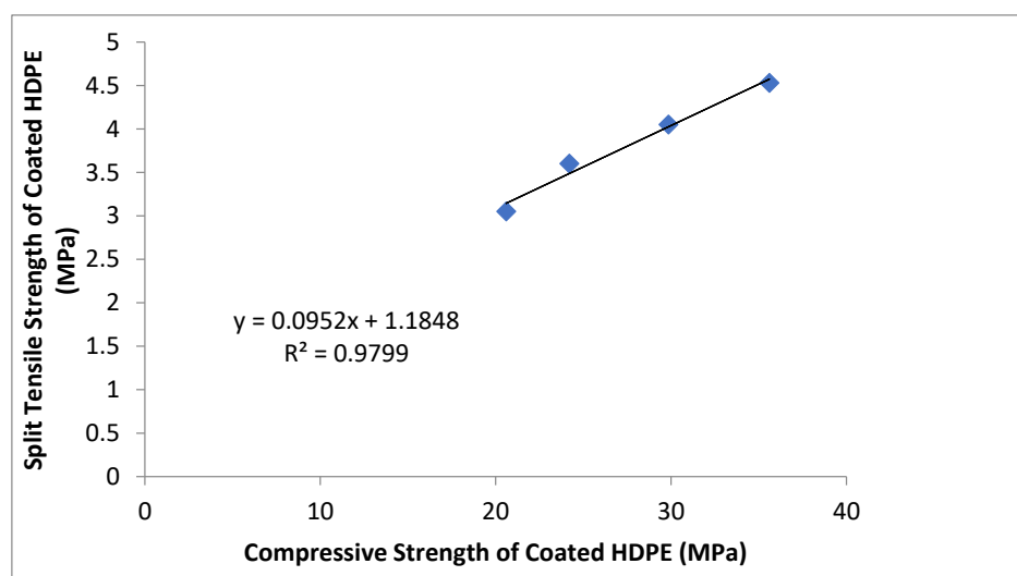
Figure 24. Correlation of compressive strength and split tensile strength of concrete with sand coated HDPE.
