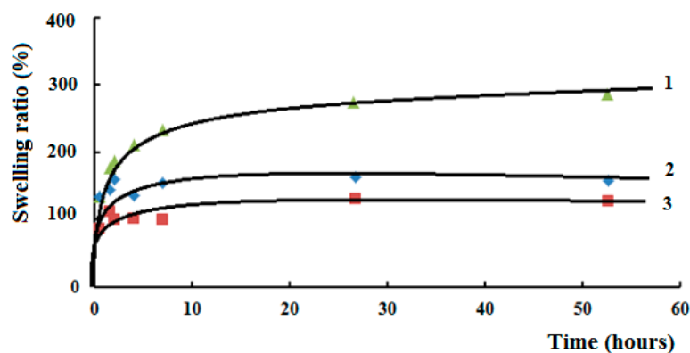
Figure 9. Swelling kinetics of chitosan hydrochloride/citrus pectin hydrogels in 0.9% solution of AlCl 3 (1), CaCl 2 (2), NaCl (3). Data are expressed as mean ± SD; n = 3.
