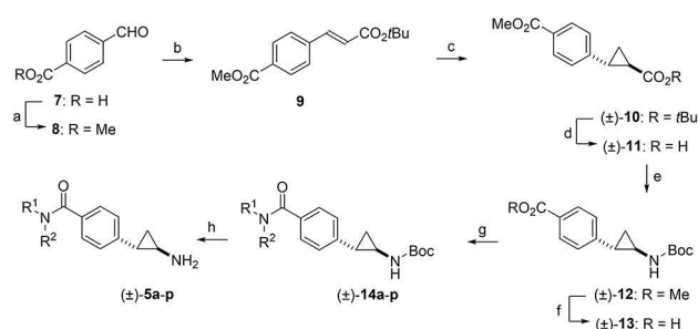
Scheme 1. Synthesis of tranylcypromine analogues 5a–p . a) AcCl, MeOH, 0 °C to RT, overnight, 91 %; b) tert -butyl diethylphosphonoacetate, KOtBu, THF, –5 °C to RT, overnight, 98 %; c) Me 2 S(O) + I – , KOtBu, DMSO, RT, overnight, 53 %; d) TFA, Et 3 SiH, CH 2 Cl 2 , RT, overnight, 72 %; e) diphenylphosphoryl azide, Et 3 N, t BuOH, reflux, 72 h, 42 %; f) LiOH, aq THF, 50 °C, 2 h, 82 %; g) R 1 R 2 NH, EDCl, HOBT, i Pr 2 NEt, RT, overnight, 36–67 %; h) HCl, THF, 13–71 %.
