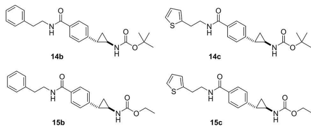
Figure 6. Structures of tranylcypromine carbamates 14b,c and 15b,c .
