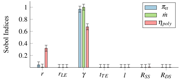
Figure 9 Sobol indices after applying the HPT-metamodel.
