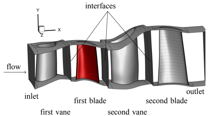
Figure 5 HPT simulation setup with studied first rotor blade highlighted in red.
