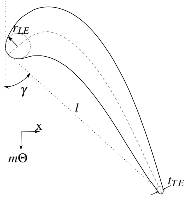
Figure 3 Blade section of deteriorated blade at mid-span.
