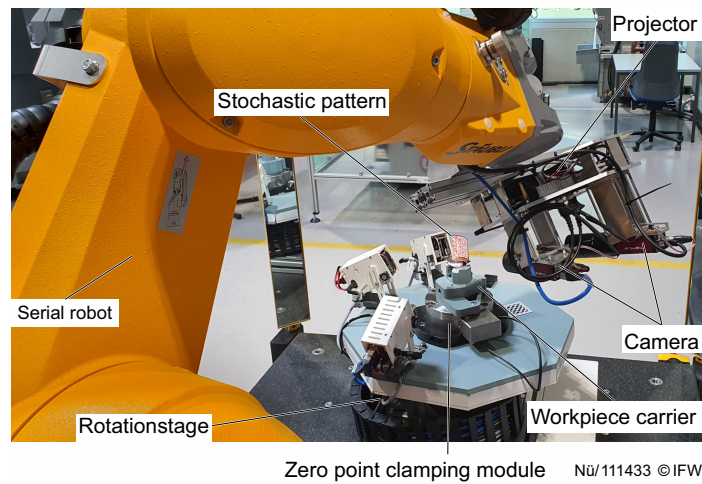
Figure 2 Measurement system scanning a blade.
