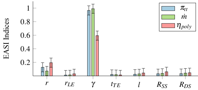
Figure 8 EASI indices for CFD data.
