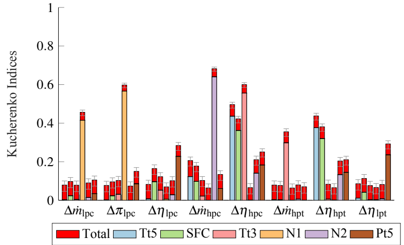
Figure 10 First and Total Kucherenko Indices of the scaling factors and overall performance output.
