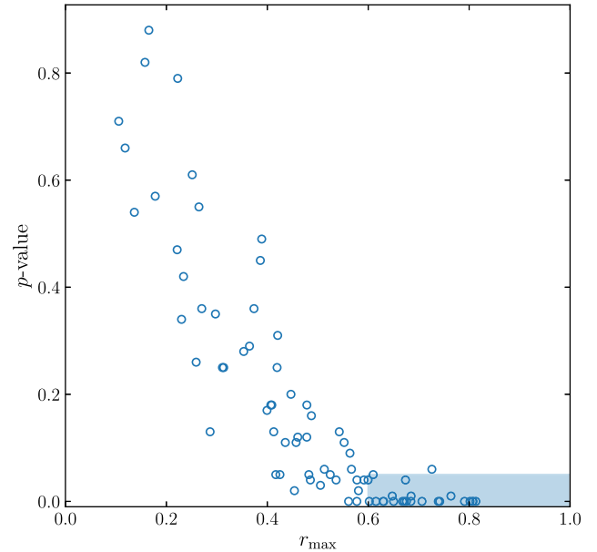
Figure 3. p -value versus r_{\text{max}} for our 78 AGN. The r_{\text{max}} is of the original pair of light curves. The shaded region indicates our selection criteria requiring a p -value < 0.05 and r_{\text{max}} > 0.6 .
