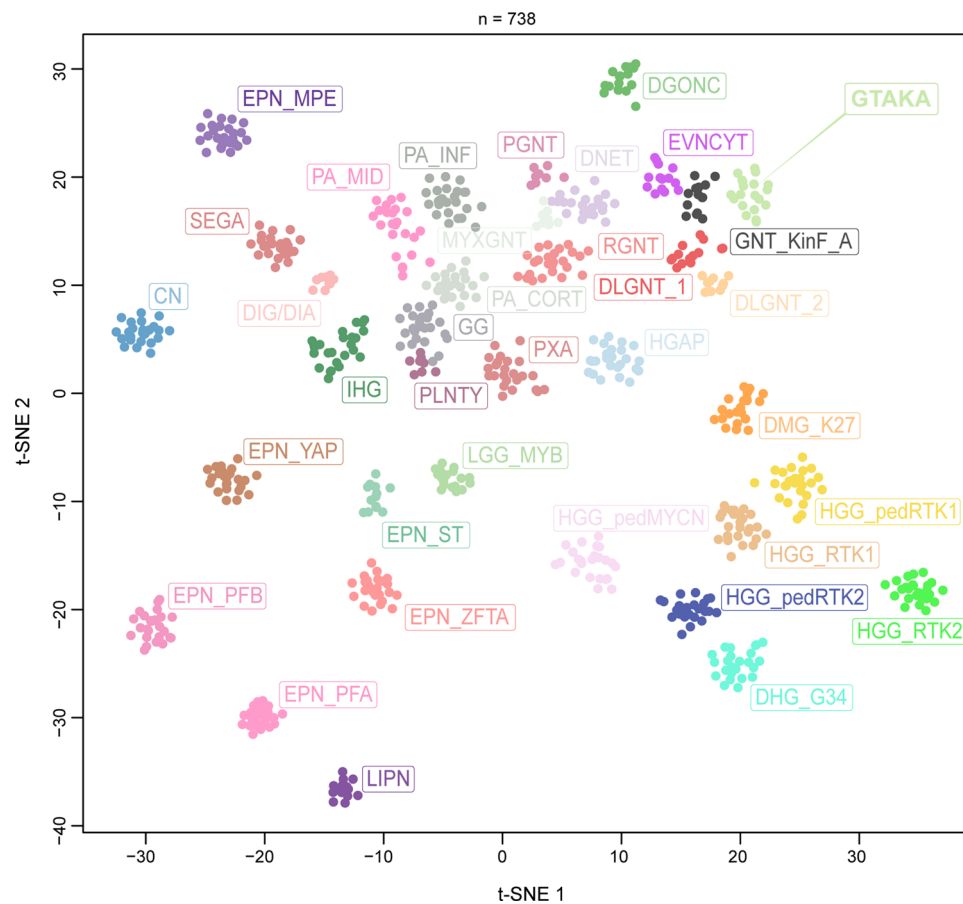
Fig.1 Unsupervised, non-linear t-distributed stochastic neighbor embedding (t-SNE) projection of DNA methylation array profiles from 738 tumor samples. DNA methylation profiling reveals a molecular distinct group of glioneuronal tumors (GTAKA). Reference DNA methylation classes: dysembryoplastic neuroepithelial tumor (DNET), rosette-forming glioneuronal tumor (RGNT), diffuse leptomenigeal glioneuronal tumor subtype 1 (DLGNT_1), diffuse leptomenigeal glioneuronal tumor subtype 2 (DLGNT_2), extraventricular neurocytoma (EVNCYT), papillary glioneuronal tumor (PGNT), ganglioglioma (GG), polymorphous low-grade neuroepithelial tumor of the young (PLNTY), myxoid glioneuronal tumor, PDG-FRA-mutant (MYXGNT), diffuse glioneuronal tumor with oligodendroglioma-like features and nuclear clusters (DGONC), glioneuronal tumor kinase-fused (GNT_KinF_A), central neurocytoma (CN), cerebellar liponeurocytoma (LIPN), desmoplastic infantile ganglioglioma / desmoplastic infantile astrocytoma (DIG/DIA), angiocentric glioma MYB/MYBL1-altered (LGG_MYB), pilocytic astrocytoma hemi-
