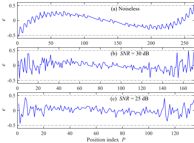
Fig. 15. Simulated tag location detection error: (a) noiseless antenna with N = 265 , (b) \text{SNR} = 30 dB with N = 171 , (c) \text{SNR} = 25 dB with N = 135 .
