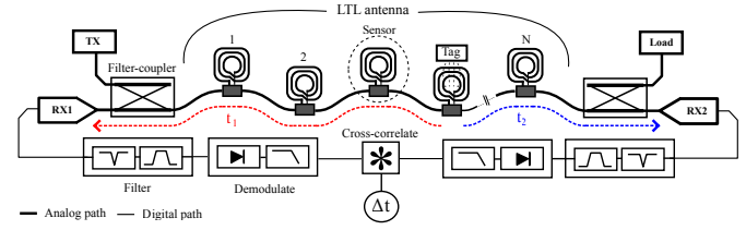
Fig. 9. Block diagram for NFC system capable of tag localization along LTL antenna.
