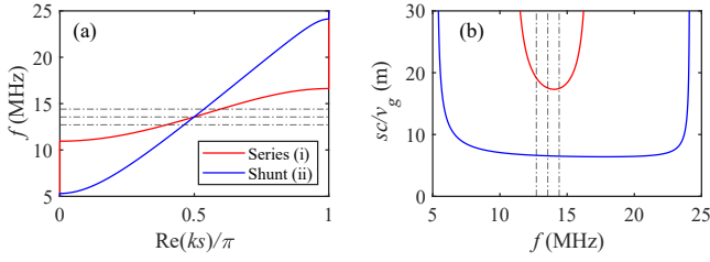
Fig. 4. Dispersion relation and slow wave factor for LTL waveguide loaded with impedances (i) and (ii) in series and shunt configurations respectively for L = 2 \mu\text{H} , C = 68.9 \text{ pF} , and d = 4 \text{ m} . Dashed lines show the frequency locations of HF carrier and tag response sidebands.
