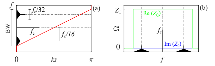
Fig. 2. (a) Dispersion curve and (b) characteristic impedance (green and blue) of an idealized LTL antenna for transponder tracking and communication. The passband covers the communication bandwidth of ISO 14443 Type A protocol. The group velocity is constant and minimized. The characteristic impedance is real and constant across the passband.
