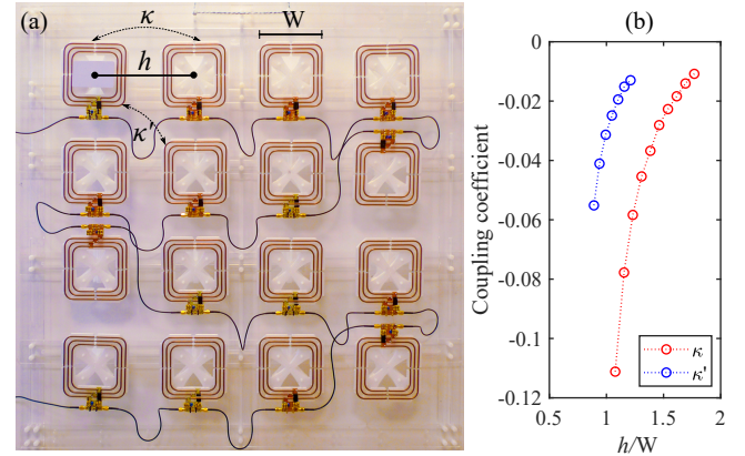
Fig. 12. (a) Photograph of a quasi 2D LTL antenna (b) Measured magnetic coupling coefficient between nearest neighbours, \kappa for adjacent elements (red) separated by h/W , and \kappa' for diagonally adjacent elements (blue).
