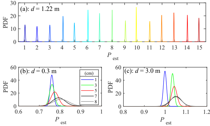
Fig. 11. Probability density functions fitted to experimental position data using sample size of 100 for each distribution. (a) Tag at 0 cm separation for all 15 sensors with d = 1.22 m; (b) tag at varying separation distances at position 1 with d = 0.3 m; (c) tag at varying separation distances at position 1 with d = 3.0 m. The tag could be located correctly for all measurements.
