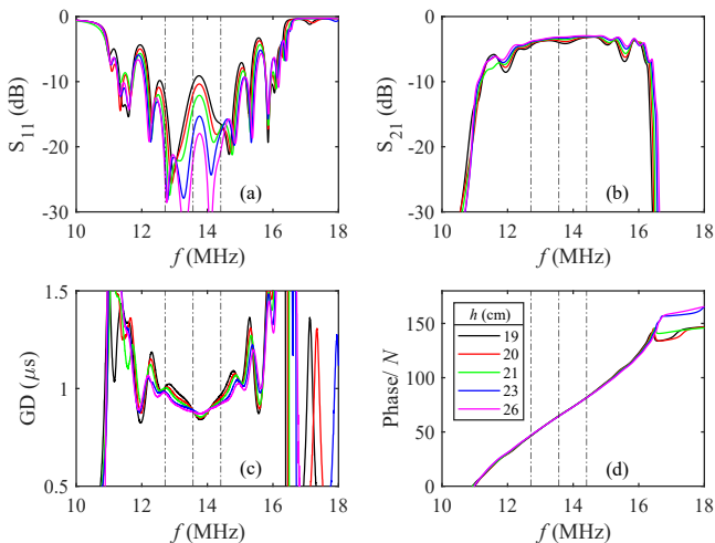
Fig. 13. Measured scattering parameters of quasi-2D grid for a range of neighbour separation distances h . (a) S_{11} parameters; (b) S_{21} parameters; (c) group delay; (d) phase shift per element in degrees.
