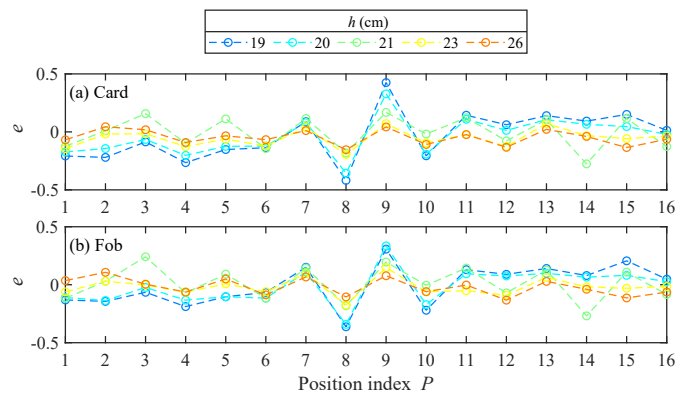
Fig. 14. Experimental variation of location error e with tag position index P over a range of neighbour separation distances h for a card-type (a) and fob-type tag (b).
