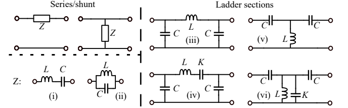
Fig. 3. Sensor network candidates that include series/shunt impedances (i-ii), pi-sections (iii-iv), or t-sections (v-vi).
