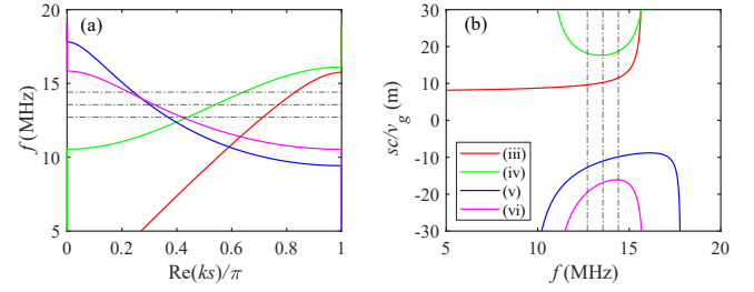
Fig. 5. (a) Dispersion curves and (b) slow wave factors for LTL antennas with d = 2 \text{ m} loaded with sections (iii–vi). For (iii) L = 0.59 \mu\text{H} , C = 250 \text{ pF} ; (iv) L = 2 \mu\text{H} , C = 115 \text{ pF} , K = 89.7 \text{ pF} ; (v) L = 0.59 \mu\text{H} , C = 200 \text{ pF} ; (vi) L = 0.37 \mu\text{H} , C = 190 \text{ pF} , K = 143 \text{ pF} . Topology (iv) offers the best match to the ideal requirements of Fig. 2(a).
