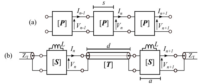
Fig. 1. Schematic presentation of (a) classical periodic cascade of two-port networks, each having a transfer matrix \mathbf{P} and (b) loaded transmission line (LTL) formed by a periodic cascade of coaxial cable sections and generic two-port networks having transmission matrices \mathbf{T} and \mathbf{S} , respectively.
