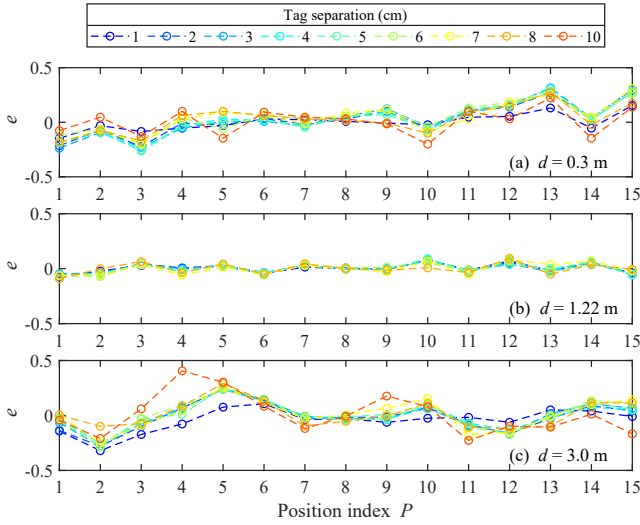
Fig. 10. Experimental variation of localization error e with tag position index P over a range of sensor-tag separation distances. (a) d = 0.3 m; (b) d = 1.22 m; (c) d = 3 m.
