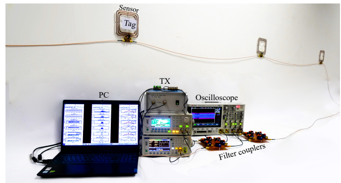
Fig. 7. Photograph of the complete NFC system including an LTL antenna and a custom reader.
