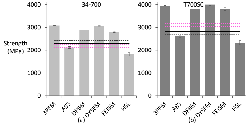
Figure 8: Predicted and measured strength values: (a) for 34-700 composites and (b) for T700SC composites.
