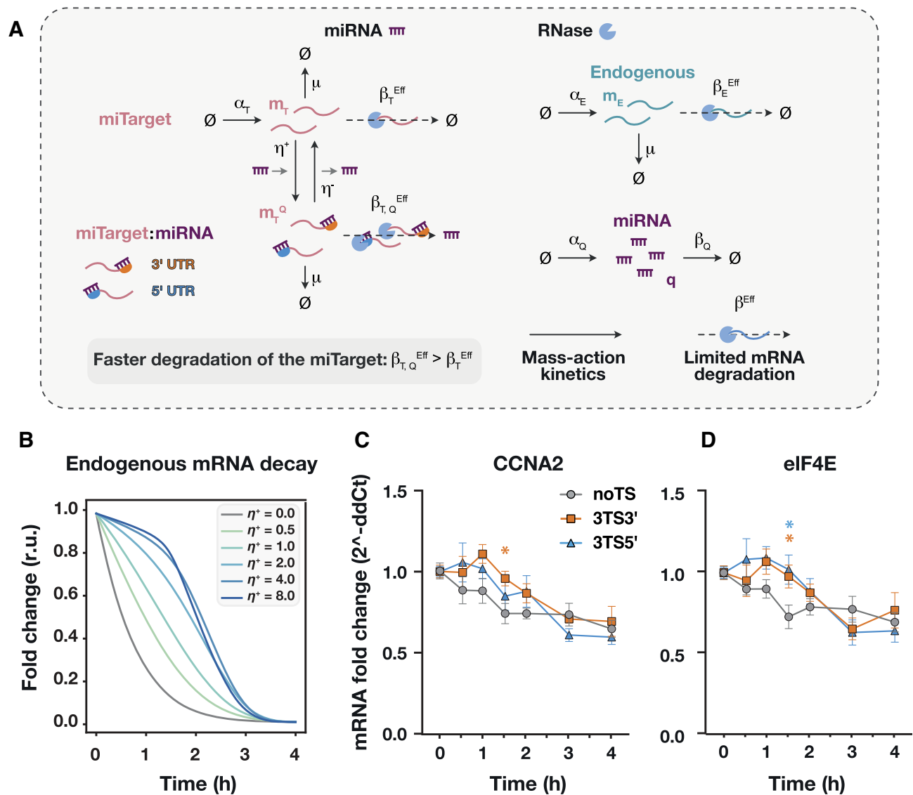
Figure 4. miRNA action increases non-target transcripts' half-life. (A) Graphical representation of the resource-aware model used to study the reallocation of the degradation resources (RNases). The model described in Figure 2 is extended to include a finite pool of RNases. The competition for the shared pool of RNases is captured via the effective mRNA degradation rate constants \beta_T^{Eff} and \beta_{T,Q}^{Eff} (miTarget), and \beta_E^{Eff} (endogenous gene). The miRNA-driven decay increases the rate of binding between the miTarget transcript and the degrading resources by increasing the association constant \beta_T^+ to the new value \beta_{T,Q}^+ . A description of the model can be found in Supplementary Note 5. All the molecular species captured in the model are listed in Supplementary Table 6, whilst all the model parameters—including the numerical values used for the simulations—are summarised in Supplementary Table 7. (B) Predicted mRNA degradation profiles of an endogenous gene upon halting of transcription for different values of the miRNA binding constant \eta^+ . Reallocation of degrading resources alters the endogenous mRNA degradation profile and depends on the miRNA binding constant. The mRNA degradation profiles were normalised to the initial data point. Each colour represents a different value for the miRNA binding constant \eta^+ . r.u.: relative units. (C, D) mRNA half-life and degradation dynamics measurement of CCNA2 (C) and eIF4E (D) upon DRB treatment (50 \mu M). All data were acquired 24 hours post transfection and are plotted as mean \pm SE. SE: standard error. N = 4-8 biological replicates. An unpaired two-sided t -test was used to compare 3TS3' and 3TS5' samples to the noTS control. P -value: * < 0.05 .
