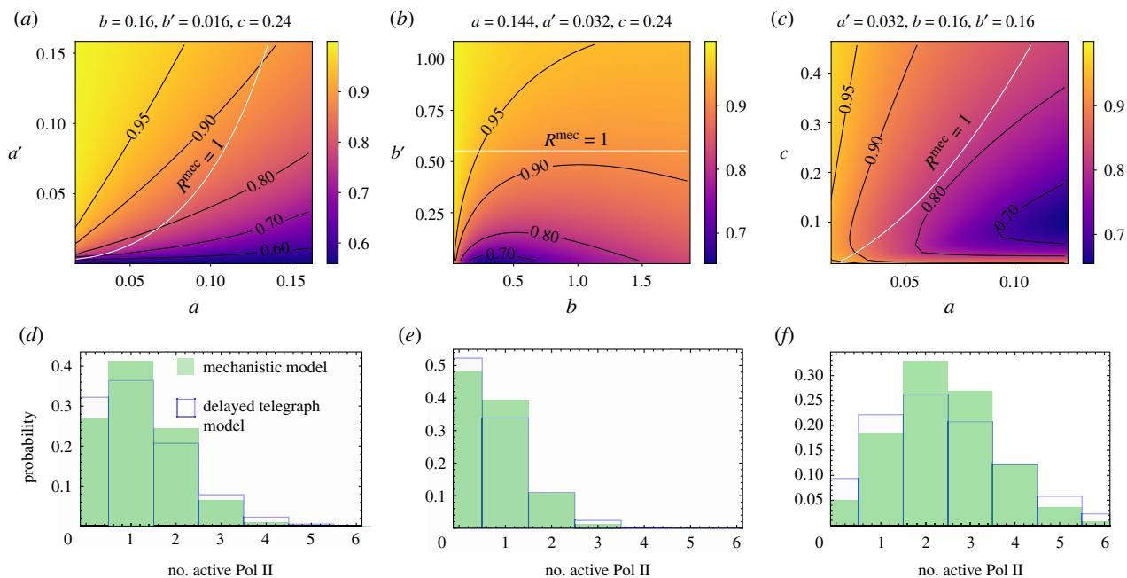
Figure 6. Accuracy of the number distributions of active Pol II constructed using the delay telegraph model for parameters close to the boundary R^{\text{mec}} = 1 . (a–c) The minimum Fano factor of active Pol II numbers in the mechanistic model as a function of the parameters \theta^{\text{mec}} = \{a, a', b, b', c\} . For a given set of \theta^{\text{mec}} , the minimum Fano factor is found by varying the elongation time \tau in equation (5.3). The region above the white line R^{\text{mec}} = 1 is where model reduction using waiting time statistics is possible. Note that inside this region, the minimum Fano factor of active Pol II numbers is smaller than 1, meaning that for small enough values of \tau , model reduction using number statistics is not possible. However, in (d–f) we show that even when this is the case, the number distributions constructed using the delay telegraph model with effective parameters given by equations (3.4) provide a reasonably good approximation to the mechanistic model distribution of active Pol II. Note that these distributions represent a worst case scenario—inside the boundary, for the vast majority of points, the two-state model distributions provide an almost perfect fit to the mechanistic model distributions as shown in figure 2. The parameters are as follows: (d) a = 0.0336 \text{ s}^{-1} , a' = 0.006 \text{ s}^{-1} , b = 0.16 \text{ s}^{-1} , b' = 0.016 \text{ s}^{-1} , c = 0.24 \text{ s}^{-1} , \tau = 13.65 \text{ s} , FF_A^{\text{mec}} = 0.74 , R^{\text{mec}} = 1.034 ; (e) a = 0.072 \text{ s}^{-1} , a' = 0.0288 \text{ s}^{-1} , b = 0.16 \text{ s}^{-1} , b' = 0.016 \text{ s}^{-1} , c = 0.24 \text{ s}^{-1} , \tau = 8.76 \text{ s} , FF_A^{\text{mec}} = 0.81 , R^{\text{mec}} = 1.004 ; and (f) a = 0.08 \text{ s}^{-1} , a' = 0.005 \text{ s}^{-1} , b = 2 \text{ s}^{-1} , b' = 0.0001 \text{ s}^{-1} , c = 1.36 \text{ s}^{-1} , \tau = 3 \text{ s} , FF_A^{\text{mec}} = 0.62 , R^{\text{mec}} = 1.0001 .
