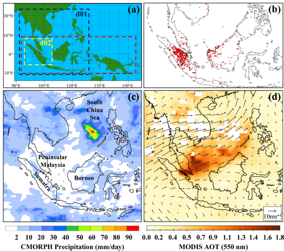
Figure 2. Overview of the aerosol and meteorological environment over the study region from 17 to 25 June 2013. (a) WRF-Chem model domain (dark blue) and nest d02 (yellow), and the Maritime Continent (MC) (red). (b) MODIS Terra and Aqua active fire hotspot detections (red dots). (c) Climate Prediction Center MORPHing technique product (CMORPH) average daily precipitation. (d) MODIS aerosol optical thickness (AOT) at 550 nm overlaid by average surface winds from the WRF-Chem simulations used in this study.
