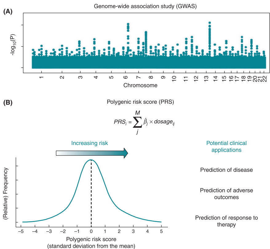
FIGURE 2 Genome-wide association studies (GWAS) test the association of common genetic variants with traits or diseases. Results are shown as a Manhattan plot (A) where the P -value (y-axis) is plotted against the genomic position (x-axis) for millions of common variants across the genome (blue markers). Polygenic risk scores (B) are generally derived from GWAS and calculated for an individual i ( PRS i ) as the sum of the products of allelic dosage ( dosage ij ) by the regression coefficient/weight ( β j ) for all M genetic variants ( j ). Created with Biorender.com
