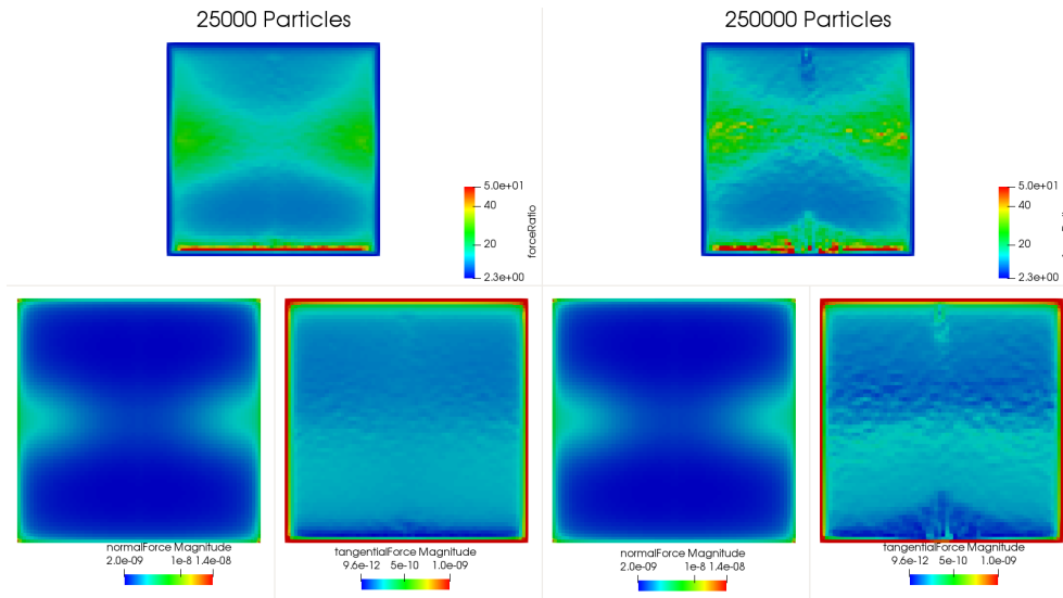
Figure 6: The top row shows force ratios on the plate substrate front surface in a) based on 25'000 computed particles and in b) based on 250'000 computed particles. The bottom row shows, the total normal (left) and tangential (right) force component magnitudes contributing to the respective force ratios.
