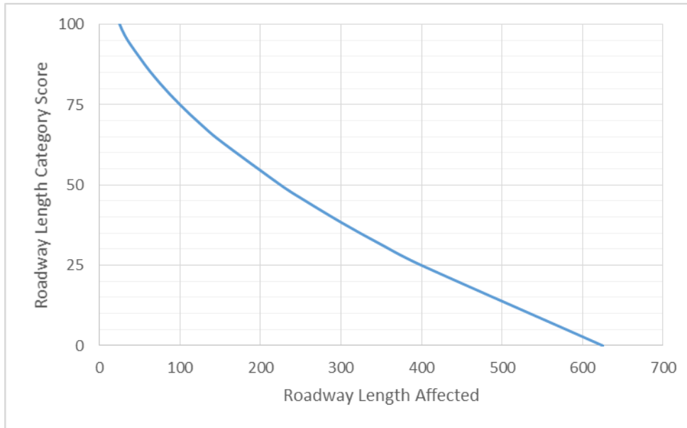
Figure 4-10: Chart illustrating the relationship between the length of roadway affected and the category score. The category score zeros out at an affected roadway length of about 625 feet.
