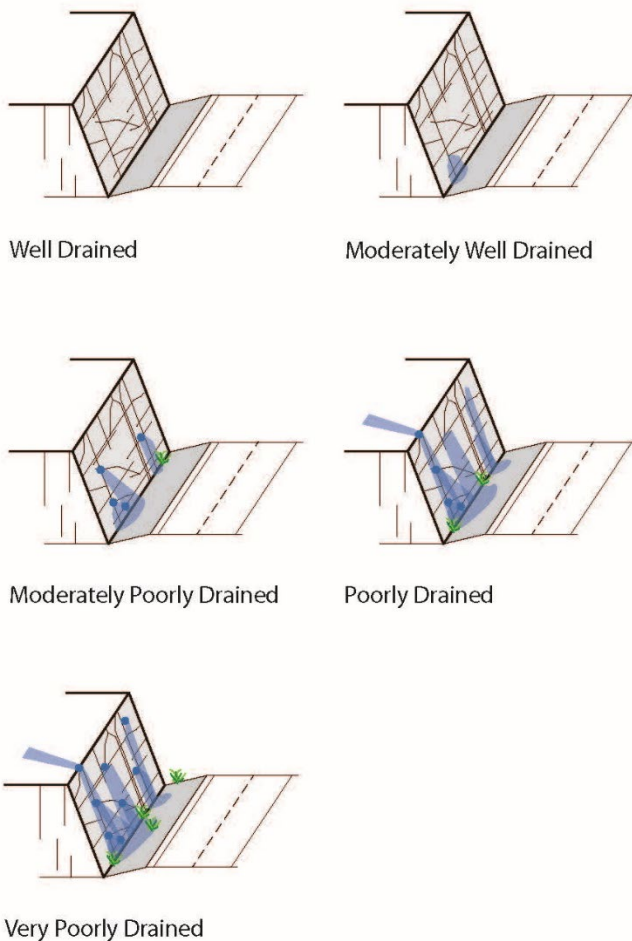
Figure 4-5: Schematic illustration of drainage categories using rock slope assets as an example.
