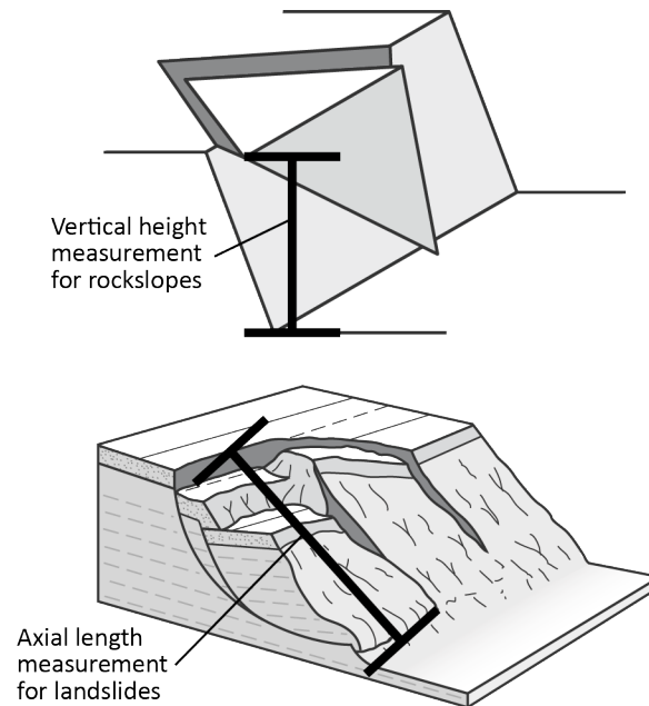
Figure 4-8: Examples of measuring vertical slope height on a rock slope and axial length on a landslide.
