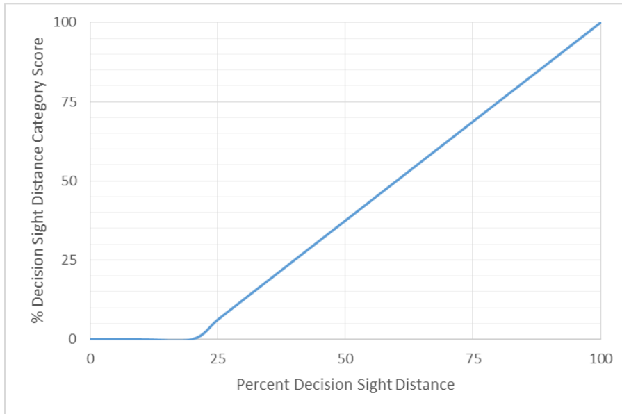
Figure 4-11: Chart illustrating the relationship between the percent decision sight distance and the category score. The category score maxes out at a percent decision sight distance of 100 % and is zero below a percent decision sight distance of 20%.
