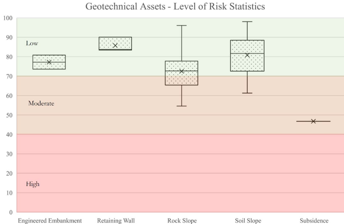
Figure 7-8: Bar and whisker plot summarizing the distribution of estimated level of risk for inventoried geotechnical assets. No subgrade assets were inventoried.
