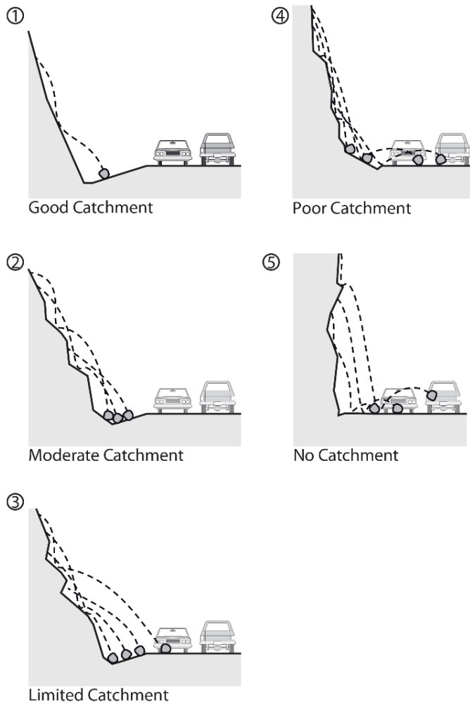
Figure 4-4: Ditch effectiveness explanatory diagram
