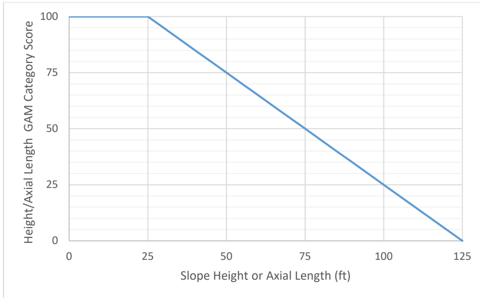
Figure 4-9: Chart illustrating the relationship between the slope height or axial length and the category score.
