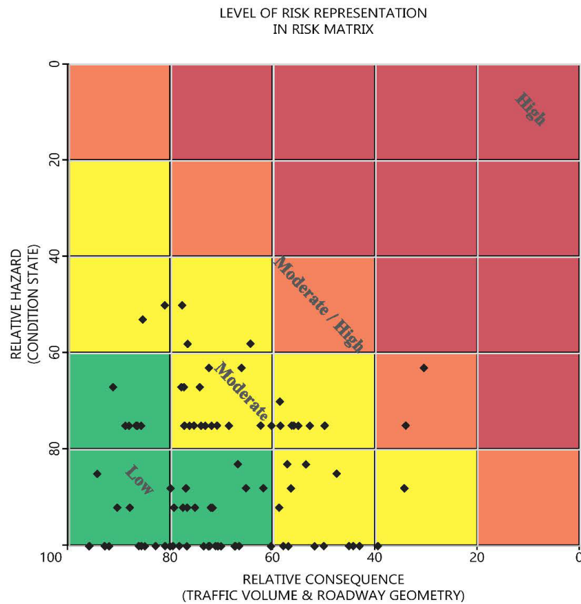
Figure ES-3: Level of Risk Matrix populated with Northwest and Northeast District geotechnical assets on NHS routes
