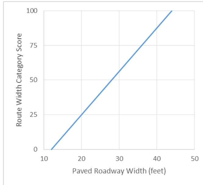
Figure 4-12: Chart illustrating the relationship between the paved roadway with and the category score.
