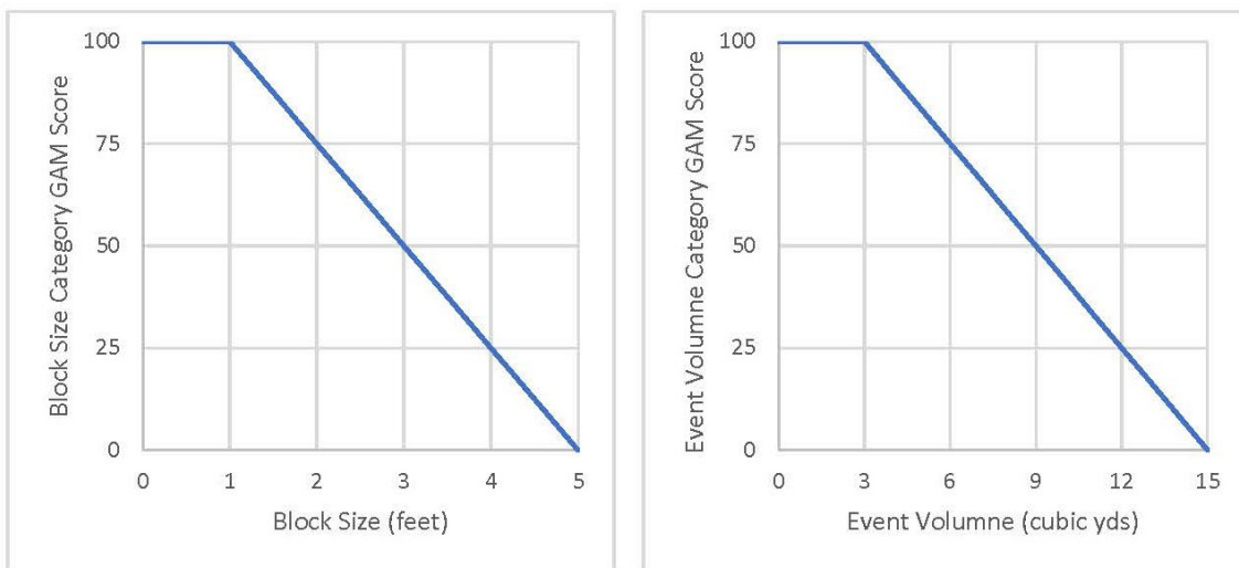
Figure 4-3: Chart pair illustrating the relationship between the block size and the category score and between the event volume and the category score.
