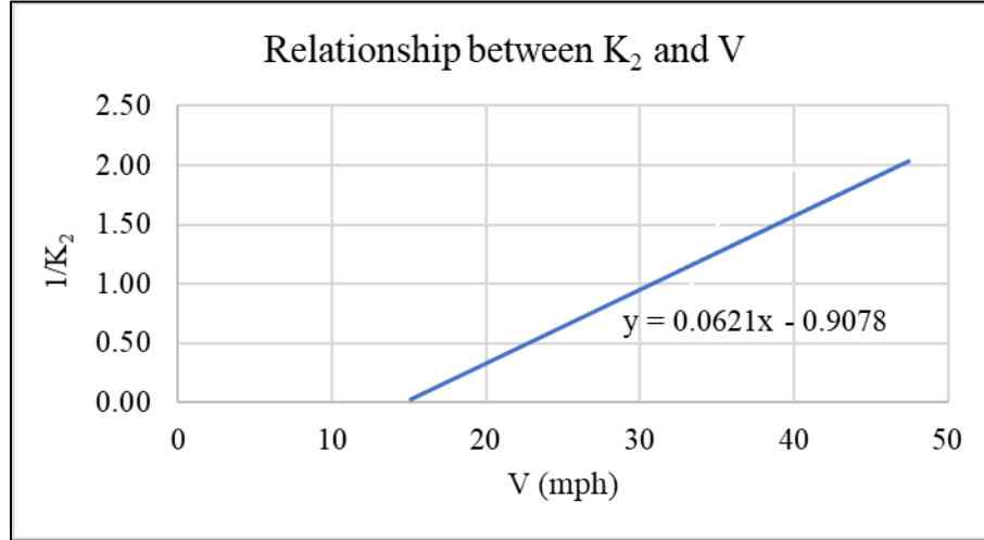
Figure 7. Variation of heat transfer parameter with speed.
