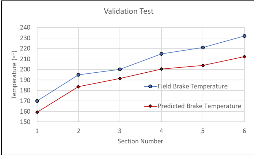
Figure 8. Comparison of field brake temperatures and predicted brake temperatures.
