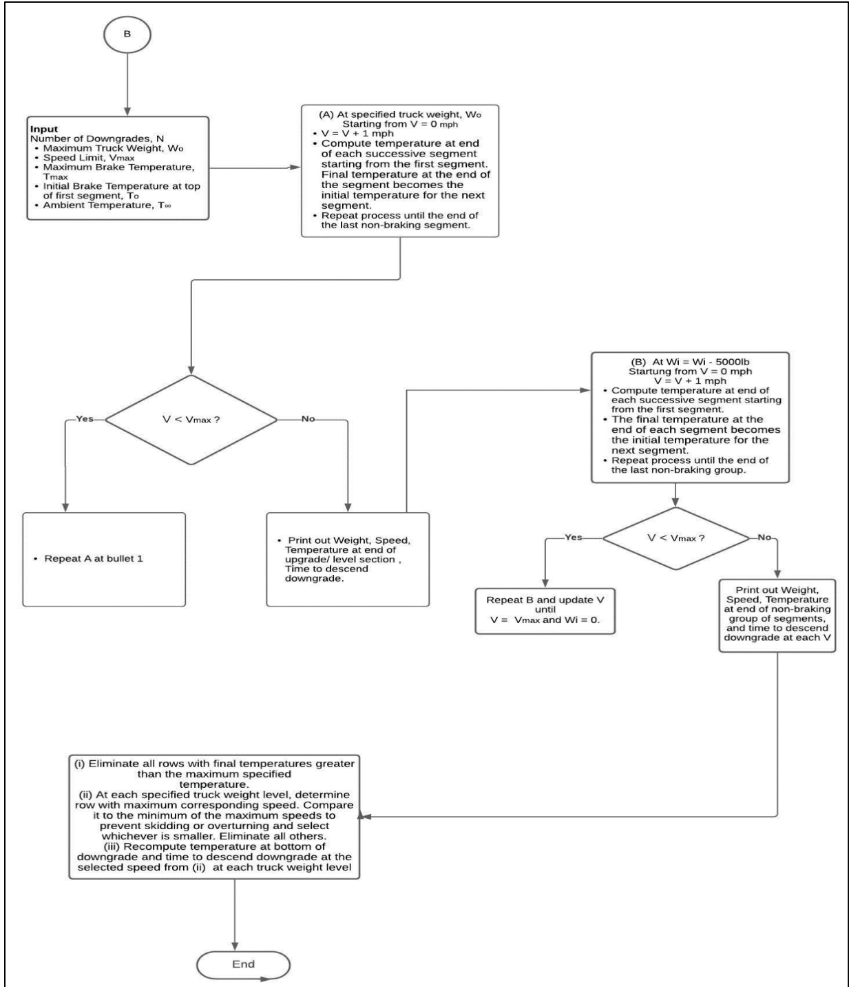
Figure 11. Process Flow Chart for Non-Braking Group of Segments for Separate Downgrade Method.
