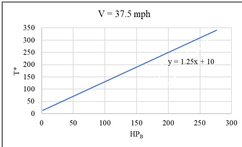
Figure 5. Temperature parameter versus power into brakes at 37.5 mph.
