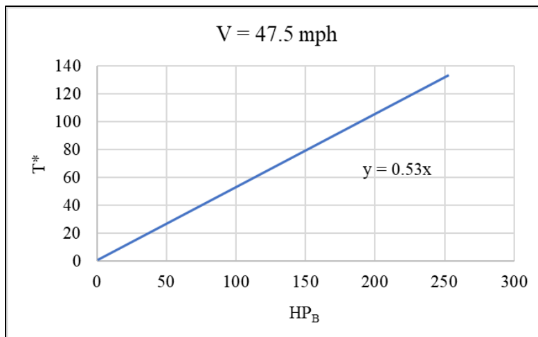
Figure 6. Temperature parameter versus power into brakes at 47.5 mph.
