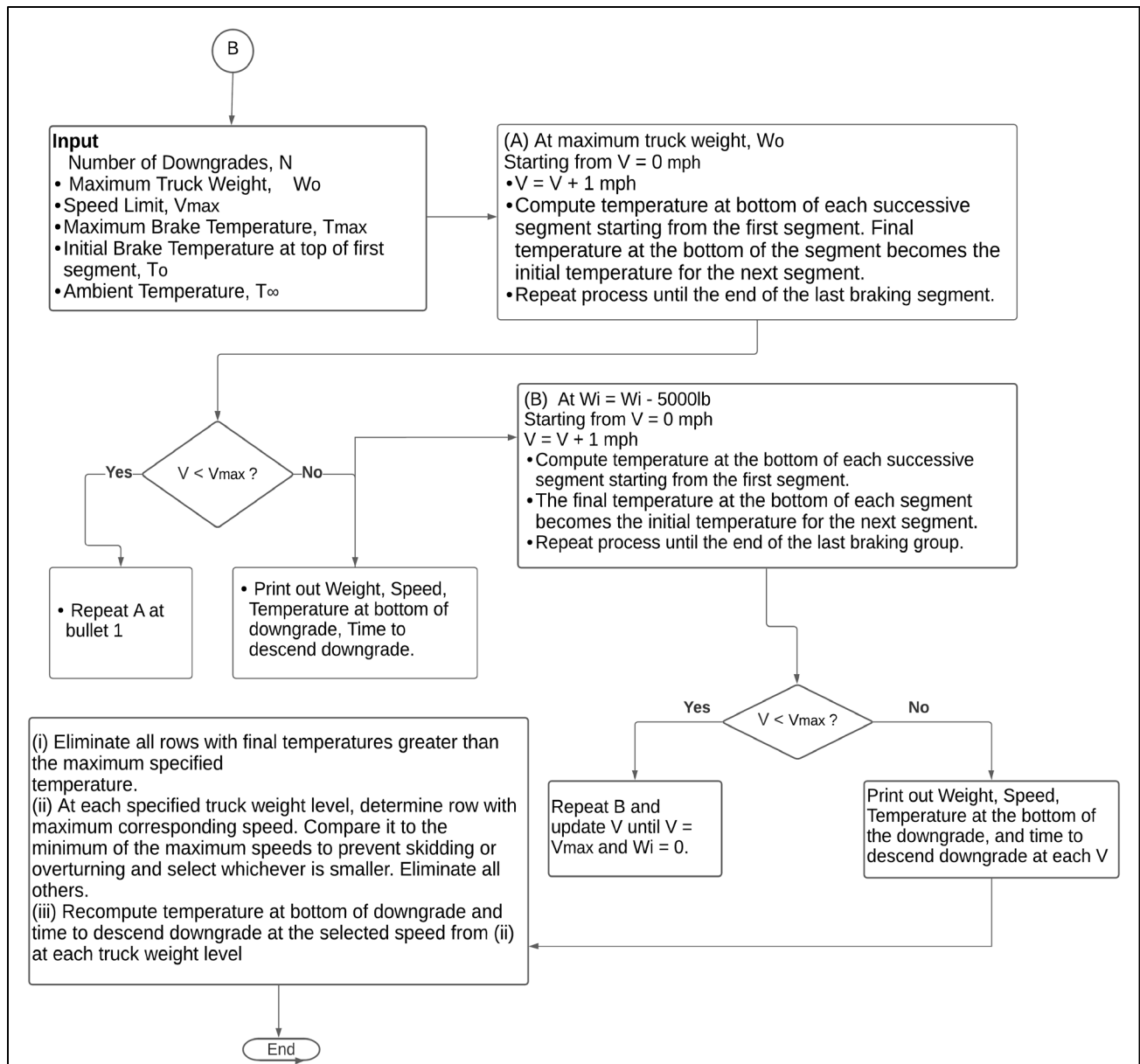
Figure 9. Process Flow Chart for Continuous Slope Method.
