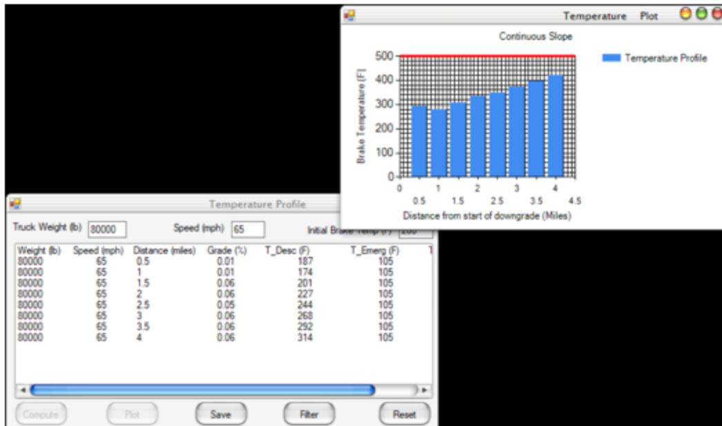
Figure A-8. An Example of Final Output and Temperature profile of Maximum Descent Speeds based on the Continuous Slope Method.
