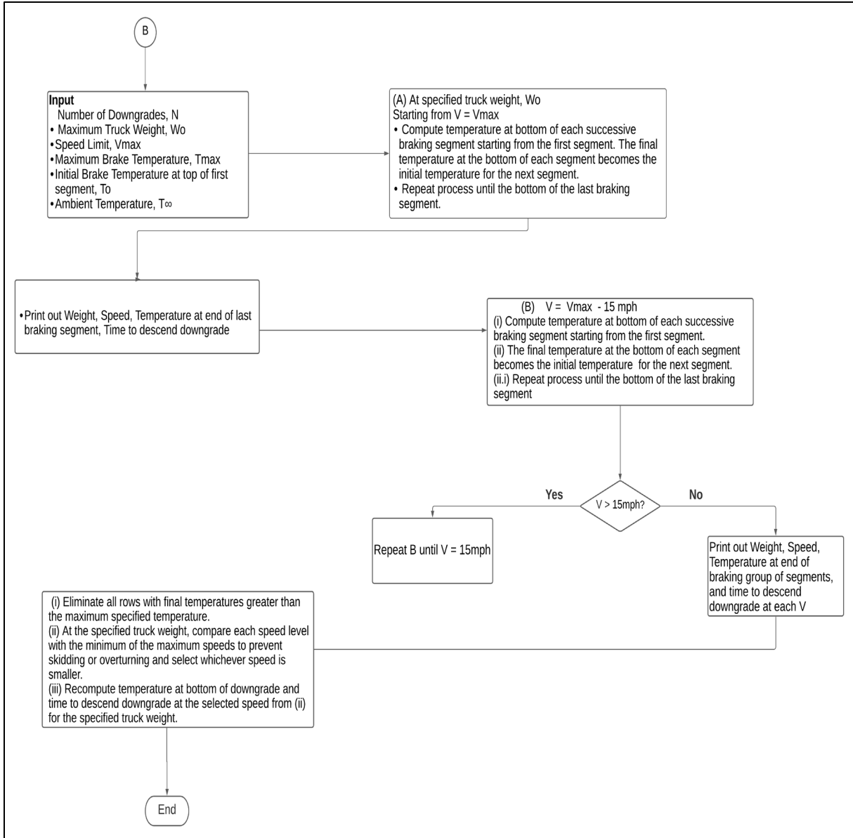
Figure 10. Process Flow Chart for Braking Group of Segments for Separate Downgrade Method.
