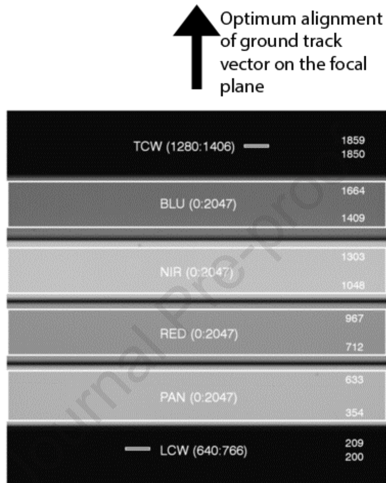
Figure 1 - CaSSIS filter setup on top of the 2048 x 2048 CMOS sensor [5]: This filter mask combined with the push-frame image acquisition setup – allows for up to four colour CaSSIS images. The numbers in between parenthesis are the horizontal pixel coordinates starting on the left, and the numbers on the right are the limits on vertical pixel coordinates for each filter. Areas outside the boxes are
