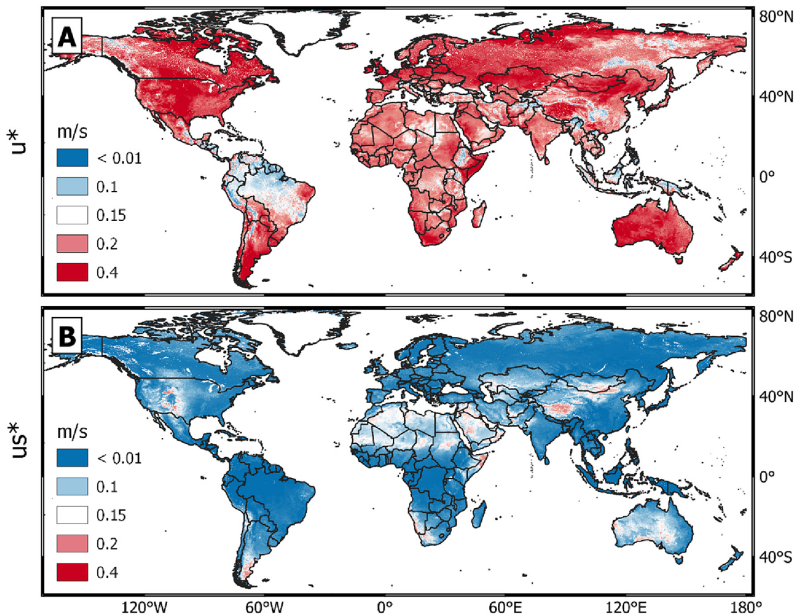
Fig. 3. For the year 2020 the albedo-based wind friction velocity ( u_* ; A) is shown for comparison with the albedo-based soil surface wind friction velocity ( u_{s*} ; B) used in the albedo-based dust emission model (AEM). The AEM relates u_{s*} directly to normalised shadow (1-albedo) and uses MODIS albedo to enable spatio-temporal variation (every 500 m pixel, daily) with changing aerodynamic roughness and wind speed. Daily albedo data were obtained from the MODIS satellites (Schaaf and Wang, 2015).
