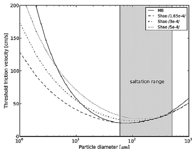
Fig. A1. Threshold friction velocity over a smooth surface calculated with Marticorena and Bergametti (1995; MB) and Shao and Lu (2000) dust emission schemes (taken from Darnenova et al., 2009).
