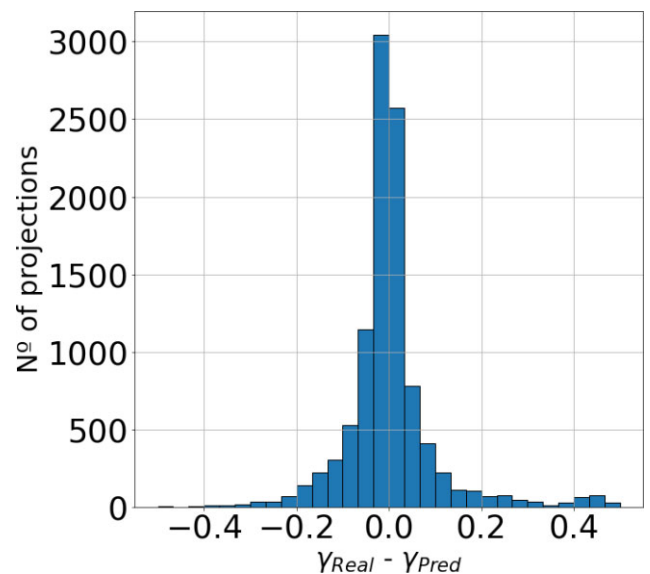
Figure 6. Distribution of \gamma_{\text{Real}} - \gamma_{\text{Pred, mode}} for every projection of each galaxy in our training set.
