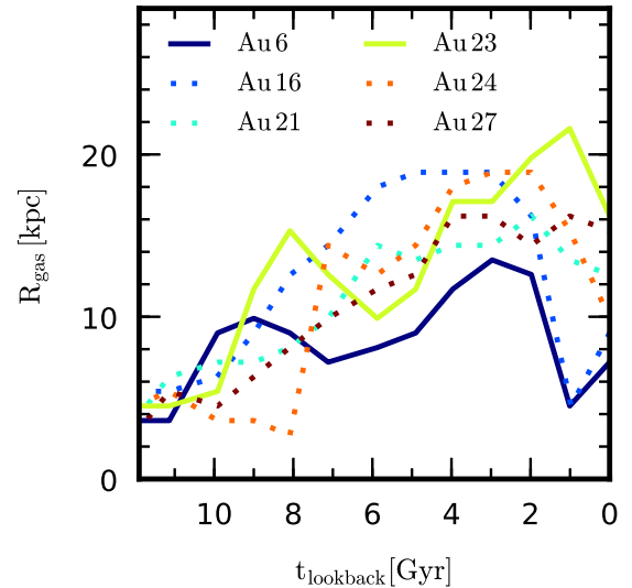
Figure 3. The evolution of the ‘edge’ of the gas disc, defined to be the radius at which the gas surface density falls below 5 M_{\odot} \text{pc}^{-2} , for all simulations. Each curve is coloured according to the label in Fig. 2.
