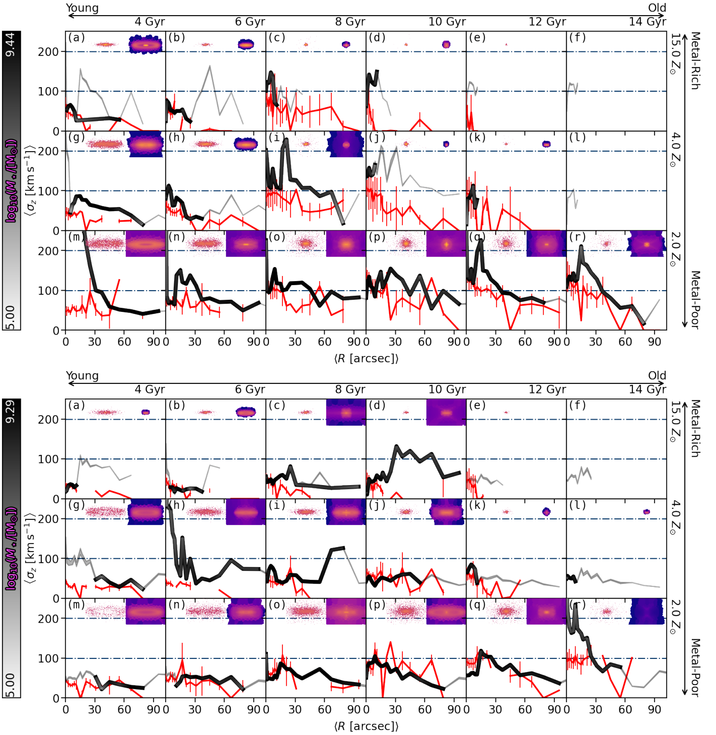
Fig. C.3. Similar to Fig. 10, showing the assembly history for halo 5 (top) and halo 6 (bottom). In addition to the \sigma_z radial profile (black/white line) and surface brightness distribution (upper right) from the Schwarzschild model, the shaded regions correspond to the variations derived from 100 Monte Carlo fits to the stellar population maps. Each panel also contains the intrinsic \sigma_z radial profile (red line) and surface brightness distribution (upper left) from the simulations.
