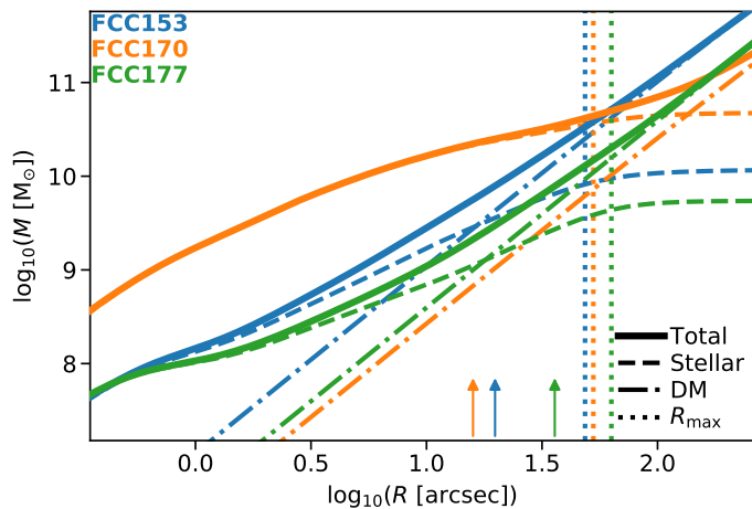
Fig. 3. Enclosed-mass profiles of the total (dynamical) mass ( solid line ), stellar mass ( dashed line ), and DM ( dot-dashed line ) for the three galaxies. The effective radii are denoted by the small arrows, and the radial extent of each spectroscopic FOV is shown by the vertical dotted line. The lower radial bound of the figure is set to half the width of the point-spread function from the spectroscopic observations.
