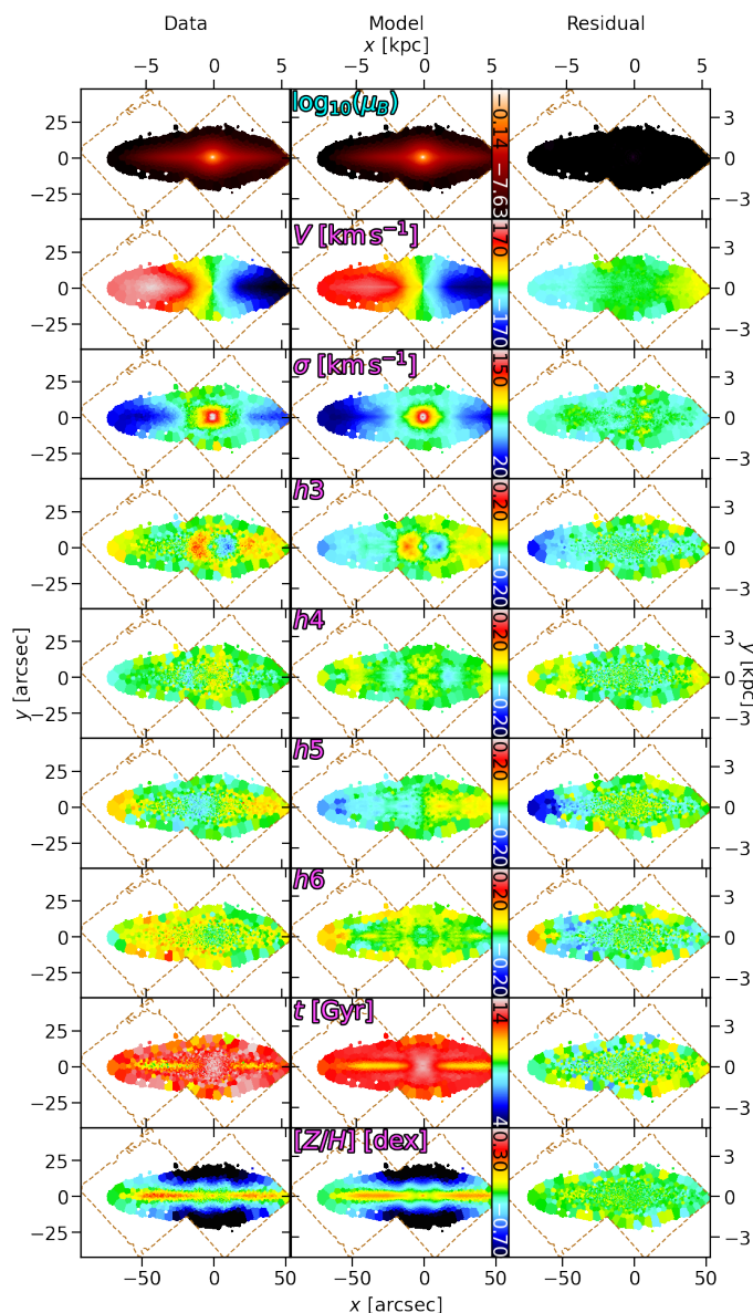
Fig. 8. Same as Fig. 7, but for FCC 170.
