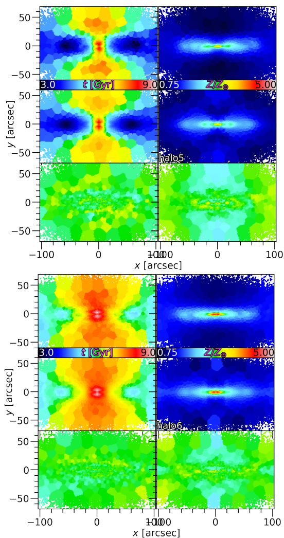
Fig. C.1. Stellar-population Schwarzschild model fits to the mock data. Mean stellar age ( left ) and metallicity ( right ) are shown for Auriga halos 5 ( top ) and 6 ( bottom ). From top to bottom, the rows represent the true means, models fits, and residuals.
