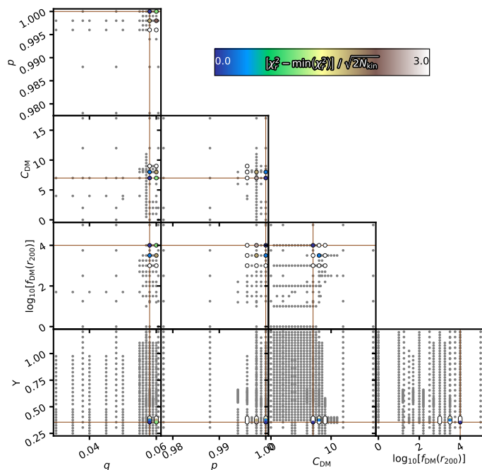
Fig. B.1. Optimisation over the 5D parameter-space for FCC 153. The grey points indicate the exploration of the parameter-space with the smaller orbit sampling, while the coloured points show the \chi^2 of the models with the high orbit sampling (see § 3.2). The best-fit parameters are indicated by the brown lines.
