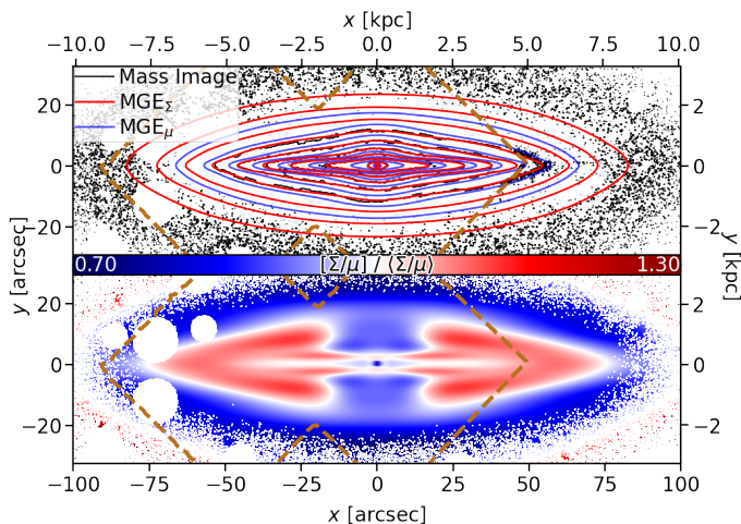
Fig. A.1. the mass-density MGE for FCC 153. Top : Contours of the projected mass density (black), the mass density MGE_z (red), and the surface brightness MGE_\mu (blue). Bottom : The ratio between the mass and surface-brightness models, showing the structural differences. This panel is normalised by the average M_*/L such that values of 1.0 (white) are consistent with the assumption of a spatially-constant M_*/L , and any deviations are percentages in stellar mass. The outline of the MUSE mosaic is shown in dashed brown.
