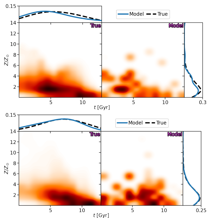
Fig. C.2. Intrinsic t - Z distribution ( left ) and that retrieved from our model ( right ) for halos 5 ( top ) and 6 ( bottom ). The 1D distributions are also shown for each simulation, as kernel density estimates of the underlying data. The intrinsic distributions are black dashed curves, and the model distributions are the blue solid curves.
