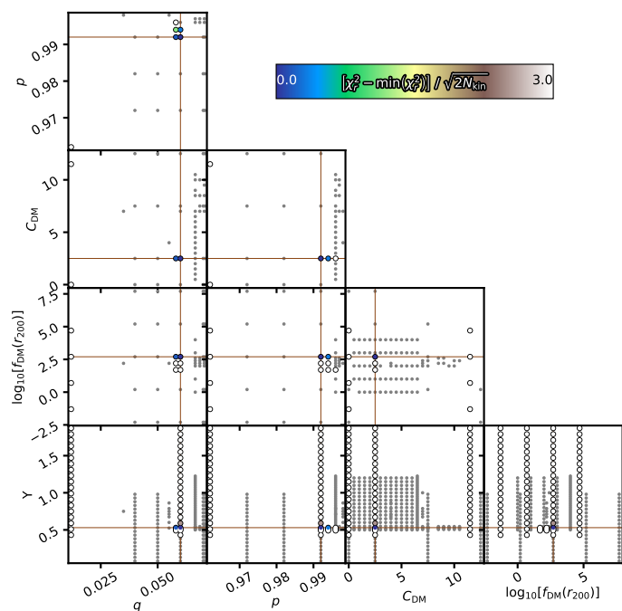
Fig. B.2. Same as Fig. B.1, but for FCC 170.
